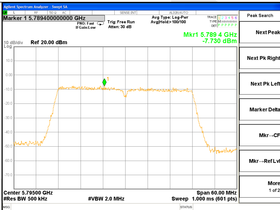
ANT 1---Test Mode: 802.11n(HT40)---5795
