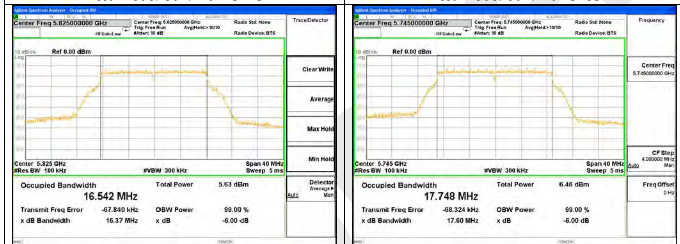
ANT 0---6dB Bandwidth Test Mode: 802.11a--5825
