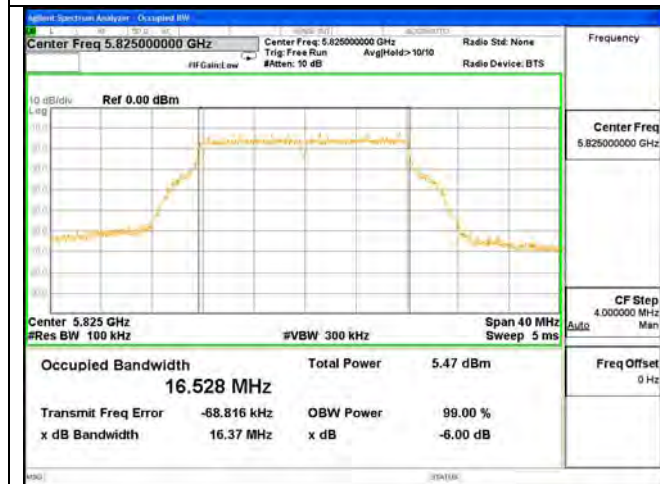
ANT 1---6dB Bandwidth Test Mode: 802.11a---5825
