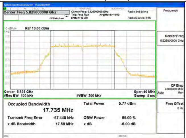
ANT 1---6dB Bandwidth Test Mode: 802.11n(HT20)---5825
