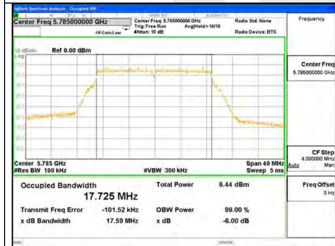
ANT 1---6dB Bandwidth Test Mode: 802.11n(HT20)---5785
