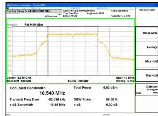
ANT 1---6dB Bandwidth Test Mode: 802.11a---5745
