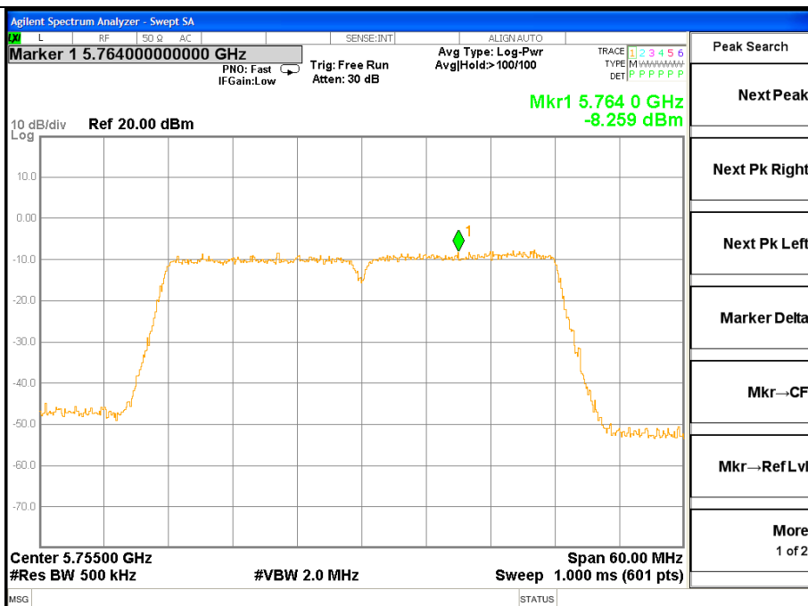
ANT 1---Test Mode: 802.11n(HT40)---5755
