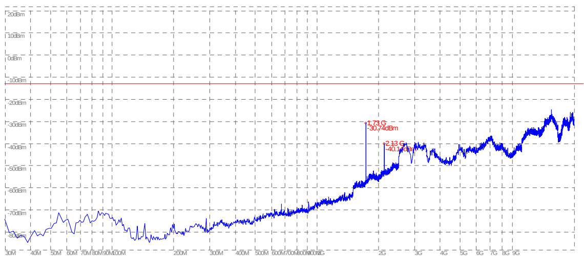
(Plot H.1: AWS 1700MHz Channel = 450, Test Antenna Horizontal)
