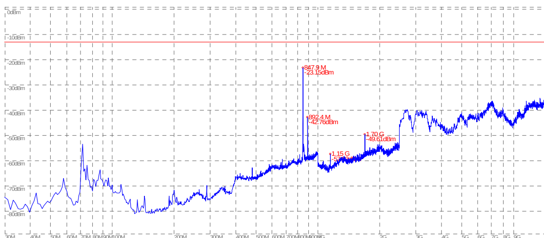
(Plot C.2: CDMA 800MHz Channel = 777, Test Antenna Vertical)
