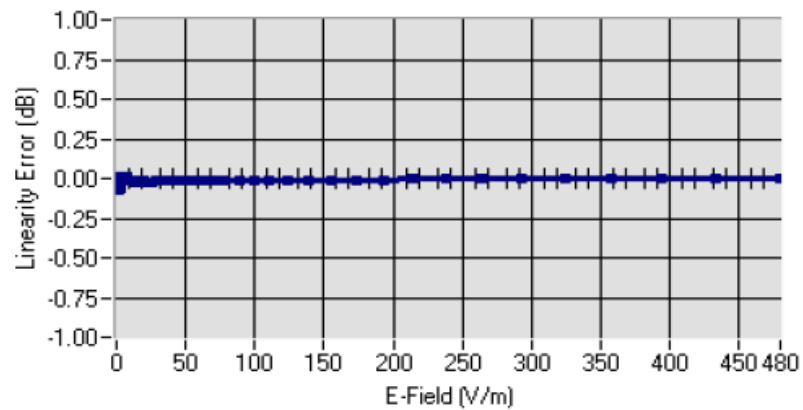
Linearity
