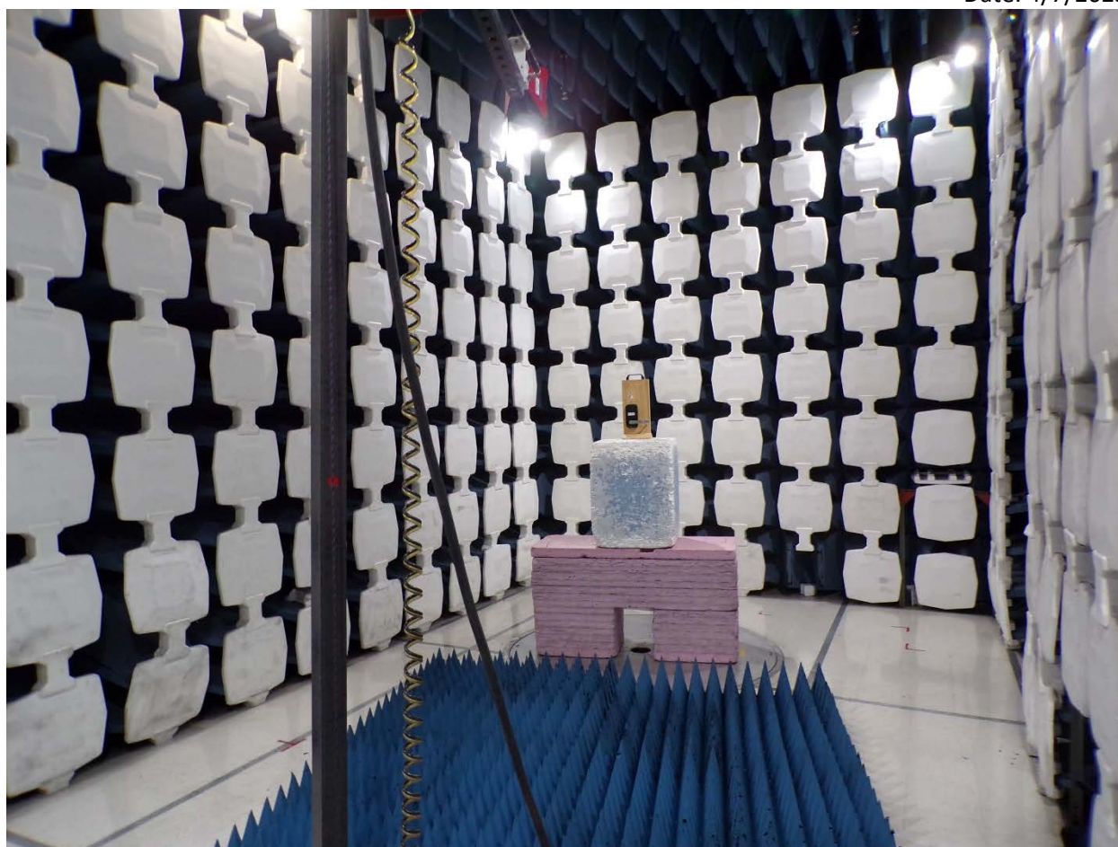
1-6GHz
