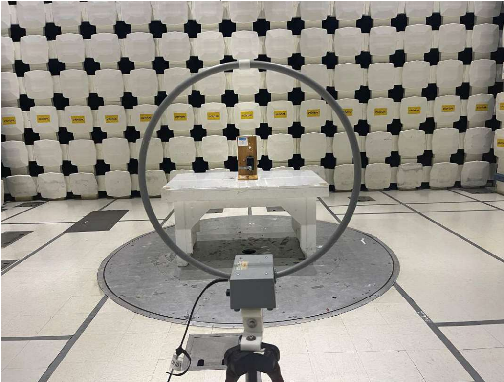
Test Setup From 9 kHz-30 MHz
