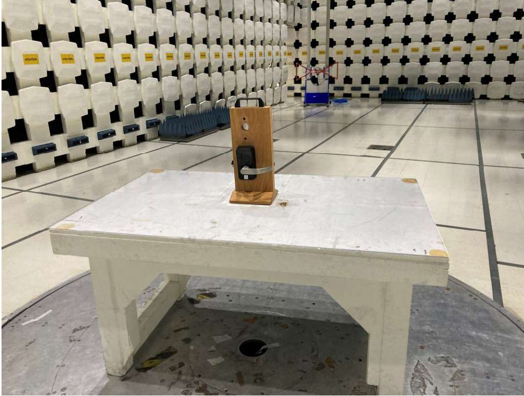
Test Setup From 30-1000 MHz
