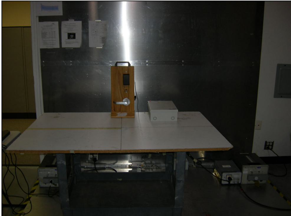
Figure 4: Conducted Emissions
