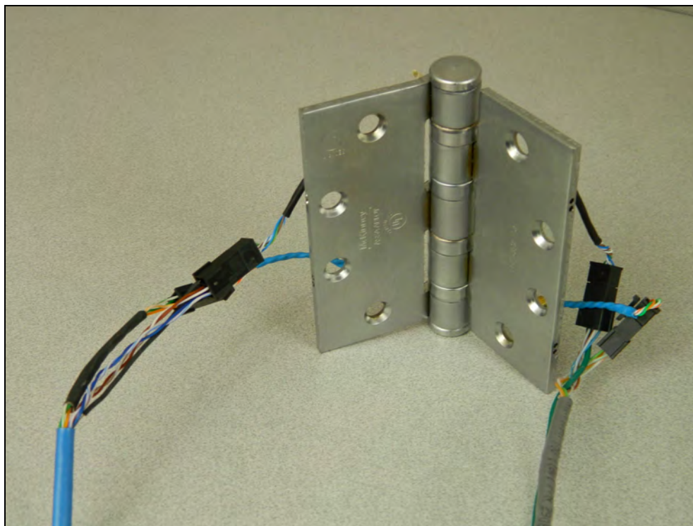
Figure 13: External Photo – Host – Passport 1000 P1 BIKMPS\C 10 Line PoE (Hinge)
