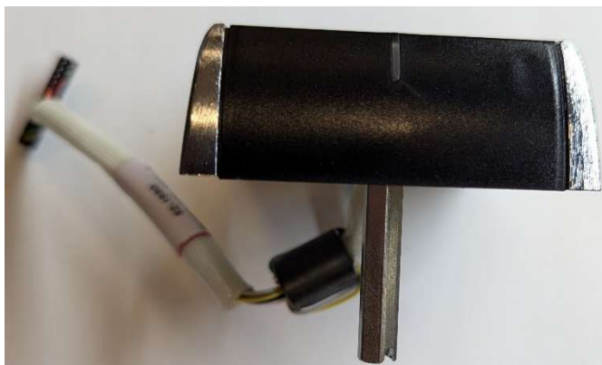
Figure 14 IN120/IN220 KEYPAD METAL WINGS TOP
