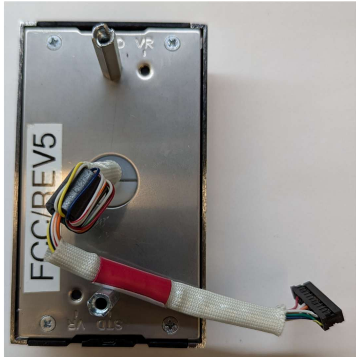
Figure 12 IN120/IN220 KEYPAD METAL WINGS REAR
