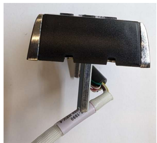
Figure 11 IN120/IN220 KEYPAD METAL WINGS BOTTOM
