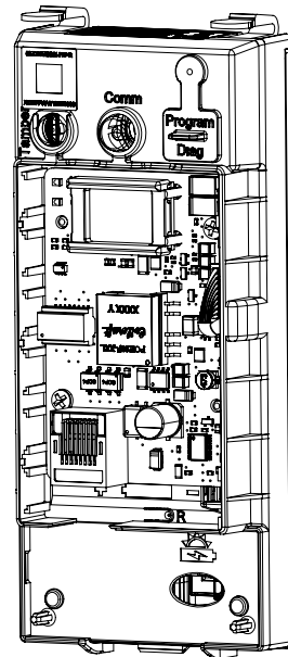
Front of controller (PoE shown)
