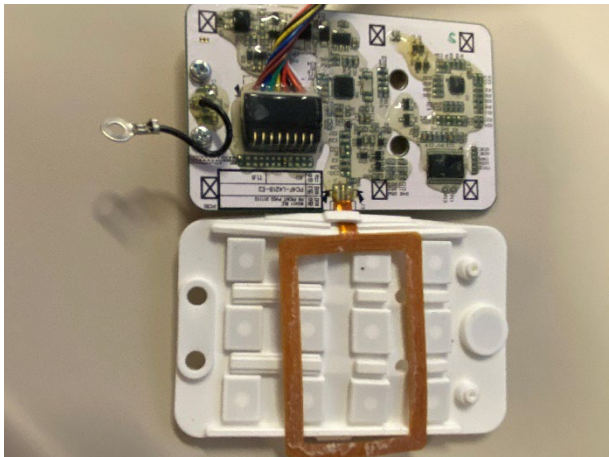
Push Button PCB Back
