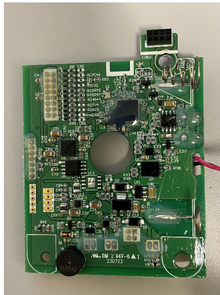
PCB Front with Battery Holder Removed
