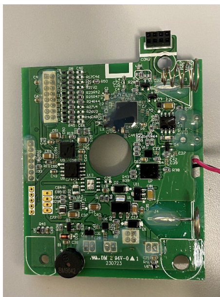
PCB Front with Battery Holder Removed
