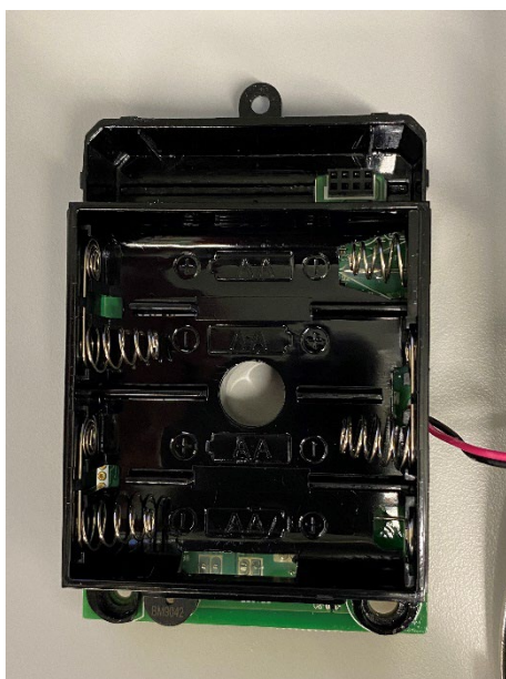
PCB Front
