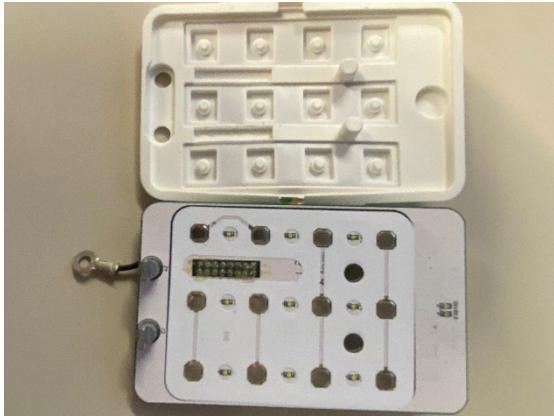
Push Button PCB Front
