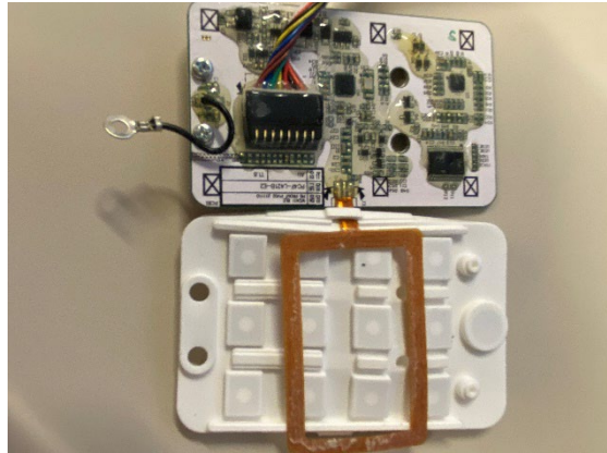
Push Button PCB Back
