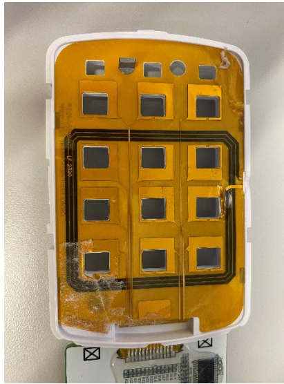
RFID Antenna Behind Touchscreen
