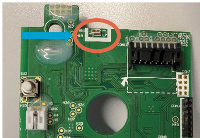
PCB Back- BLE Antenna Location
