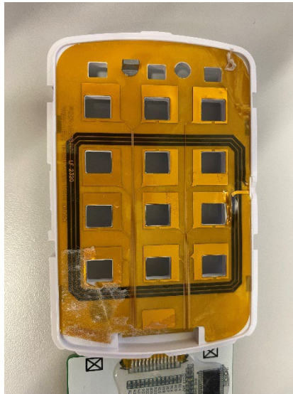
RFID Antenna Behind Touchscreen
