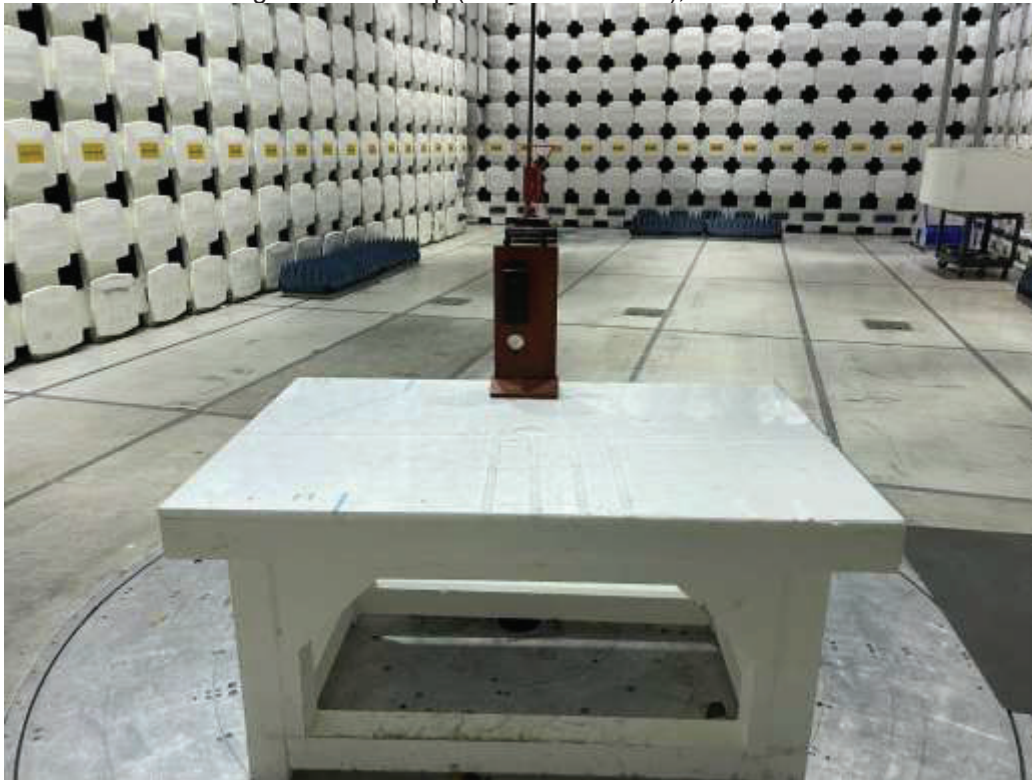
BLE &amp; Zigbee Test Setup (Plastic Enclosure), RE 30-1000 MHz
