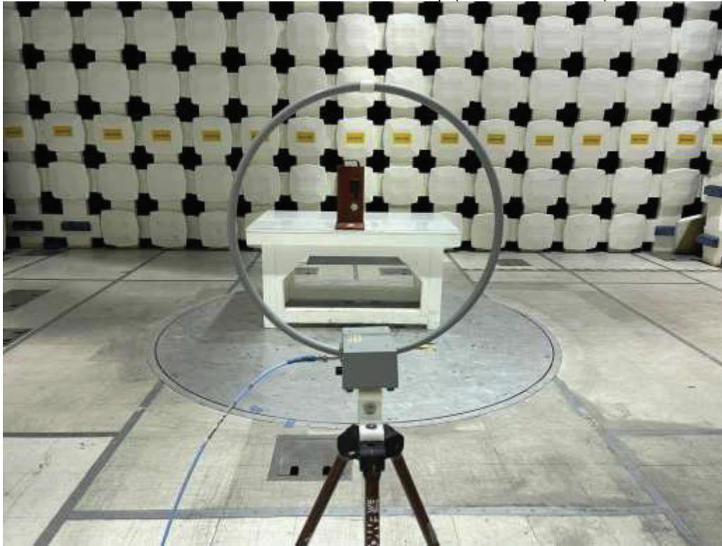
125 kHz &amp; 13.56 MHz RFID Test Setup (Plastic Enclosure)
