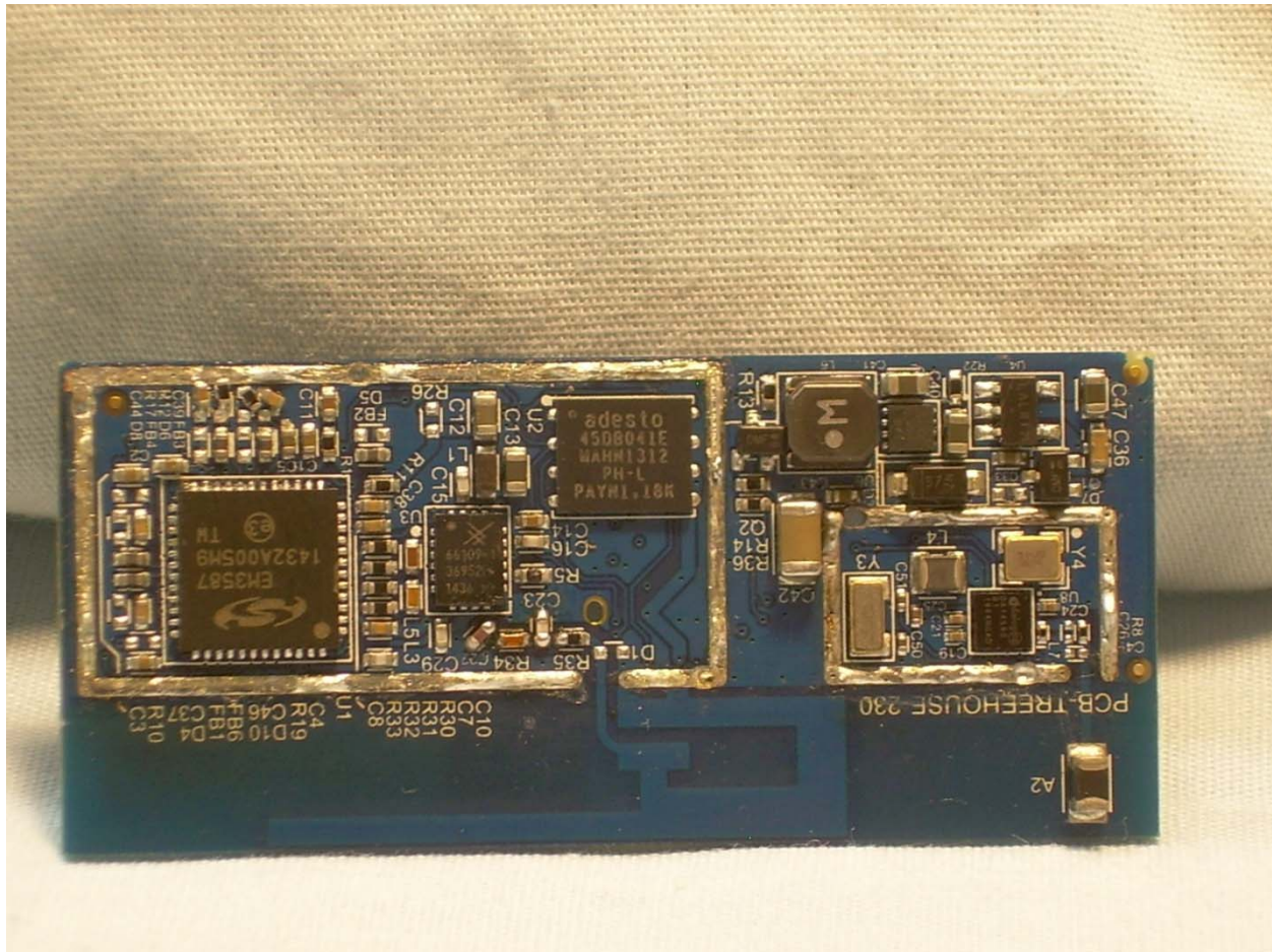
Photograph 7 – View of the PCB with RF Shielding Removed
