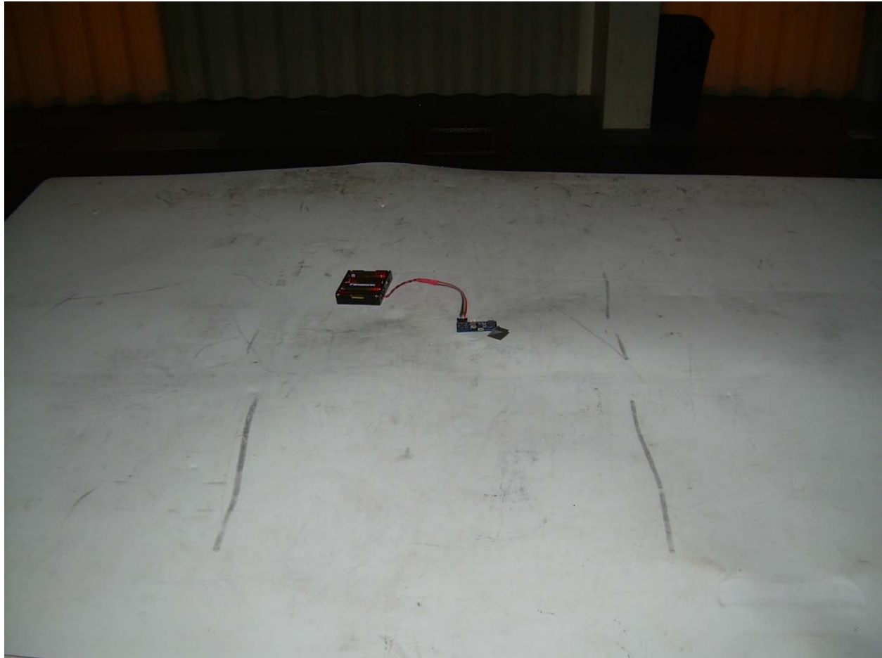
Photograph 1 – Front View of the Radiated Emission Setup – EUT Flat on Table
