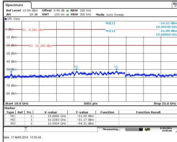
Figure 7.5.1.2-6: 10 GHz – 25 GHz – 2440 MHz
