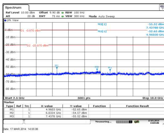
Figure 7.5.1.2-8: 2.5 GHz – 10 GHz – 2480 MHz
