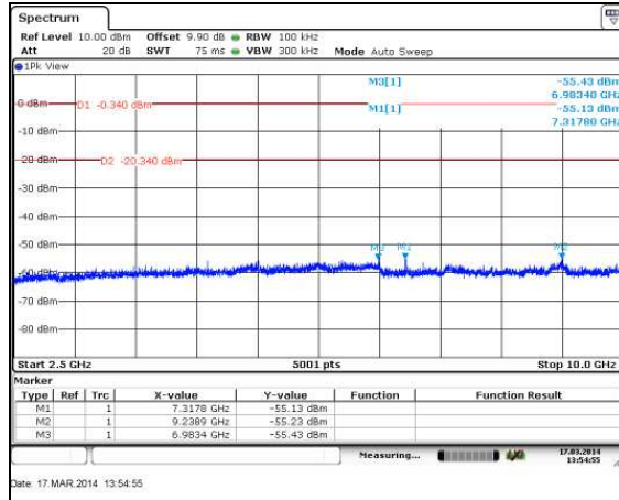
Figure 7.5.1.2-5: 2.5 GHz – 10 GHz – 2440 MHz
