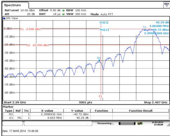
Figure 7.5.1.2-10: Lower Band-edge - 2405 MHz
