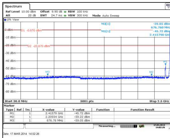
Figure 7.5.1.2-7: 30 MHz – 2.5 GHz – 2480 MHz
