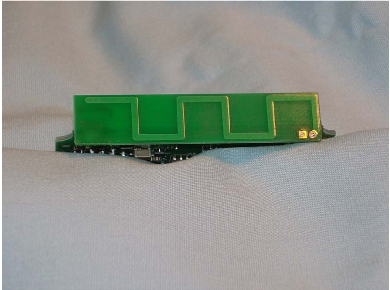
View of the Antenna PCB
