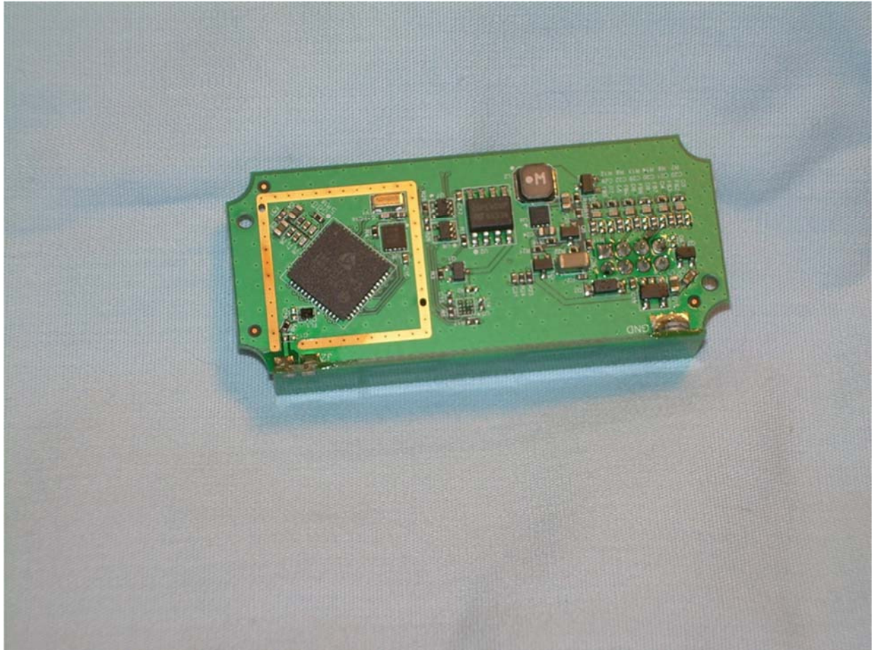
View of the Top Side of the PCB with RF Shielding Removed
