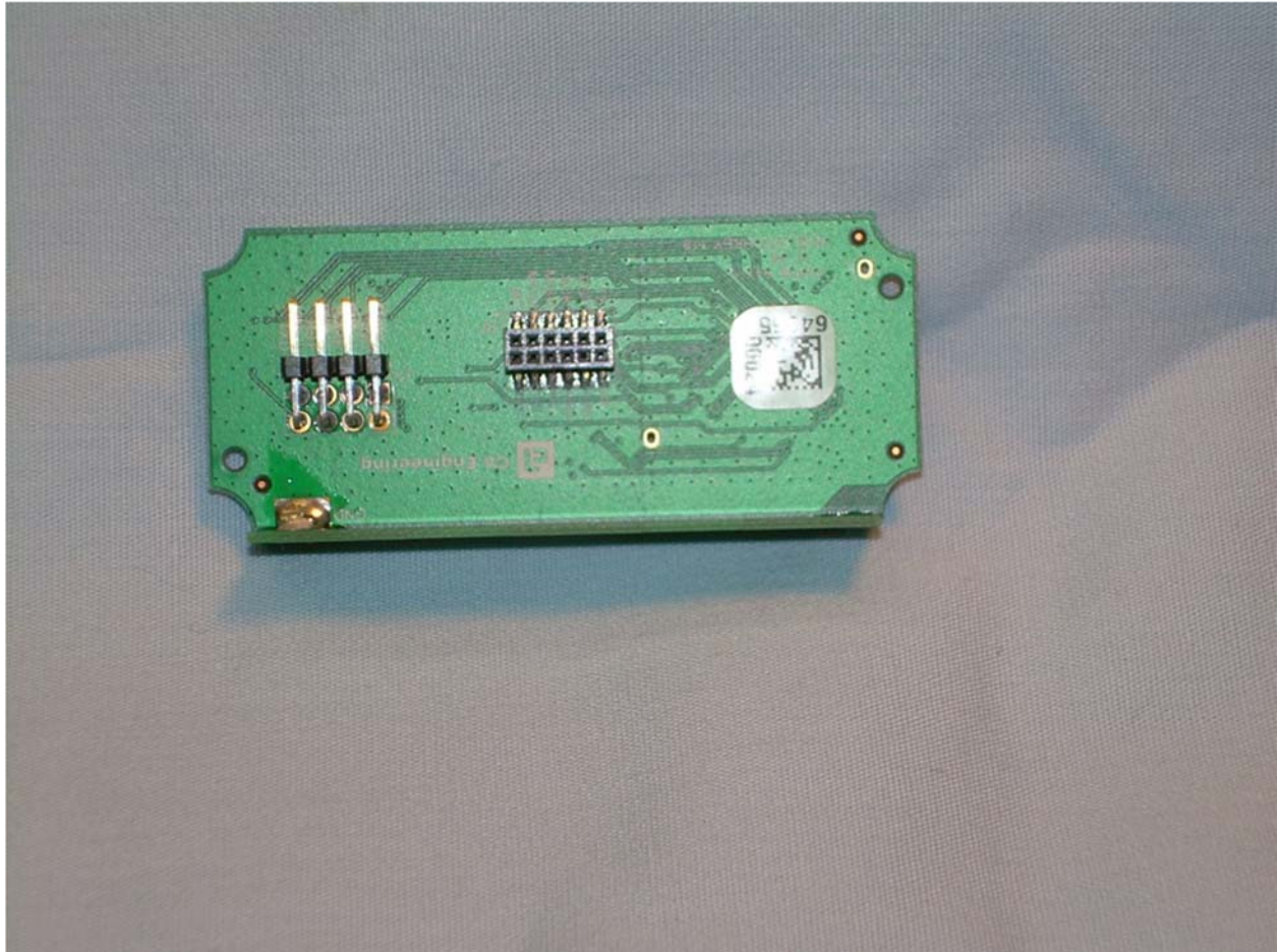
View of the Bottom of the EUT PCB
