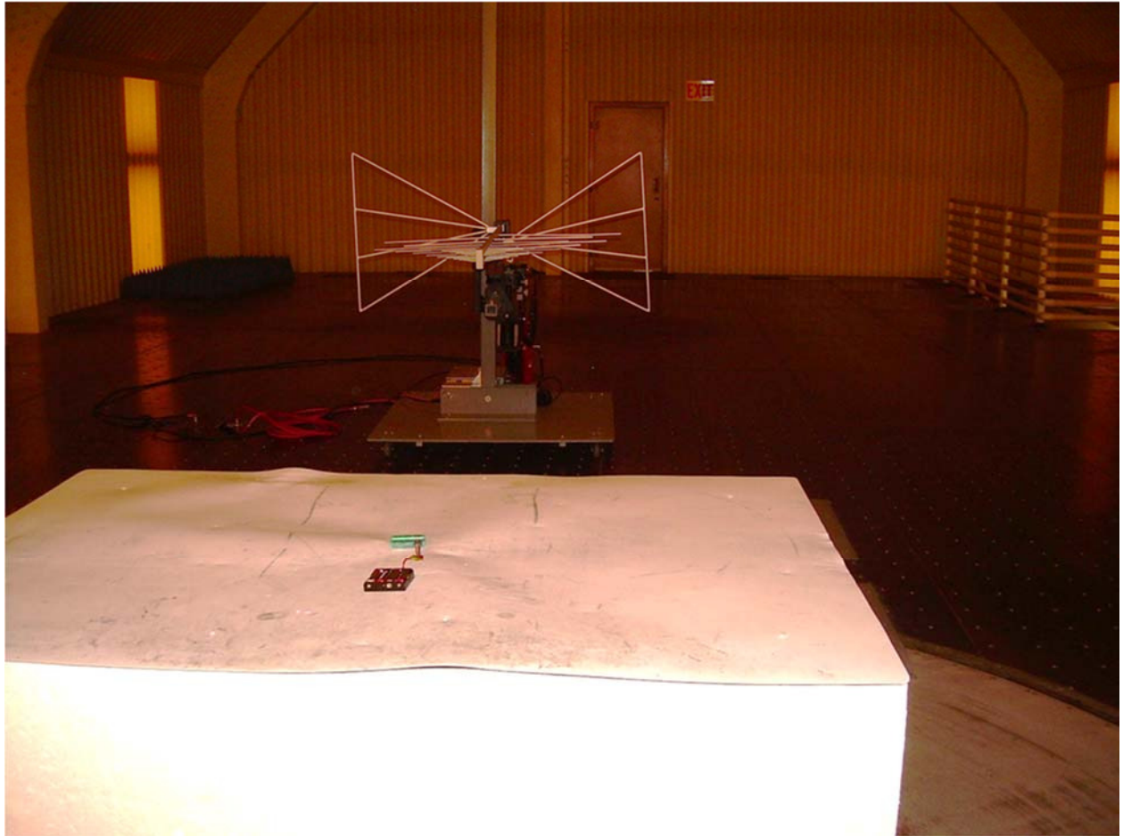
Back View Radiated Disturbance Flat Configuration
