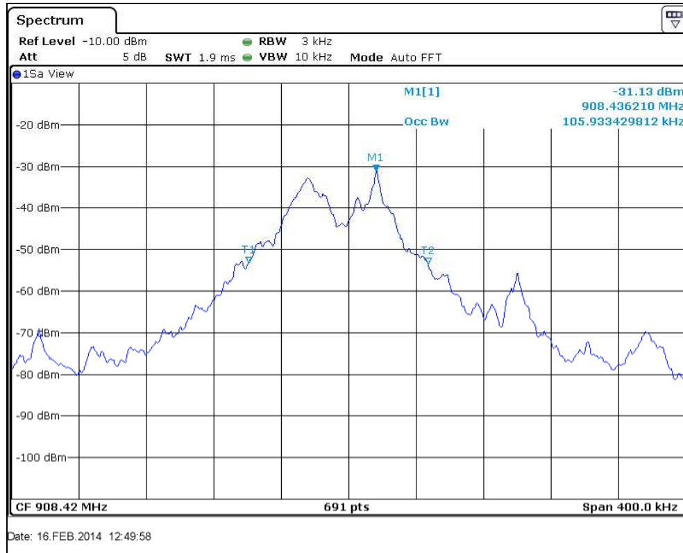
Figure 7.3.2-2: 99% OBW
