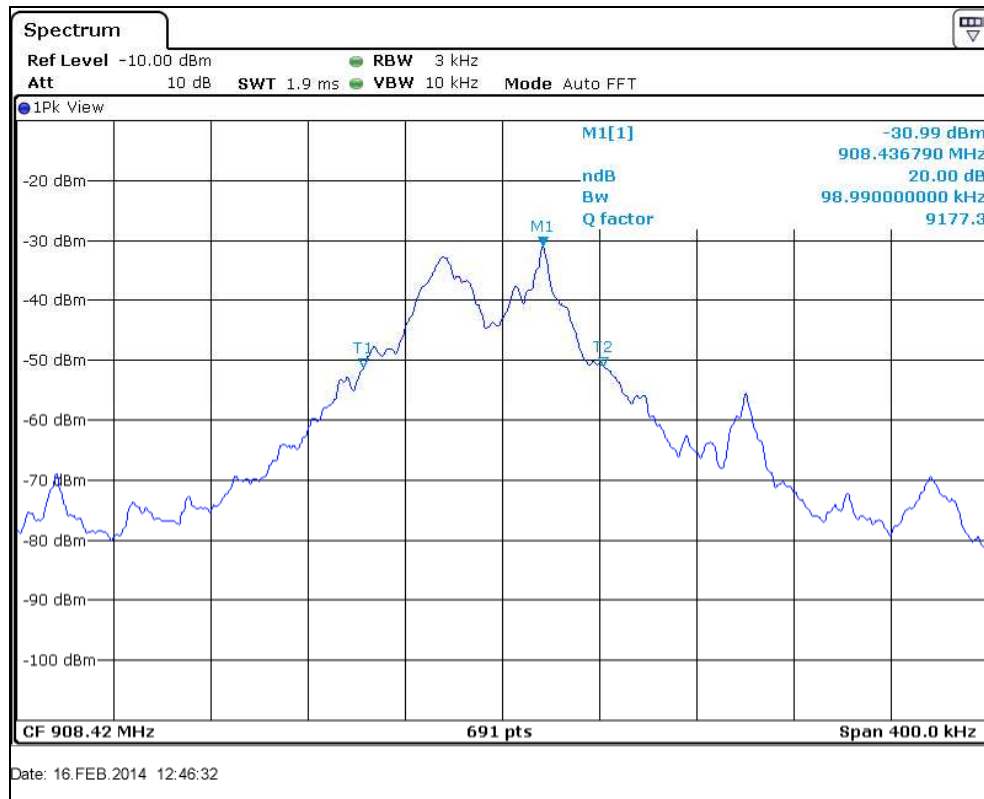
Figure 7.3.2-1: 20dB BW
