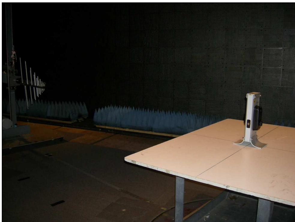
Figure 2: Radiated Emissions – Push Button Deadbolt Lock
