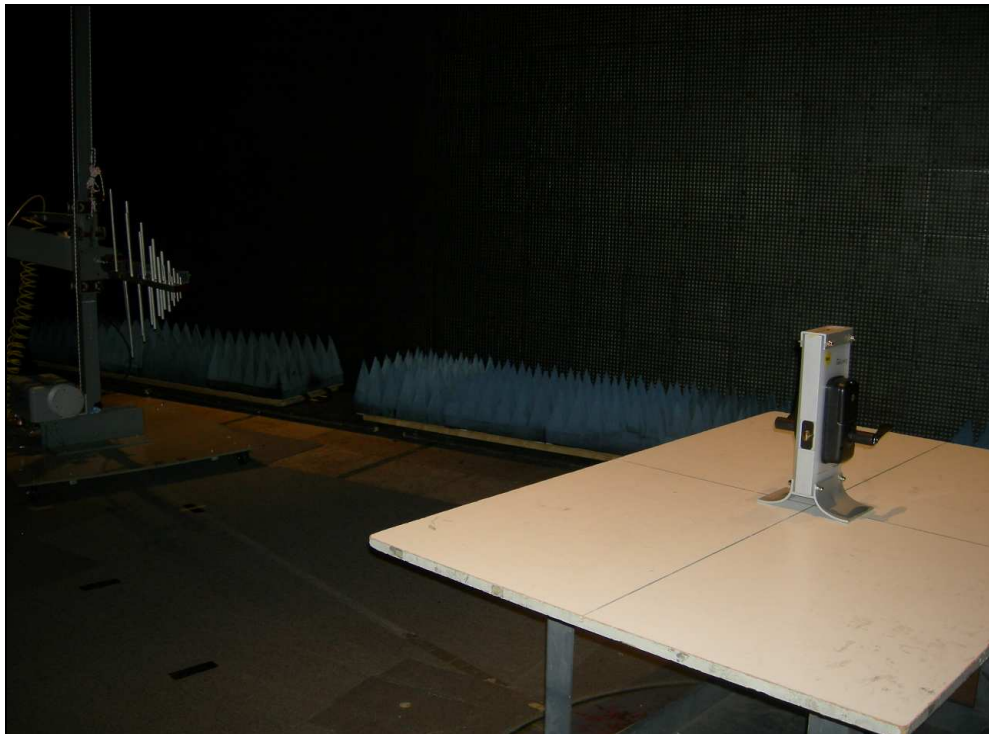
Figure 10: Radiated Emissions – Touch Screen Lever Lock
