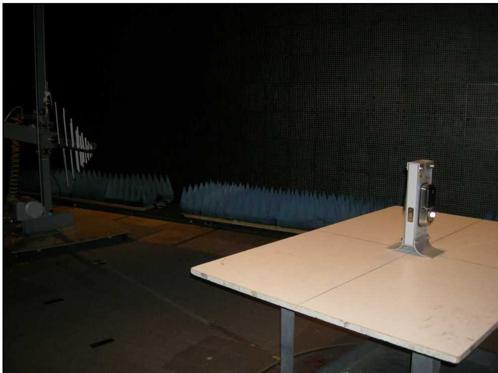
Figure 4: Radiated Emissions – Touch Screen Deadbolt Lock
