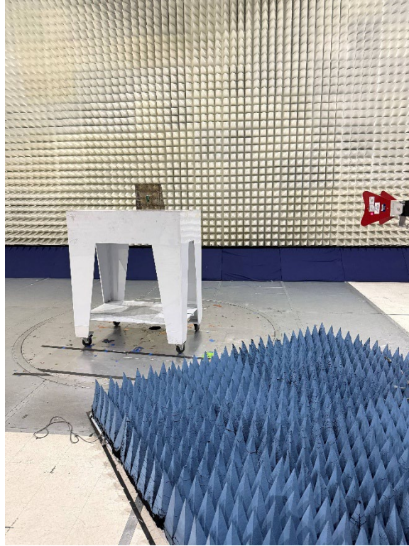
Radiated Emission, 1GHz – 4GHz
