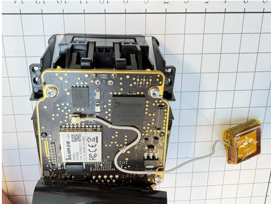
RFID module and antenna
