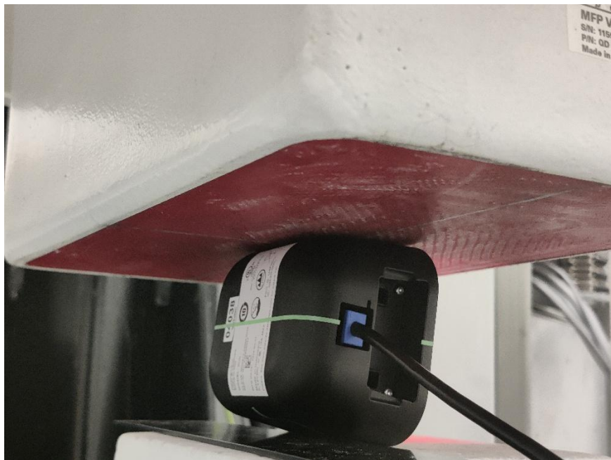
Figure 6 Left 0mm separation distance
