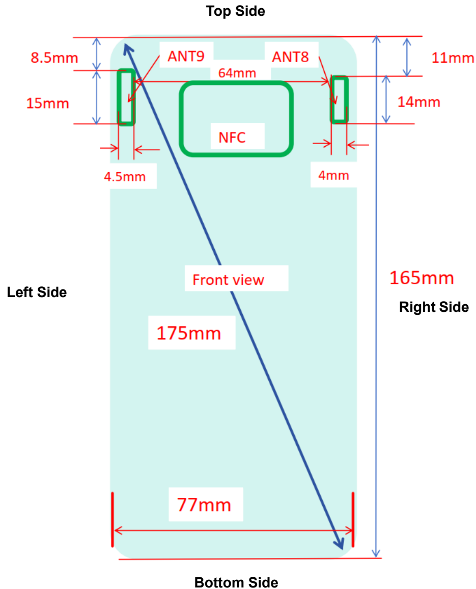
Picture 11.1 Antenna Locations (Front View)
