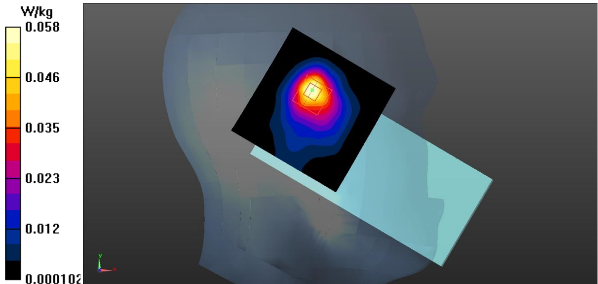
Fig.1 Bluetooth Head
