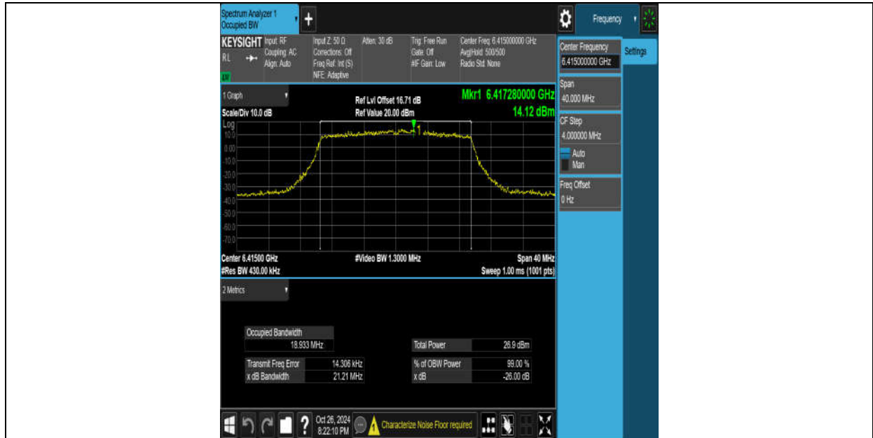
11AX20MIMO-Ant8-6415-PASS
