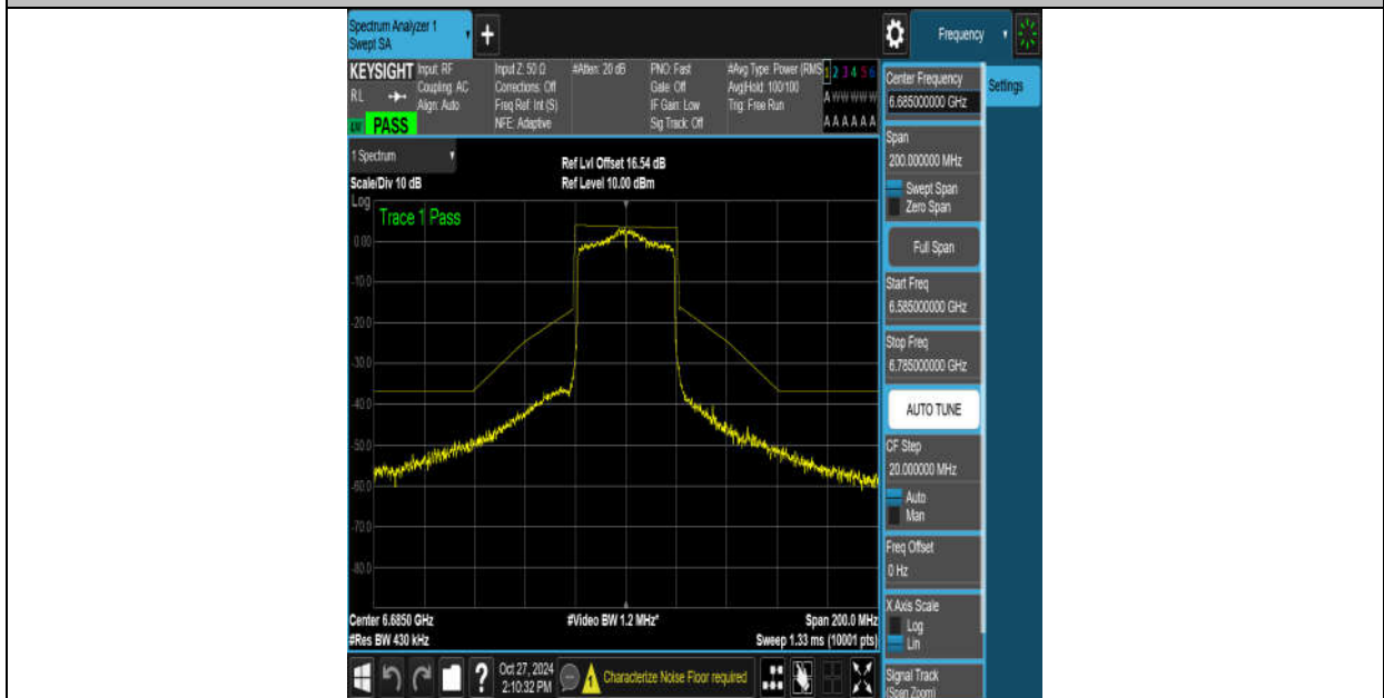
NTNV-11AX40MIMO-Ant8-6685-PASS
