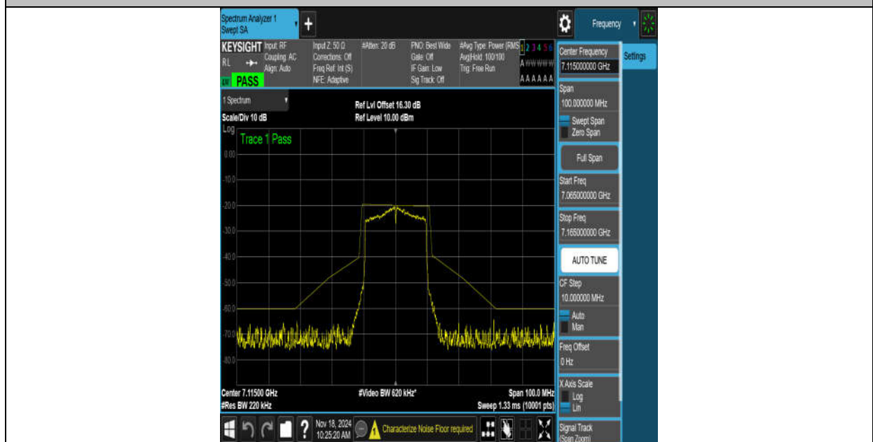
NTNV-11AX20MIMO-Ant8-7115-PASS
