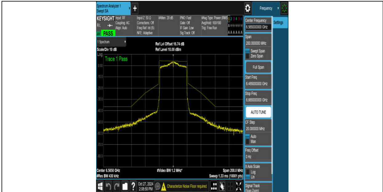
NTNV-11AX40MIMO-Ant9-6565-PASS
