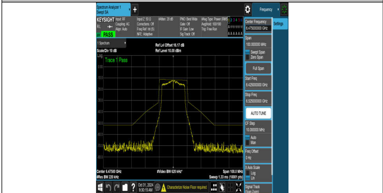
NTNV-11A-Ant8-6475-PASS
