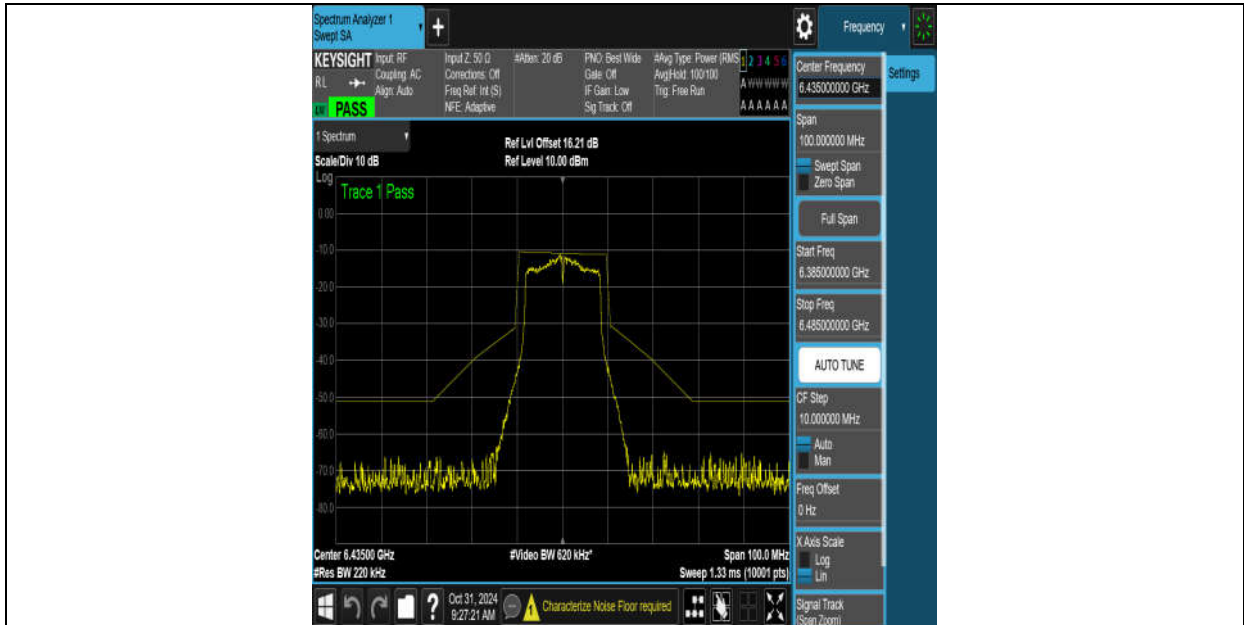
NTNV-11A-Ant9-6435-PASS
