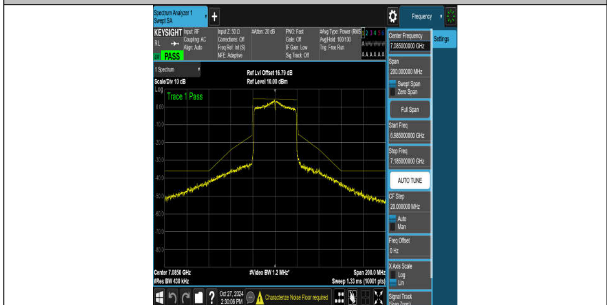
NTNV-11AX40MIMO-Ant8-7085-PASS
