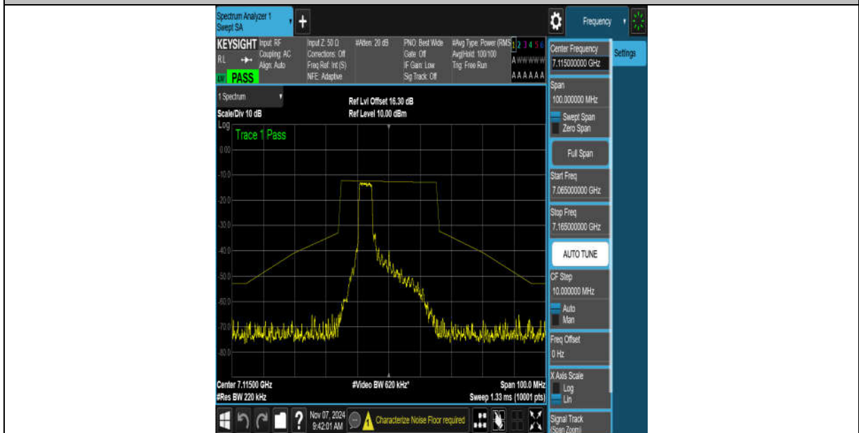
NTNV-11AX20MIMO-Ant8-7115-52Tone-RU37-PASS
