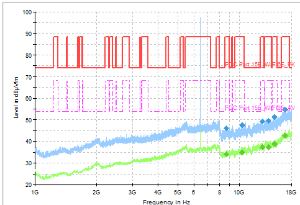
Fig. 25 Transmitter Spurious Emission (802.11ax-HE20, CH97, 1GHz-18GHz)
