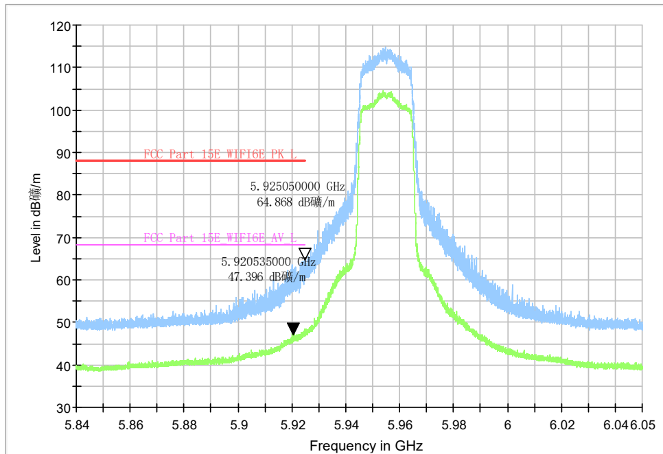
Fig. 3 Band Edges (802.11ax-HE20, CH1 5955MHz)
