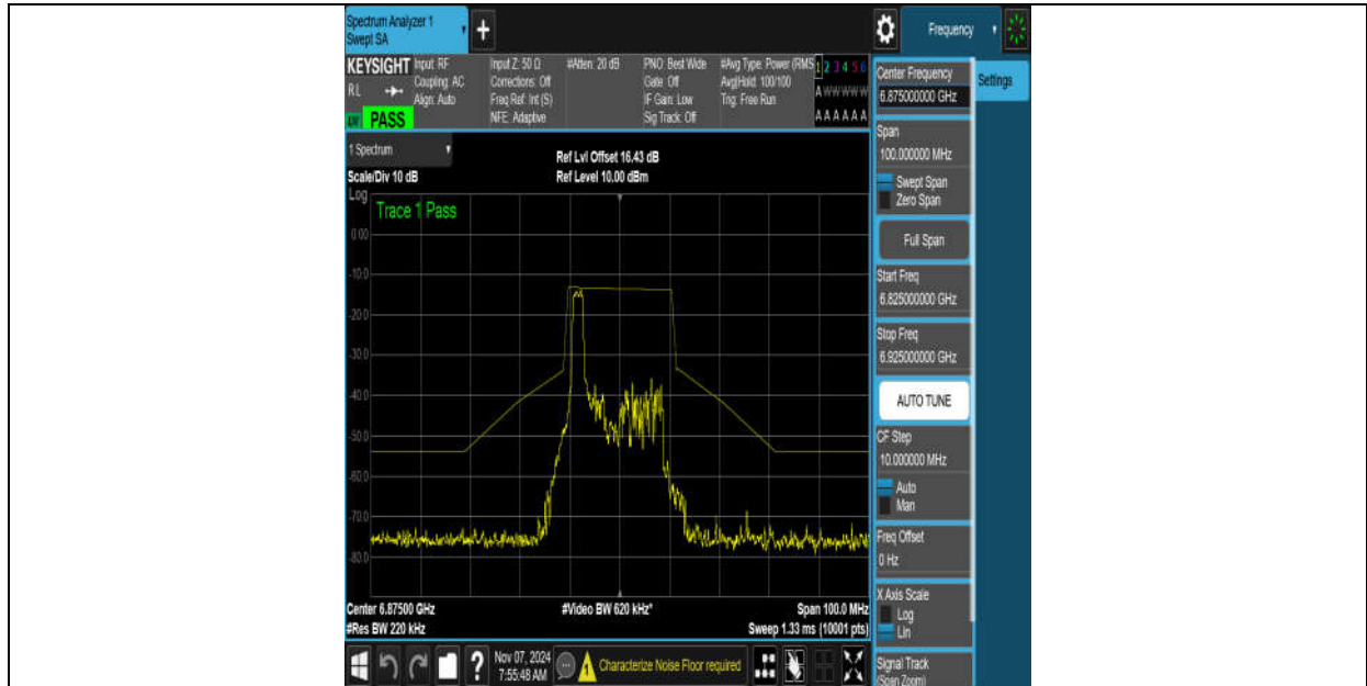
NTNV-11AX20MIMO-Ant9-6875-26Tone-RU0-PASS
