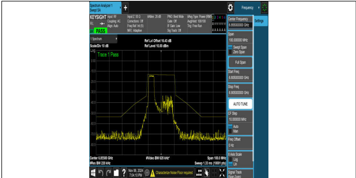
NTNV-11AX20MIMO-Ant9-6855-52Tone-RU37-PASS
