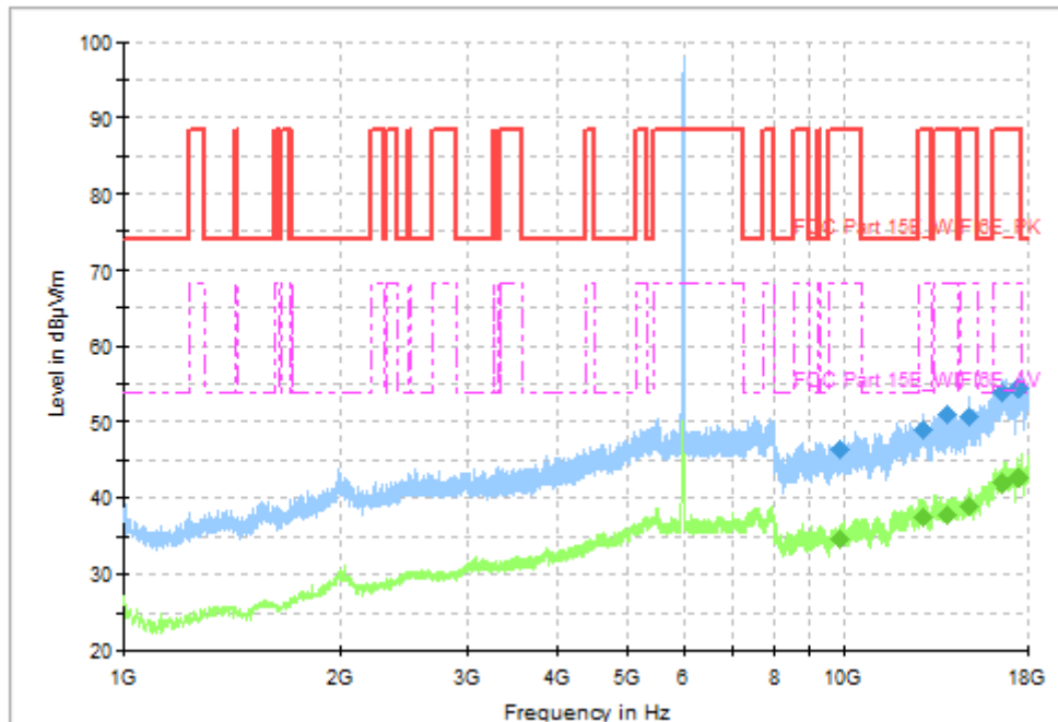
Fig. 43 Transmitter Spurious Emission (802.11ax-HE80, CH7, 1GHz-18GHz)
