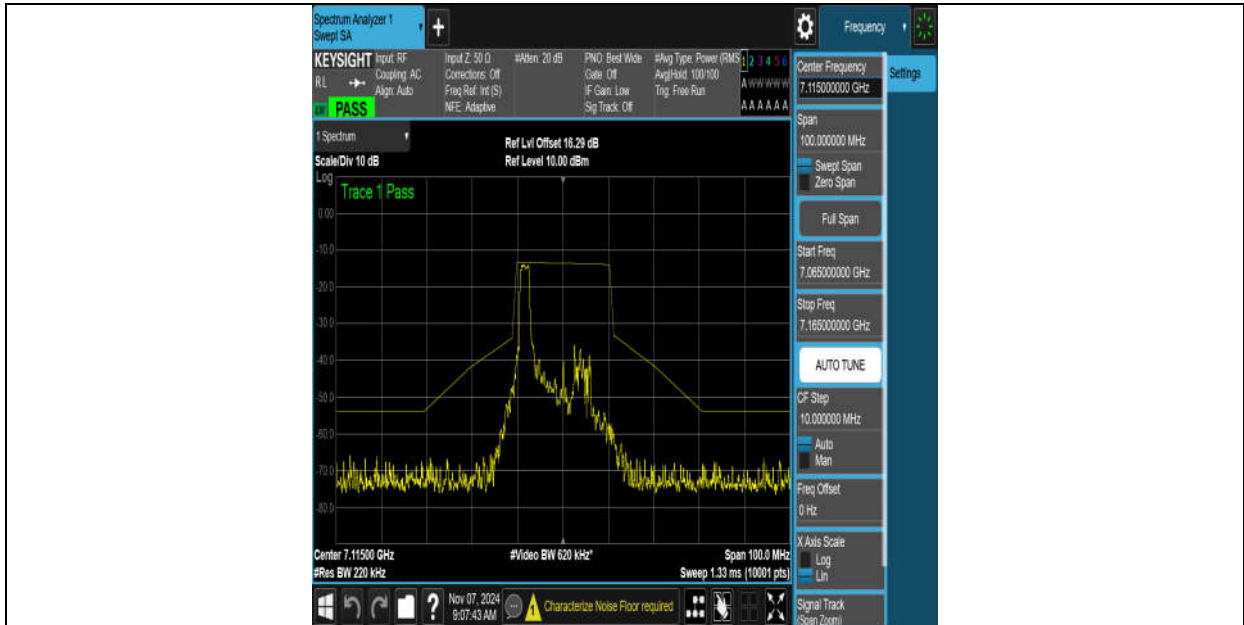
NTNV-11AX20MIMO-Ant9-7115-26Tone-RU0-PASS
