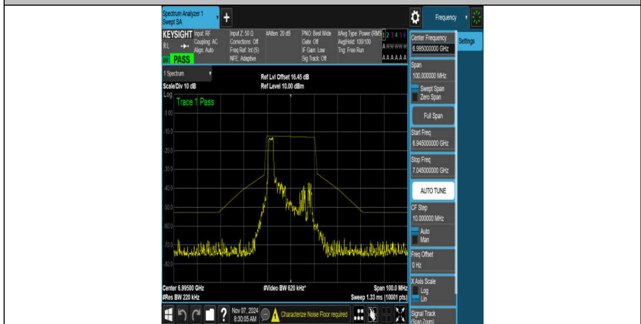
NTNV-11AX20MIMO-Ant8-6995-26Tone-RU0-PASS
