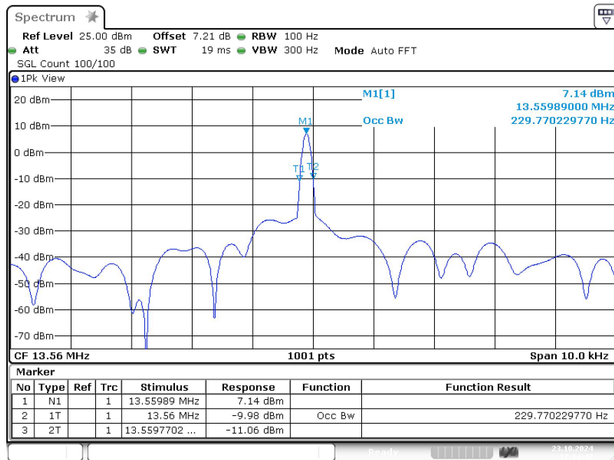
Figure A-7 Occupied Bandwidth
