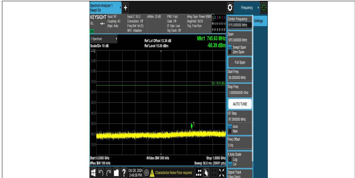
BLE_1M-Ant8-2440-30~1000-PASS
