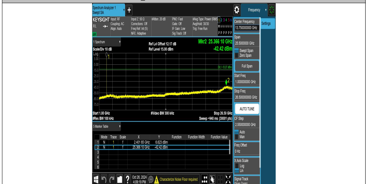
BLE_2M-Ant8-2402-1000~26500-PASS
