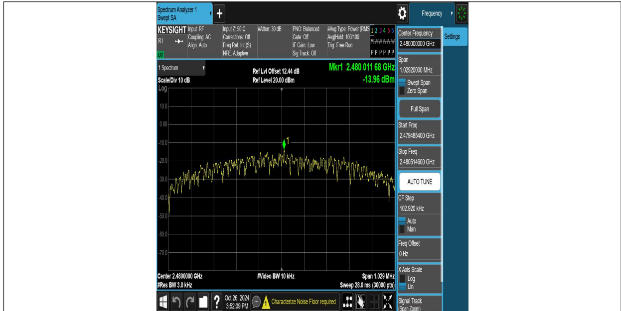
BLE_1M-Ant8-2480-PASS
