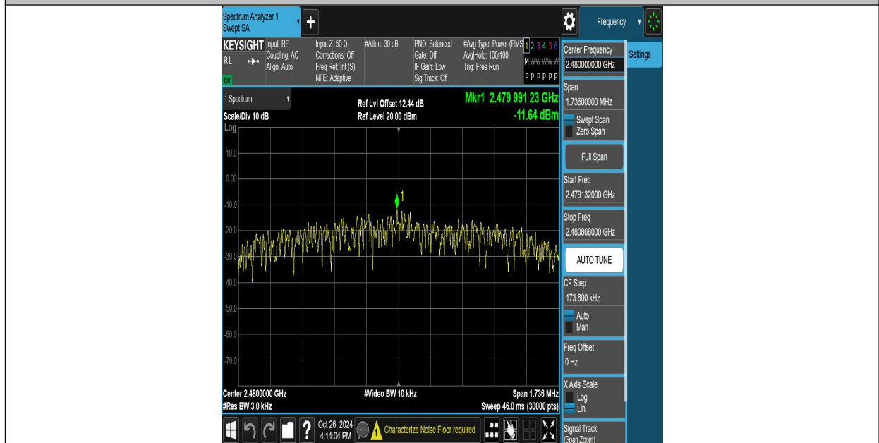
BLE_2M-Ant8-2480-PASS
