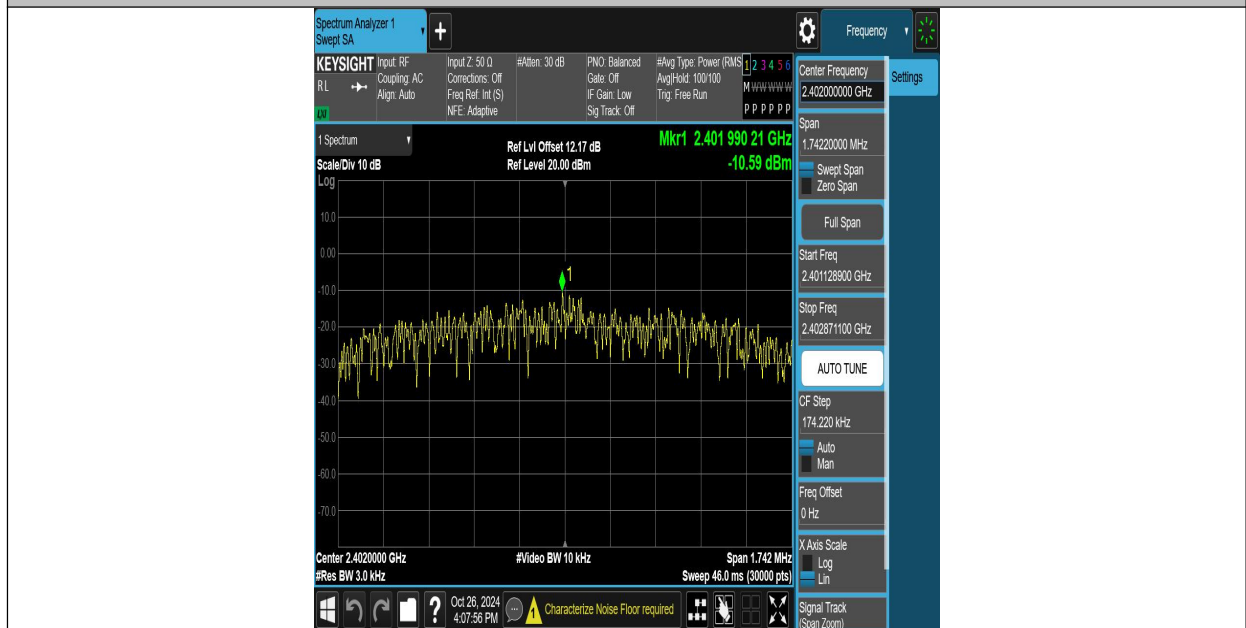
BLE_2M-Ant8-2402-PASS
