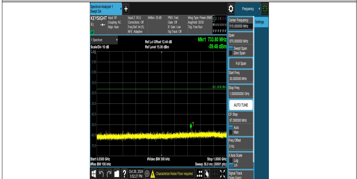
BLE_1M-Ant8-2480-30~1000-PASS
