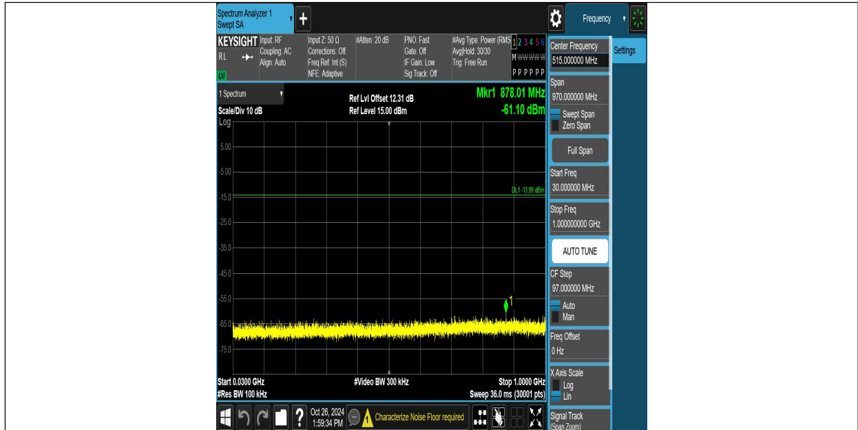
DH5-Ant8-2441-30~1000-PASS
