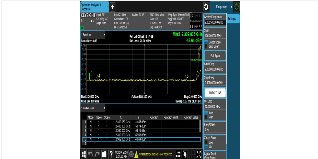
2DH5-Ant8-2402-PASS
