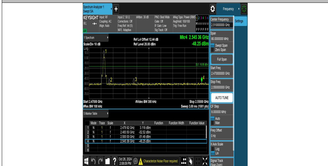
2DH5-Ant8-2480-PASS
