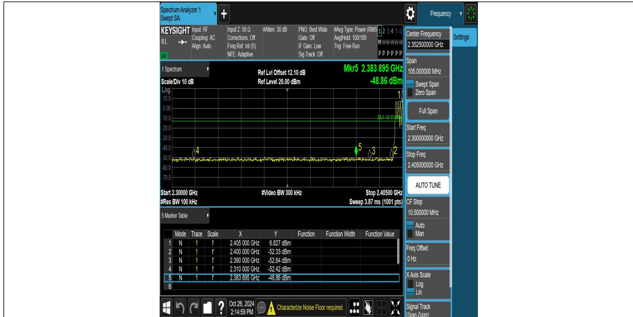
DH5-Ant8-Hop_2402-PASS
