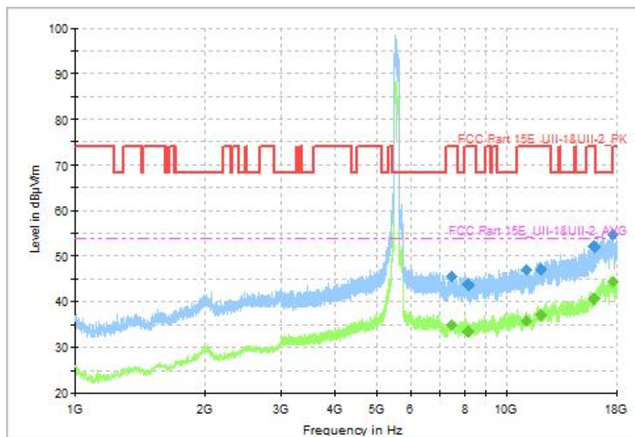
Fig. 65 Transmitter Spurious Emission (802.11ax-HE160, CH114 5570MHz, 1GHz-18GHz), MIMO
