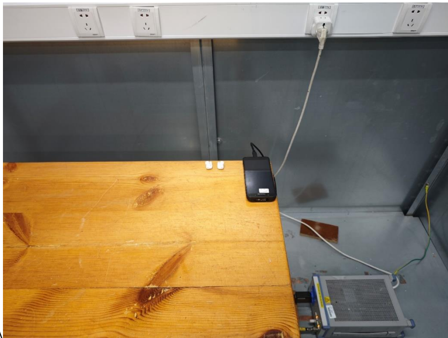
38. Conducted Emission (Part 15B, Bluetooth headset+ Charging)
