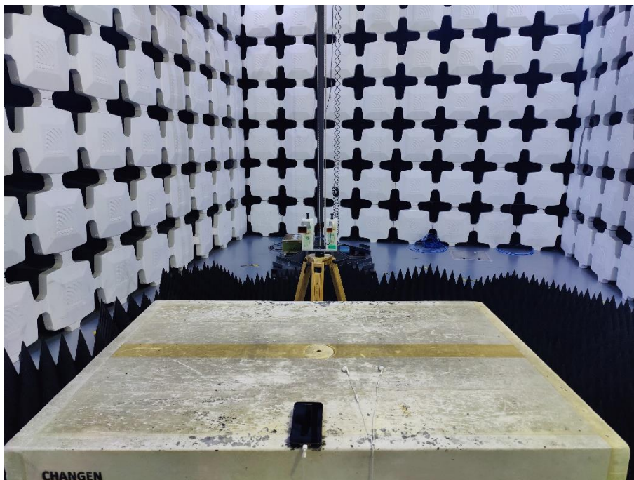
28. Radiated Emissions (Part 15B Band 5GHz Wi-Fi+Bluetooth+headset+Front Camera+microphone,26.5GHz-40GHz)
