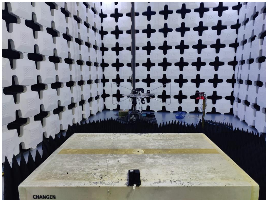
26. Radiated Emissions (Part 15B Band 5GHz Wi-Fi+Bluetooth+headset+Front Camera+microphone,1GHz-18GHz)
