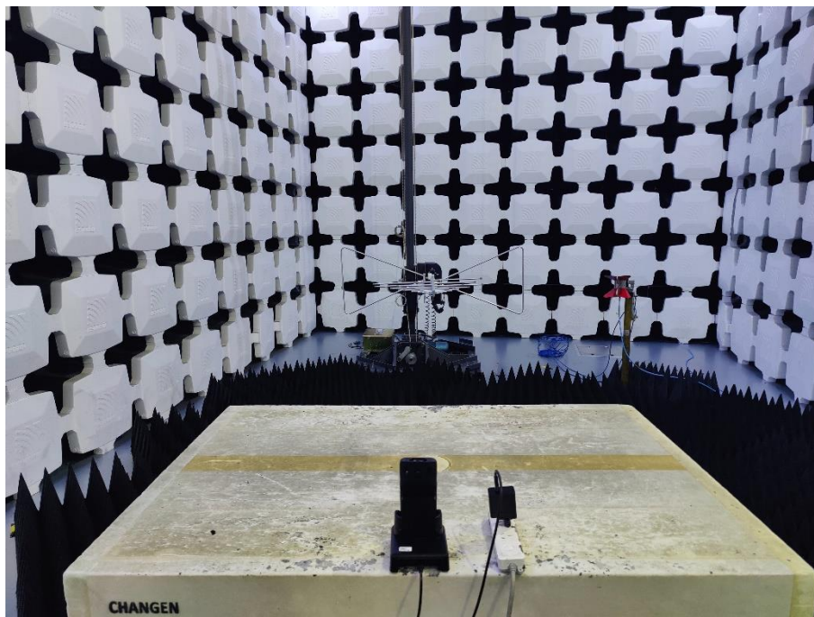
18. Radiated Emissions (Part 15B Wireless Power Transfer, 1GHz-18GHz)
