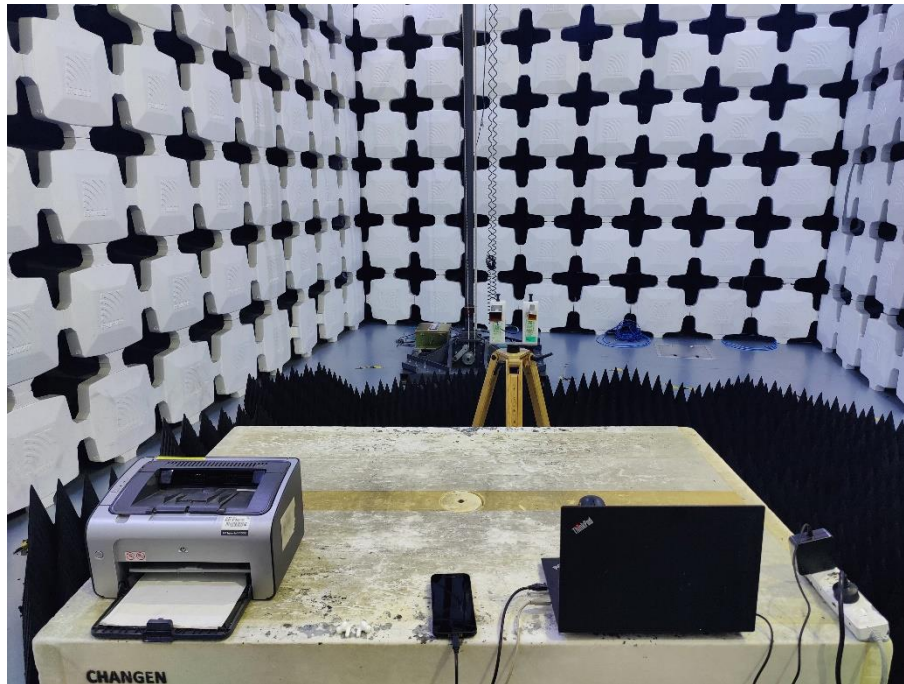
11. Radiated Emissions (Part 15B, Data Transfer+Bluetooth Headset, 18GHz-26.5GHz)
