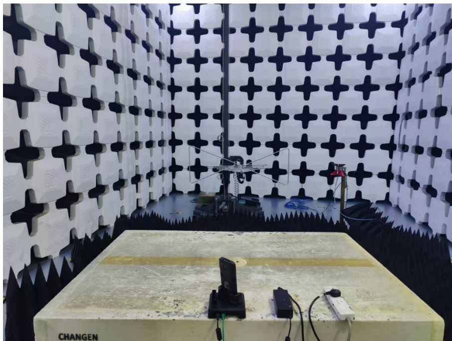
22. Radiated Emissions (Part 15B Charging via POGO PIN/Ethernet Connection, 1GHz-18GHz)
