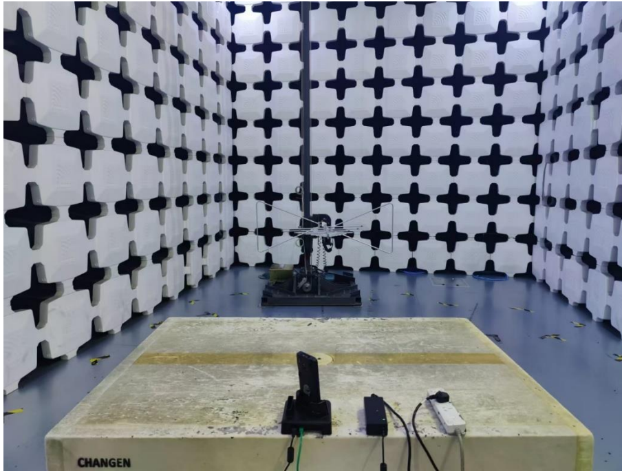
21. Radiated Emissions (Part 15B Charging via POGO PIN/Ethernet Connection, 30MHz-1GHz)
