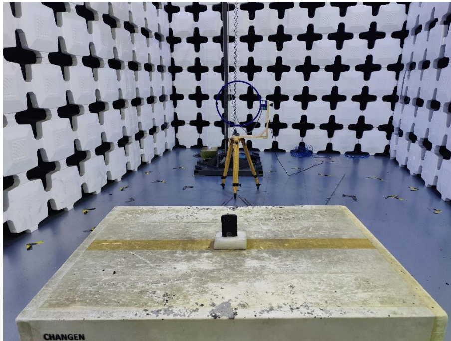
31. Radiated Emissions (Part 15C&Part 15E, 9kHz-30MHz)
