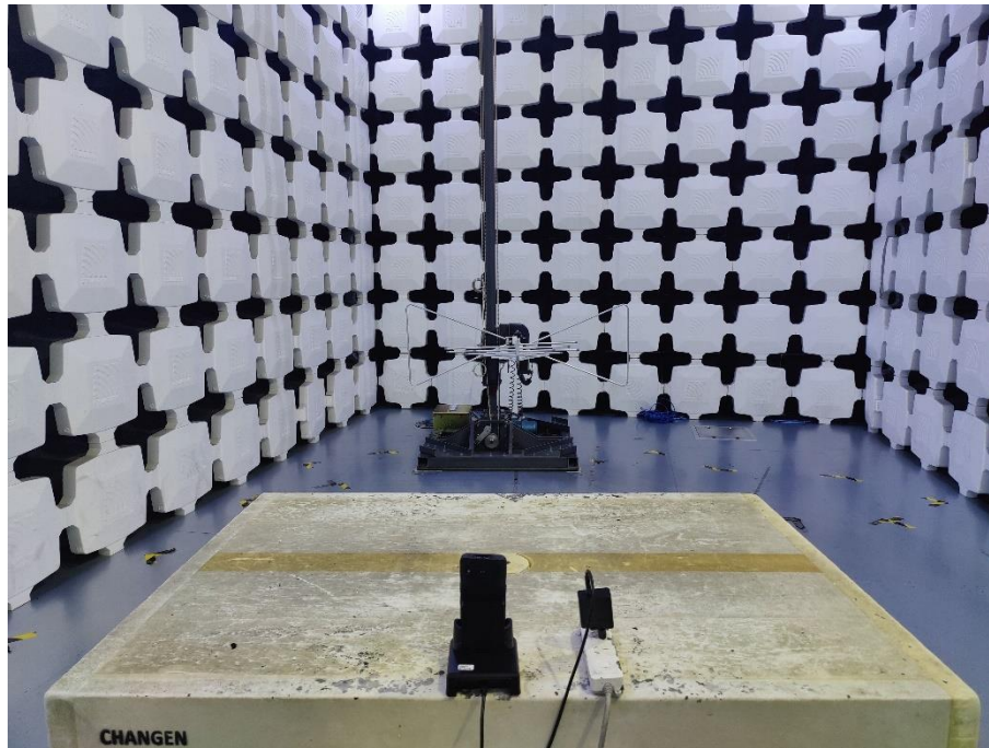
17. Radiated Emissions (Part 15B Wireless Power Transfer, 30MHz-1GHz)
