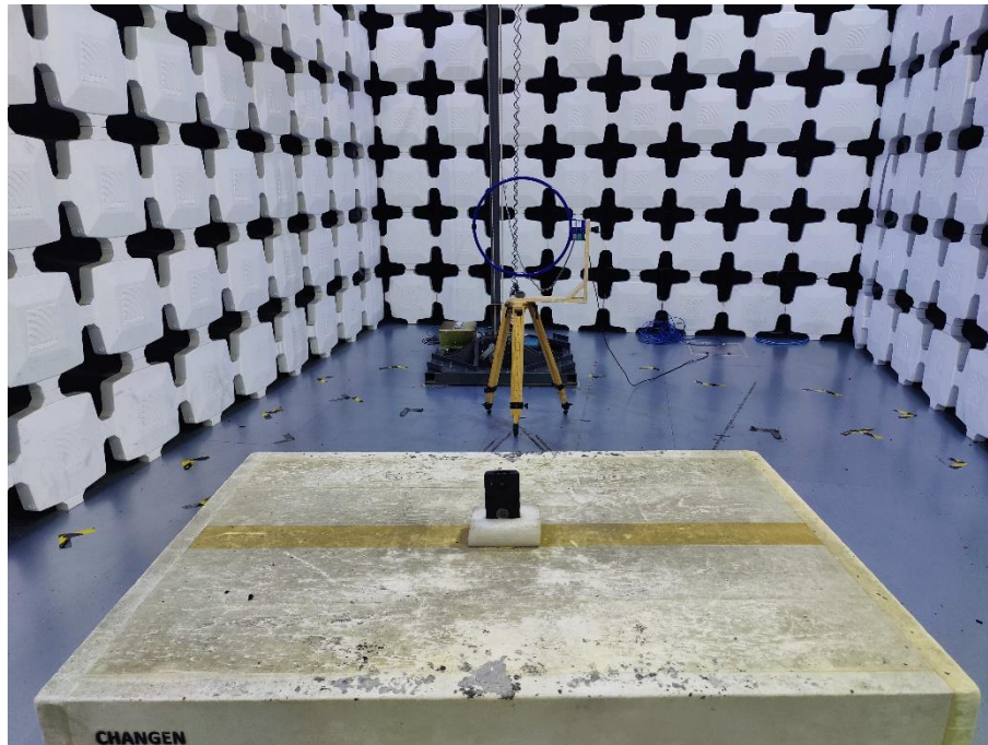
29. Radiated Emissions (Part 15C NFC, 9kHz-30MHz)
