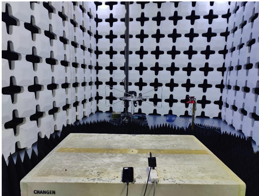
14. Radiated Emissions (Part 15B WiFi/Bluetooth/NFC/Camera/Video Player/Scanning/Glove mode/Charging,1GHz-18GHz)
