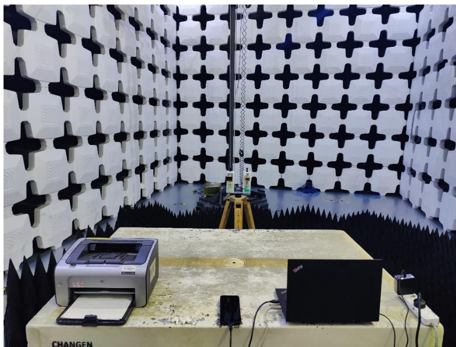
12. Radiated Emissions (Part 15B, Data Transfer+Bluetooth Headset, 26.5GHz-40GHz)
