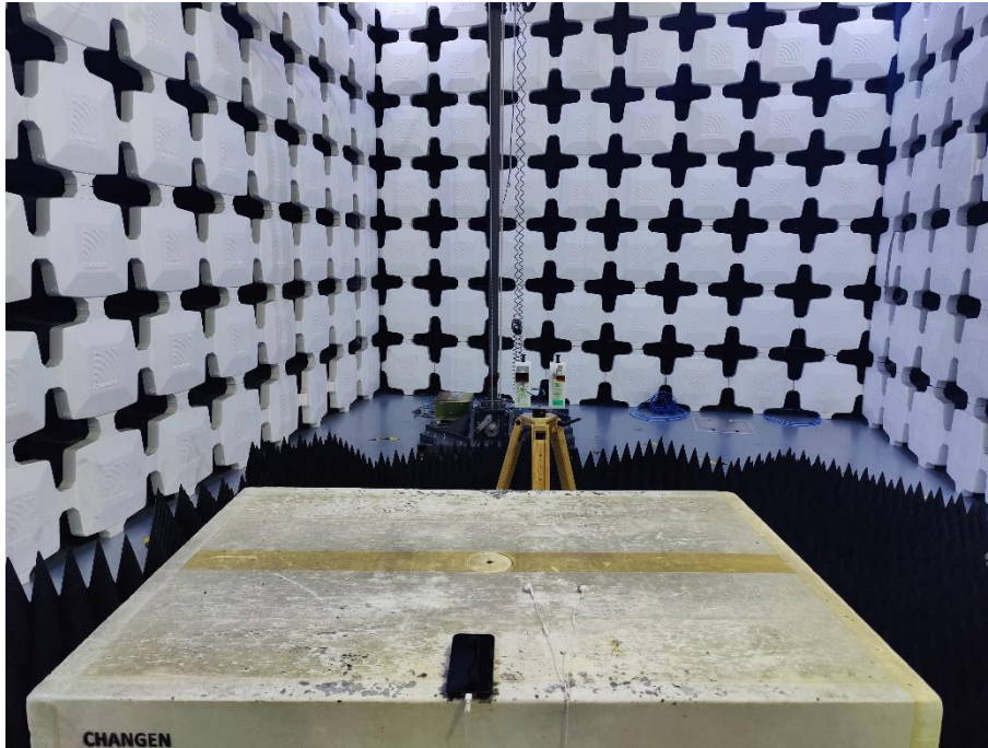
27. Radiated Emissions (Part 15B Band 5GHz Wi-Fi+Bluetooth+headset+Front Camera+microphone,18GHz-26.5GHz)
