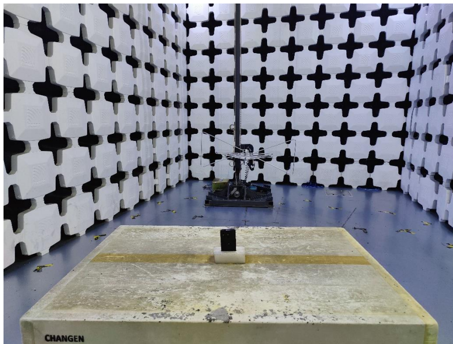
30. Radiated Emissions (Part 15C NFC, 30MHz-1GHz)
