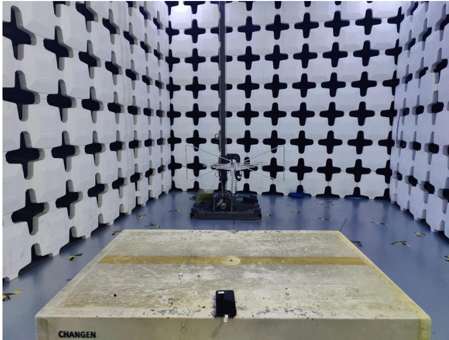
25. Radiated Emissions (Part 15B Band 5GHz Wi-Fi+Bluetooth+headset+Front Camera+microphone,30MHz-1GHz)
