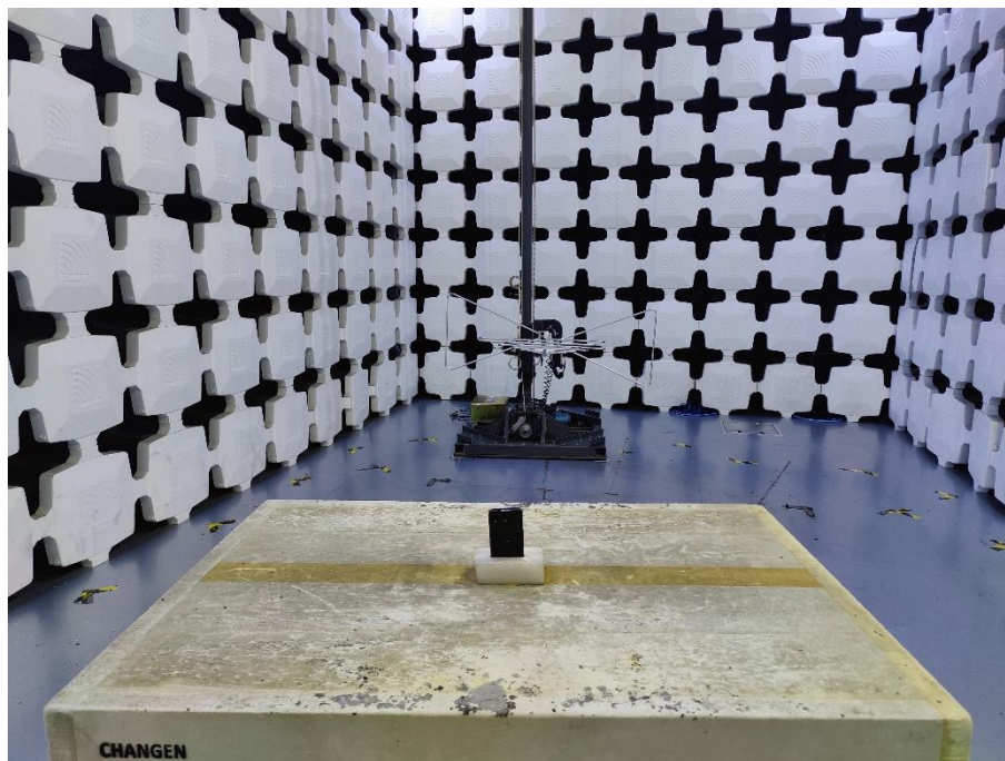
32. Radiated Emissions (Part 15C&Part 15E,30MHz-1GHz)
