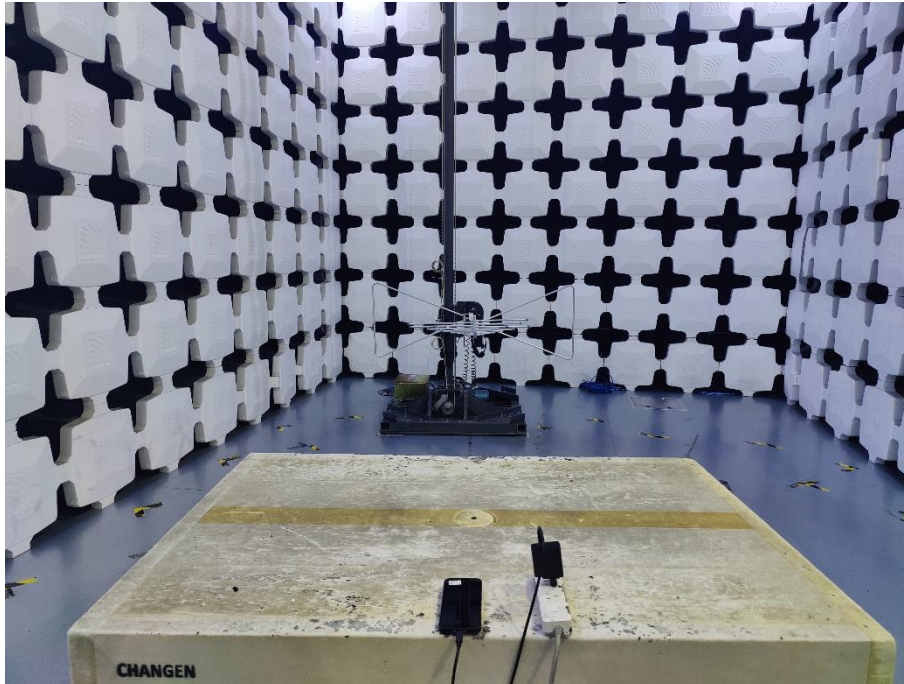
13. Radiated Emissions (Part 15B WiFi/Bluetooth/NFC/Camera/Video Player/Scanning/Glove mode/Charging,30MHz-1GHz)
