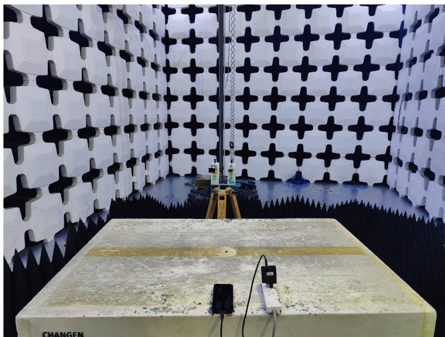
16. Radiated Emissions (Part 15B WiFi/Bluetooth/NFC/Camera/Video Player/Scanning/Glove mode/Charging,26.5GHz-40GHz)
