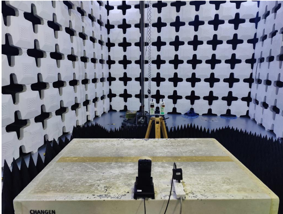
19. Radiated Emissions (Part 15B Wireless Power Transfer,18GHz-26.5GHz)
