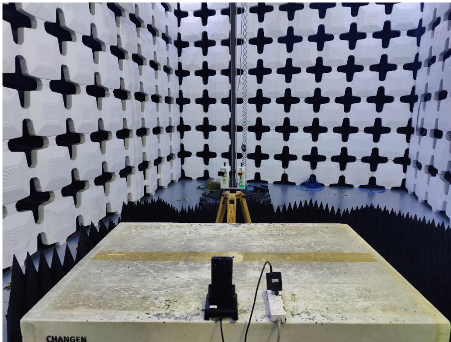
20. Radiated Emissions (Part 15B Wireless Power Transfer,26.5GHz-40GHz)
