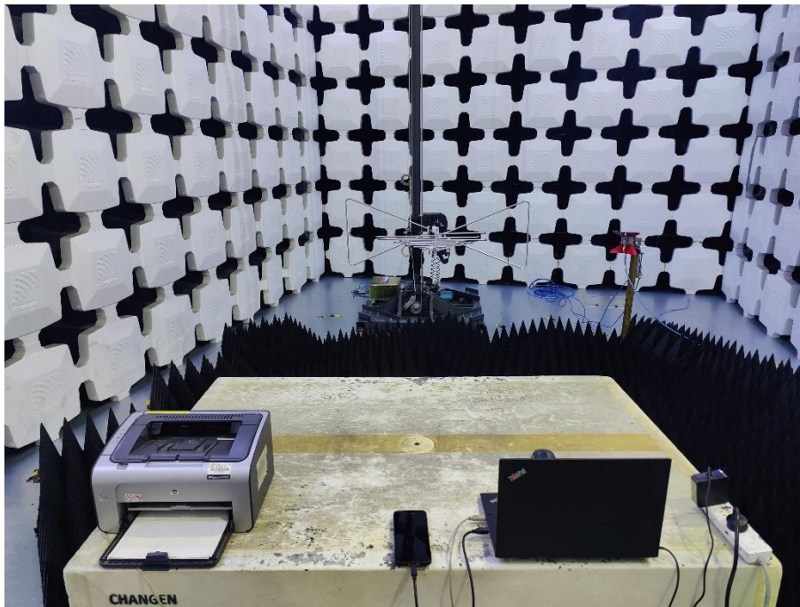
2. Radiated Emissions (Part 15B, Data Transfer, 1GHz-18GHz)
