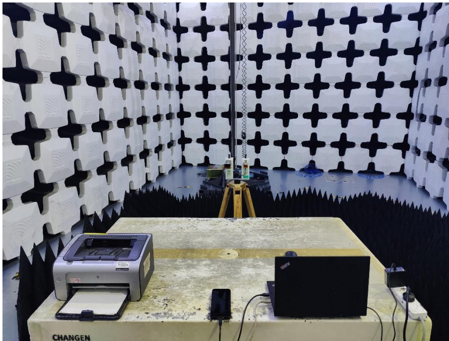
4. Radiated Emissions (Part 15B, Data Transfer, 26.5GHz-40GHz)
