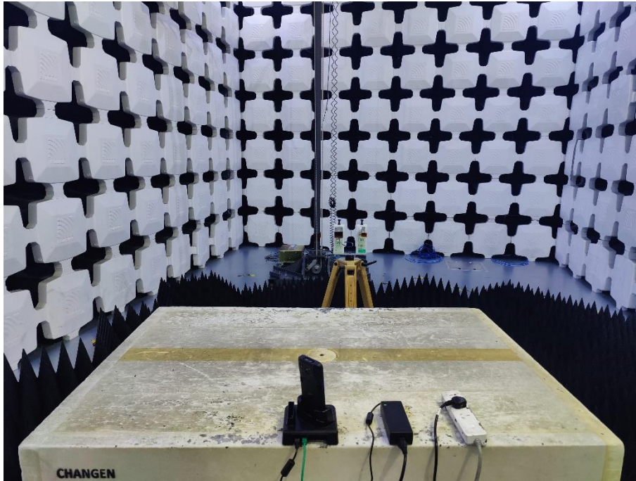
23. Radiated Emissions (Part 15B Charging via POGO PIN/Ethernet Connection,18GHz-26.5GHz)
