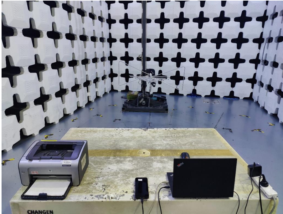
9. Radiated Emissions (Part 15B, Data Transfer+Bluetooth Headset, 30MHz-1GHz)
