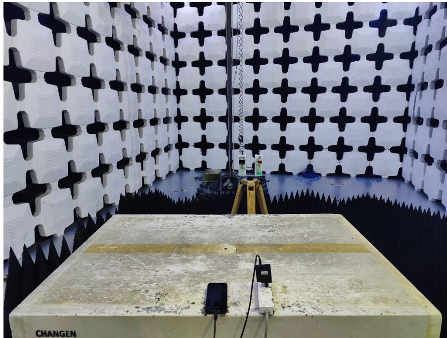
15. Radiated Emissions (Part 15B WiFi/Bluetooth/NFC/Camera/Video Player/Scanning/Glove mode/Charging,18GHz-26.5GHz)
