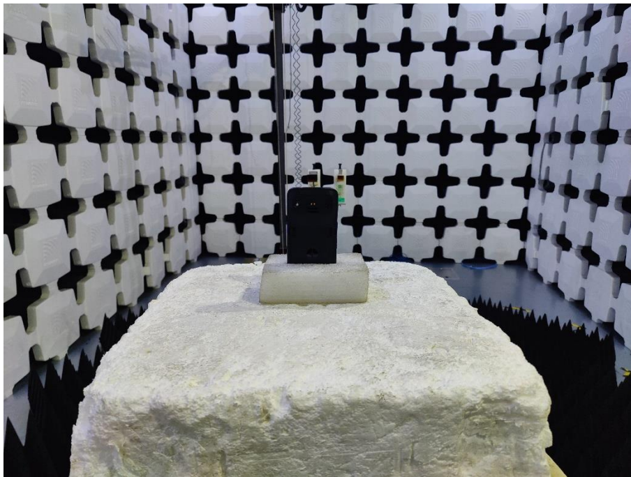
34. Radiated Emissions (Part 15C&Part 15E, 18GHz -26.5GHz)
