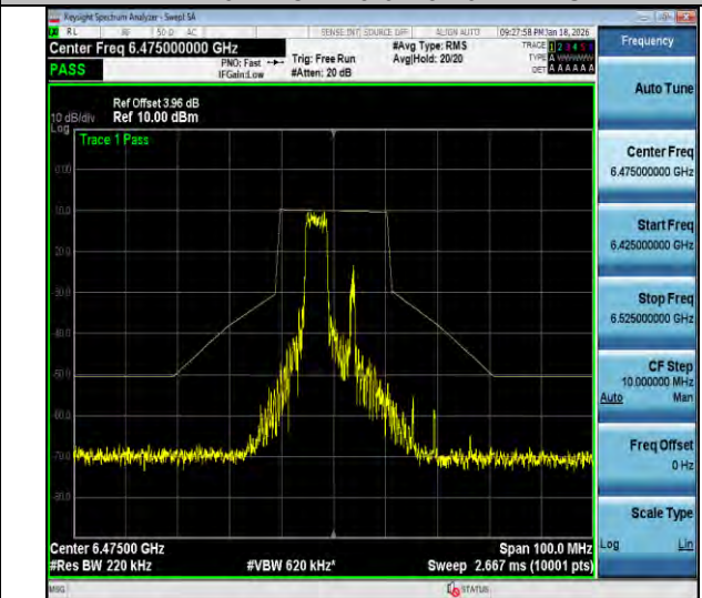
NTVN-11ax20MIMO-Ant3-6475-52Tone-RU39-PASS
