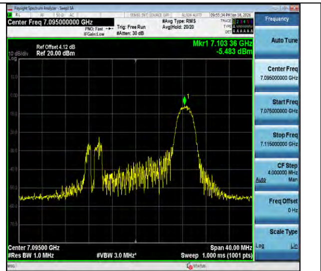
11ax20MIMO-Ant3-7095-26Tone-RU8-PASS
