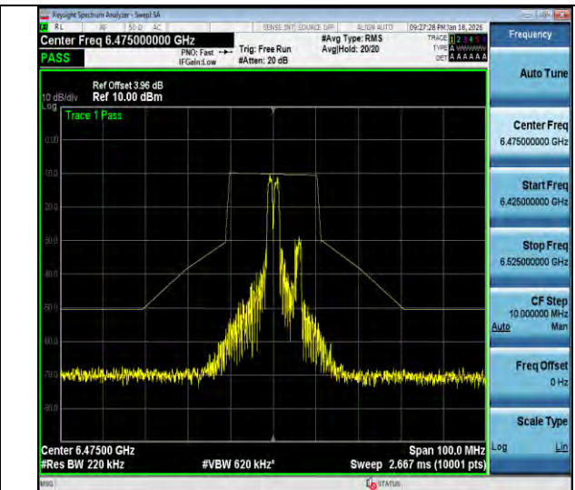
NTVN-11ax20MIMO-Ant3-6475-26Tone-RU4-PASS
