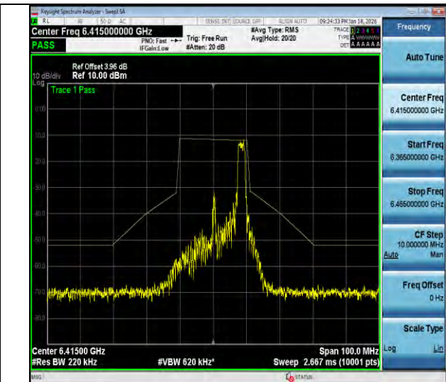
NTVN-11ax20MIMO-Ant3-6415-26Tone-RU8-PASS
