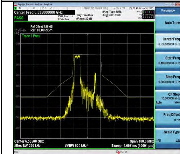
NTVN-11ax20MIMO-Ant2-6535-52Tone-RU37-PASS
