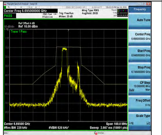
NTVN-11ax20MIMO-Ant3-6695-52Tone-RU39-PASS
