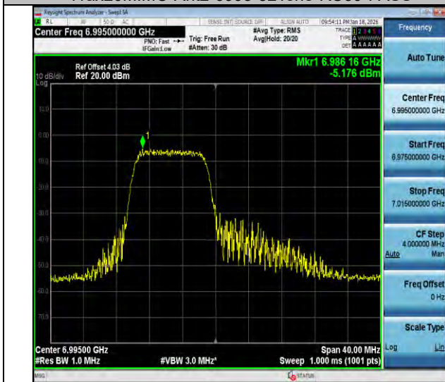
11ax20MIMO-Ant2-6995-106Tone-RU53-PASS
