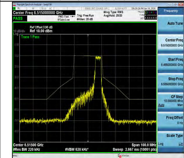
NTVN-11ax20MIMO-Ant3-6515-52Tone-RU40-PASS
