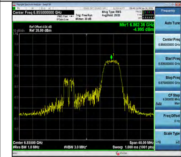
11ax20MIMO-Ant2-6855-52Tone-RU40-PASS
