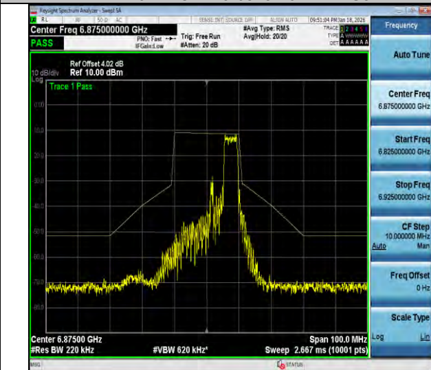
NTVN-11ax20MIMO-Ant3-6875-52Tone-RU40-PASS
