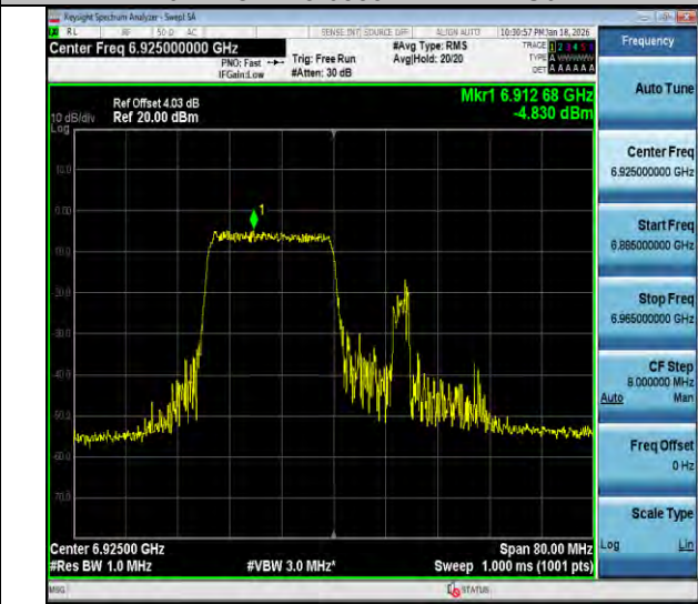
11ax40MIMO-Ant2-6925-242Tone-RU61-PASS
