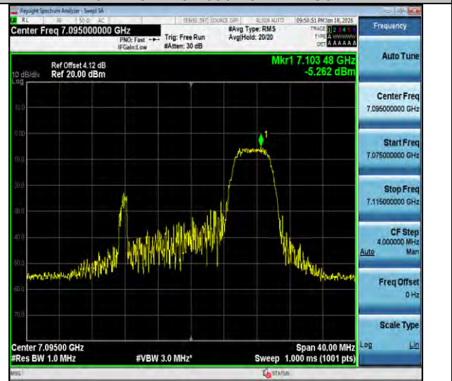
11ax20MIMO-Ant3-7095-52Tone-RU40-PASS
