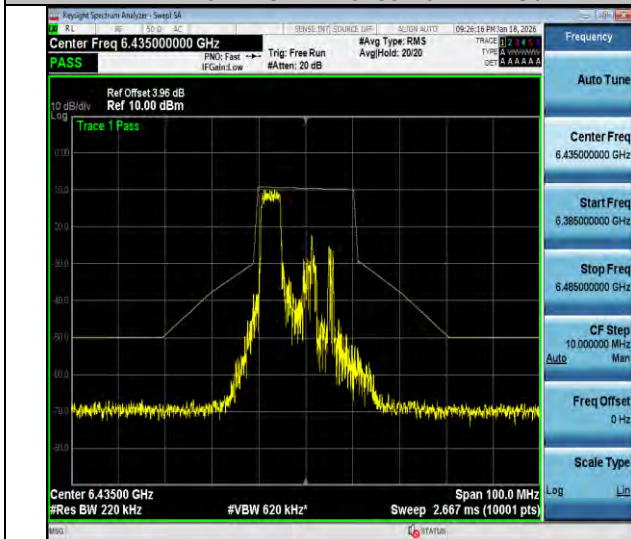
NTVN-11ax20MIMO-Ant2-6435-52Tone-RU37-PASS
