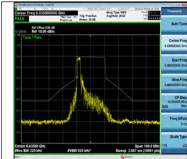
NTVN-11ax20MIMO-Ant2-6435-26Tone-RU0-PASS
