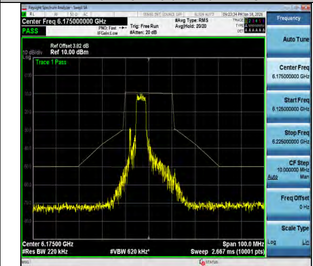
NTVN-11ax20MIMO-Ant3-6175-52Tone-RU39-PASS
