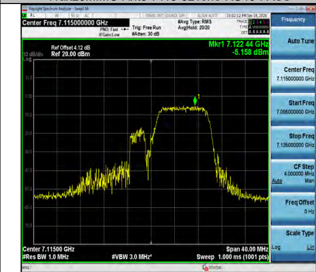
11ax20MIMO-Ant3-7115-106Tone-RU54-PASS
