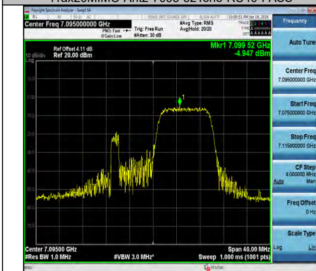
11ax20MIMO-Ant3-7095-106Tone-RU54-PASS
