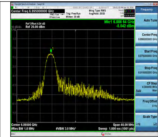
11ax20MIMO-Ant3-6895-26Tone-RU0-PASS
