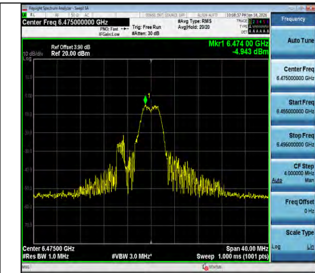
11ax20MIMO-Ant3-6475-26Tone-RU4-PASS
