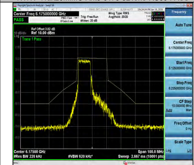
NTVN-11ax20MIMO-Ant3-6175-106Tone-RU53-PASS
