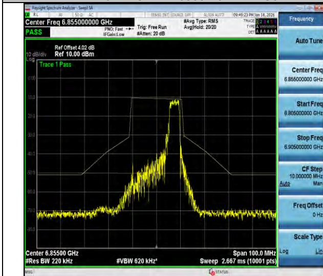
NTVN-11ax20MIMO-Ant2-6855-52Tone-RU40-PASS
