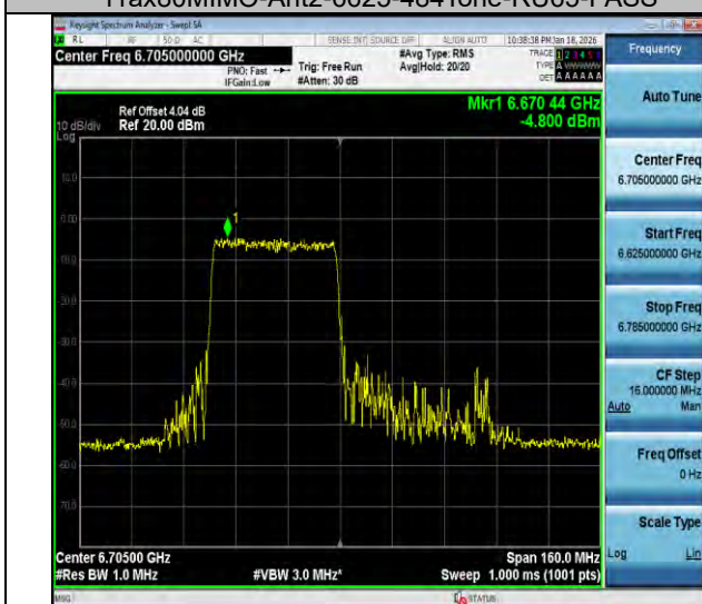
11ax80MIMO-Ant2-6705-484Tone-RU65-PASS
