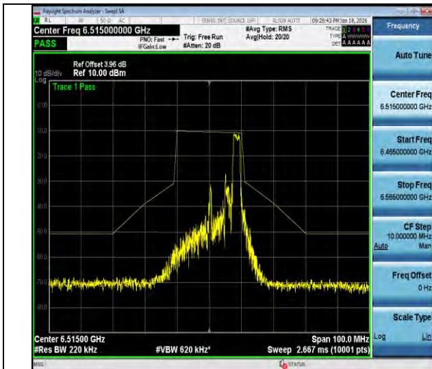
NTVN-11ax20MIMO-Ant2-6515-26Tone-RU8-PASS
