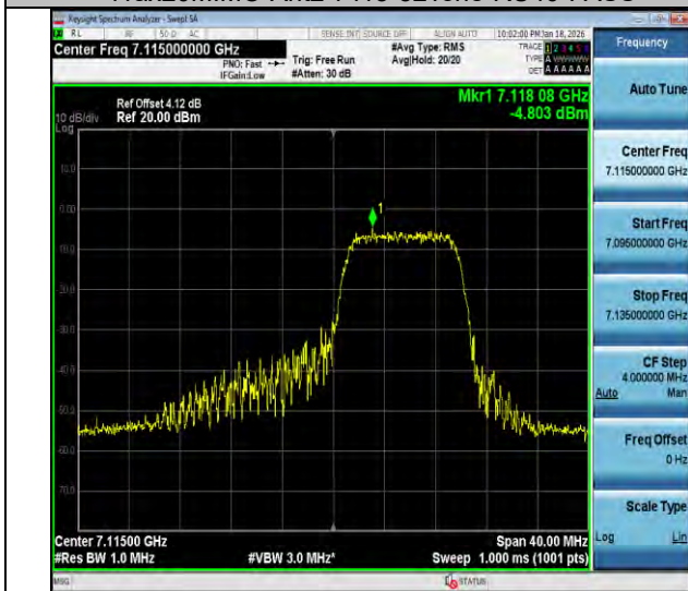
11ax20MIMO-Ant2-7115-106Tone-RU54-PASS
