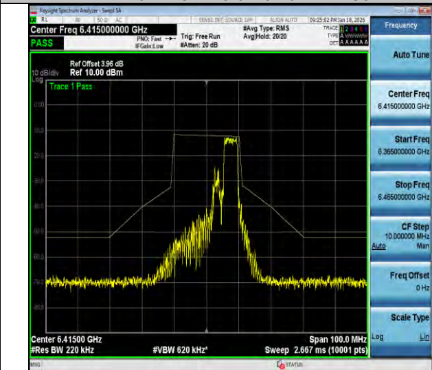
NTVN-11ax20MIMO-Ant3-6415-52Tone-RU40-PASS
