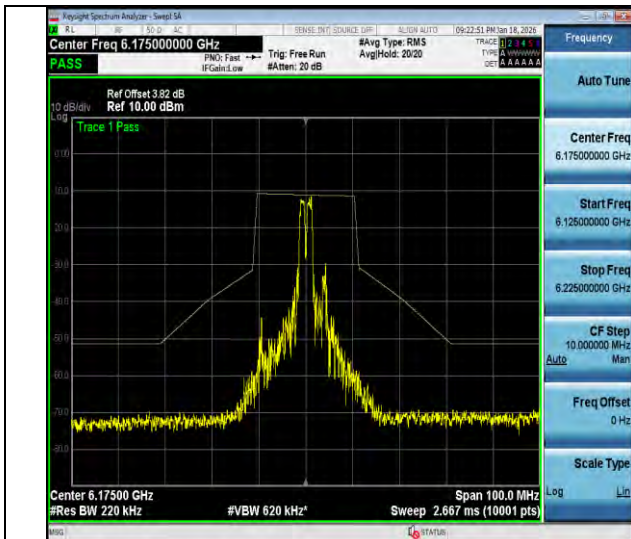
NTVN-11ax20MIMO-Ant2-6175-26Tone-RU4-PASS
