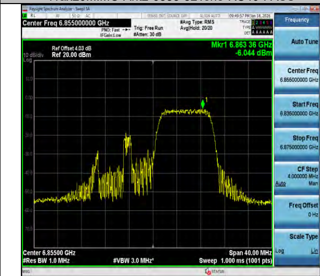
11ax20MIMO-Ant3-6855-106Tone-RU54-PASS
