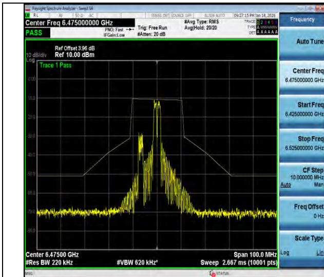
NTVN-11ax20MIMO-Ant2-6475-26Tone-RU4-PASS
