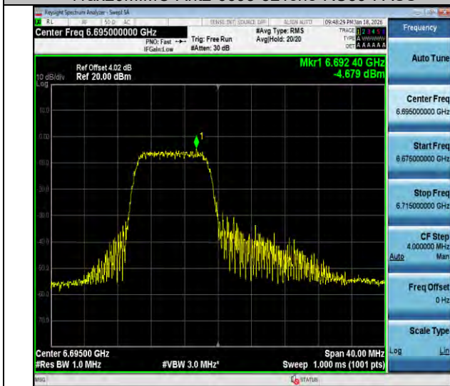
11ax20MIMO-Ant2-6695-106Tone-RU53-PASS
