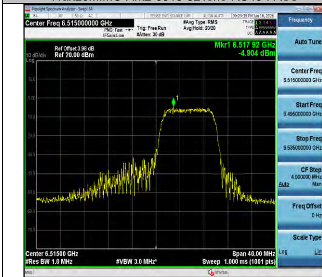
11ax20MIMO-Ant2-6515-106Tone-RU54-PASS
