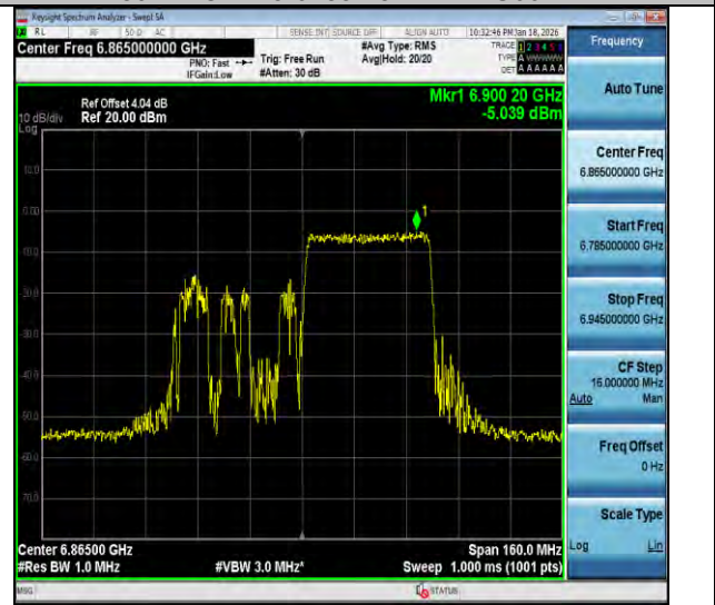
11ax80MIMO-Ant3-6865-484Tone-RU66-PASS
