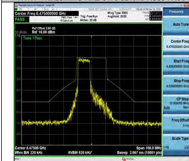
NTVN-11ax20MIMO-Ant2-6475-106Tone-RU53-PASS
