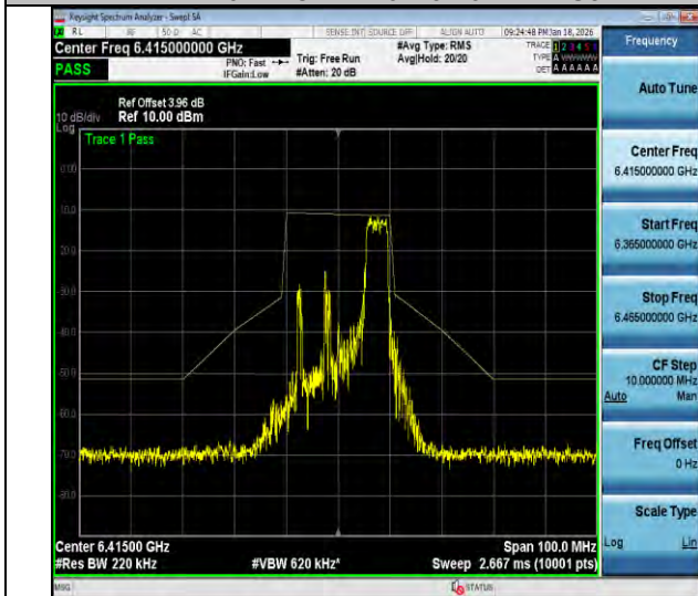
NTVN-11ax20MIMO-Ant2-6415-52Tone-RU40-PASS
