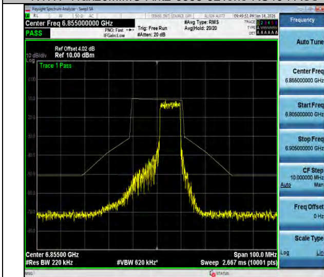
NTVN-11ax20MIMO-Ant2-6855-106Tone-RU54-PASS
