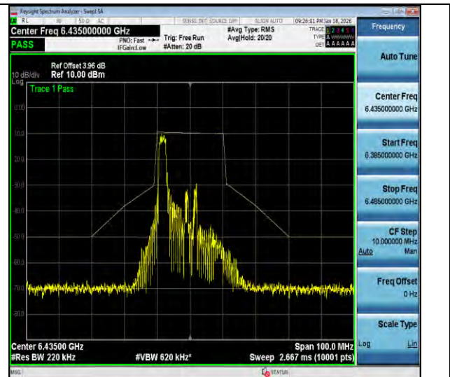
NTVN-11ax20MIMO-Ant3-6435-26Tone-RU0-PASS
