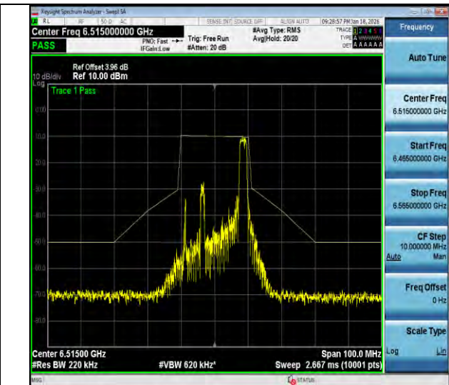
NTVN-11ax20MIMO-Ant3-6515-26Tone-RU8-PASS
