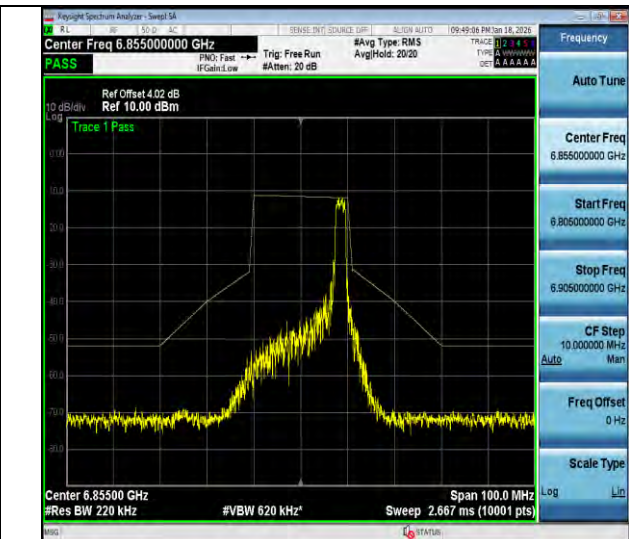
NTVN-11ax20MIMO-Ant3-6855-26Tone-RU8-PASS
