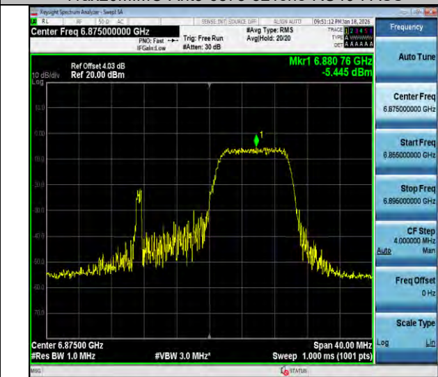
11ax20MIMO-Ant2-6875-106Tone-RU54-PASS
