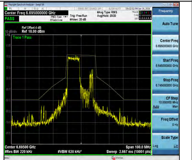
NTVN-11ax20MIMO-Ant3-6695-106Tone-RU53-PASS
