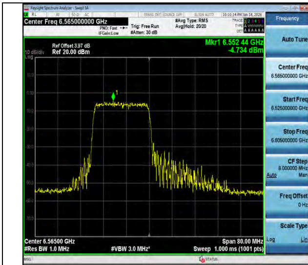
11ax40MIMO-Ant2-6565-242Tone-RU61-PASS
