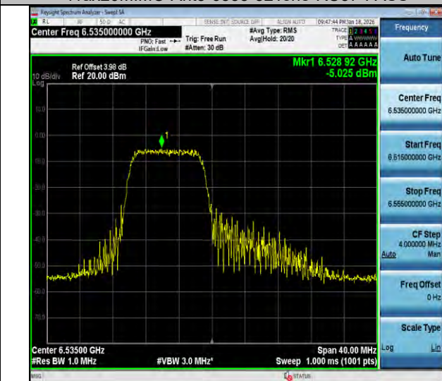
11ax20MIMO-Ant3-6535-106Tone-RU53-PASS
