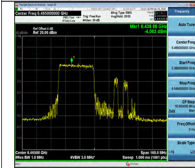
11ax80MIMO-Ant2-6465-484Tone-RU65-PASS
