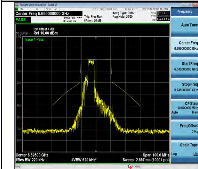
NTVN-11ax20MIMO-Ant2-6695-52Tone-RU39-PASS
