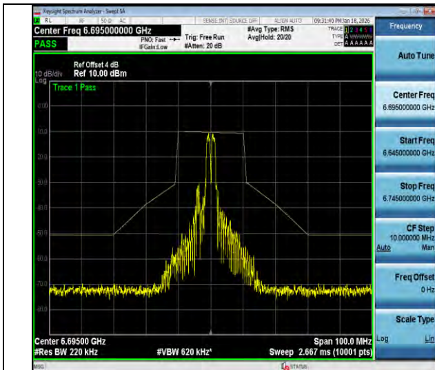
NTVN-11ax20MIMO-Ant2-6695-26Tone-RU4-PASS
