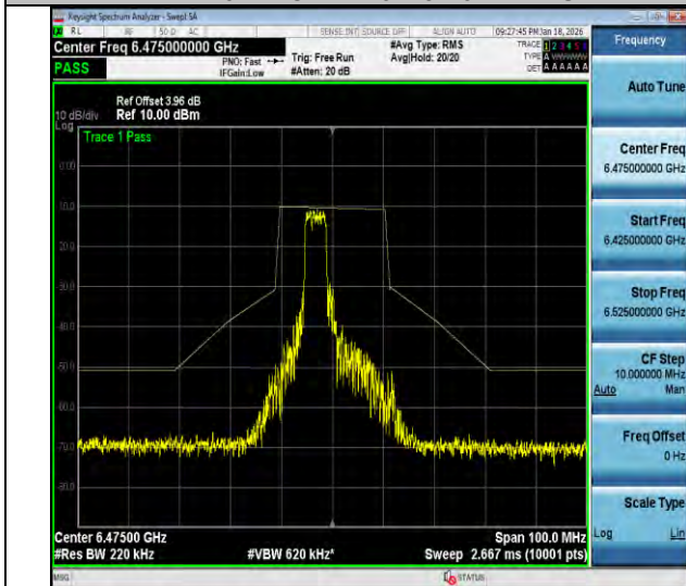
NTVN-11ax20MIMO-Ant2-6475-52Tone-RU39-PASS
