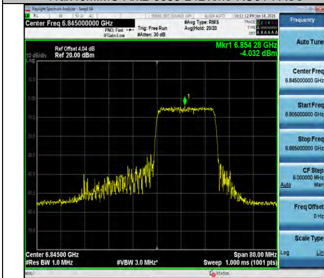
11ax40MIMO-Ant2-6845-242Tone-RU62-PASS
