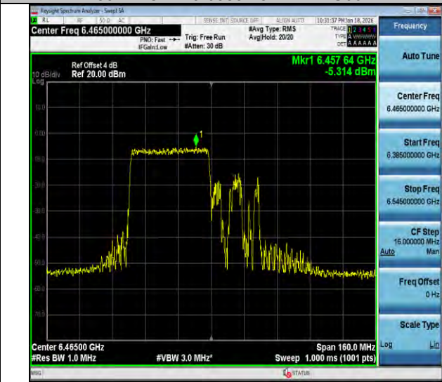
11ax80MIMO-Ant3-6465-484Tone-RU65-PASS
