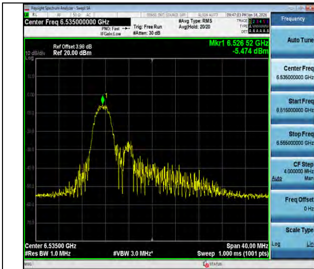
11ax20MIMO-Ant2-6535-26Tone-RU0-PASS
