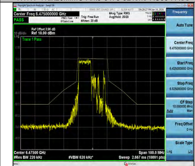
NTVN-11ax20MIMO-Ant3-6475-106Tone-RU53-PASS
