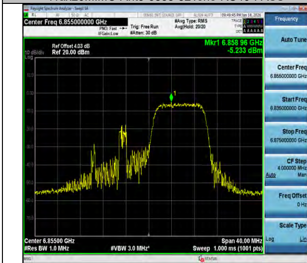
11ax20MIMO-Ant2-6855-106Tone-RU54-PASS
