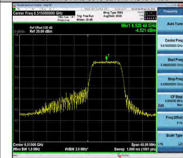
11ax20MIMO-Ant3-6515-106Tone-RU54-PASS
