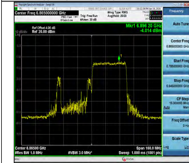
11ax80MIMO-Ant2-6865-484Tone-RU66-PASS
