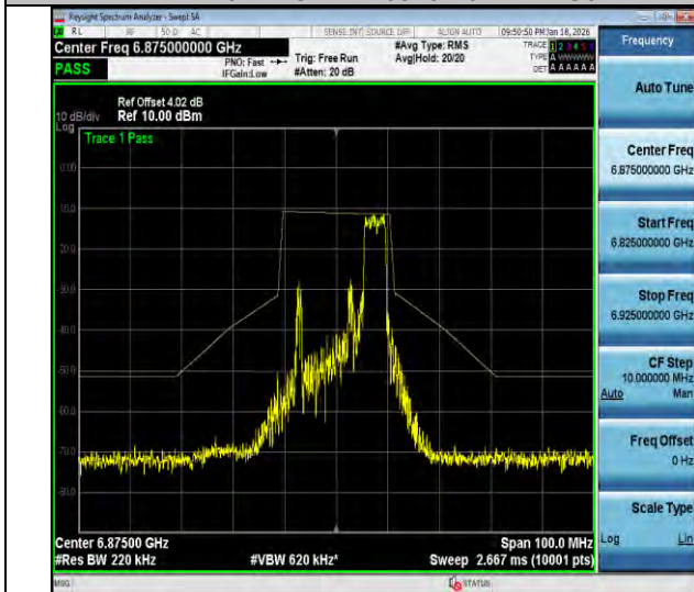
NTVN-11ax20MIMO-Ant2-6875-52Tone-RU40-PASS
