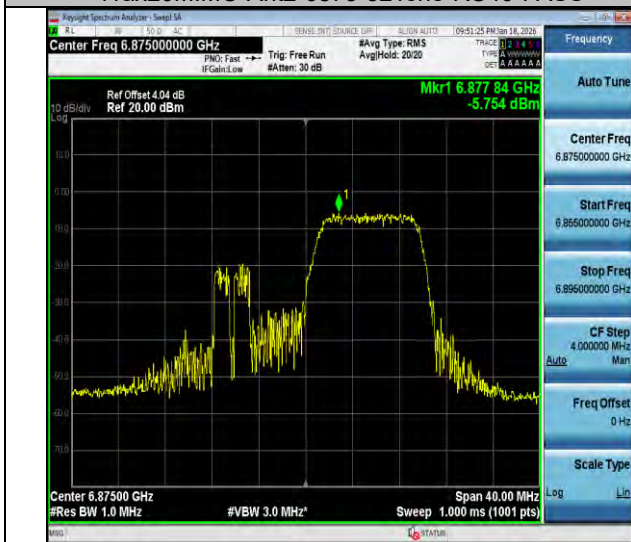
11ax20MIMO-Ant3-6875-106Tone-RU54-PASS
