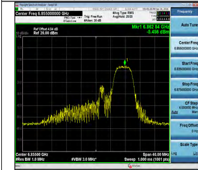
11ax20MIMO-Ant3-6855-52Tone-RU40-PASS
