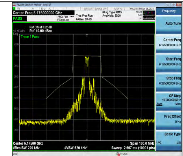
NTVN-11ax20MIMO-Ant3-6175-26Tone-RU4-PASS
