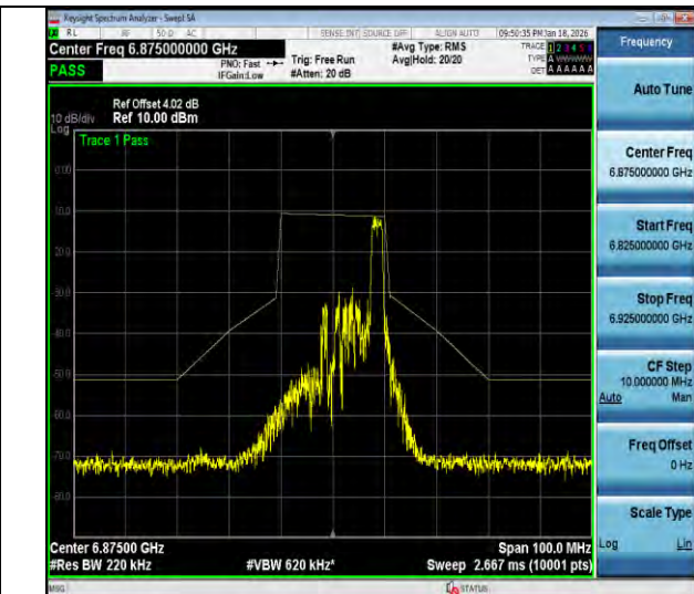
NTVN-11ax20MIMO-Ant3-6875-26Tone-RU8-PASS
