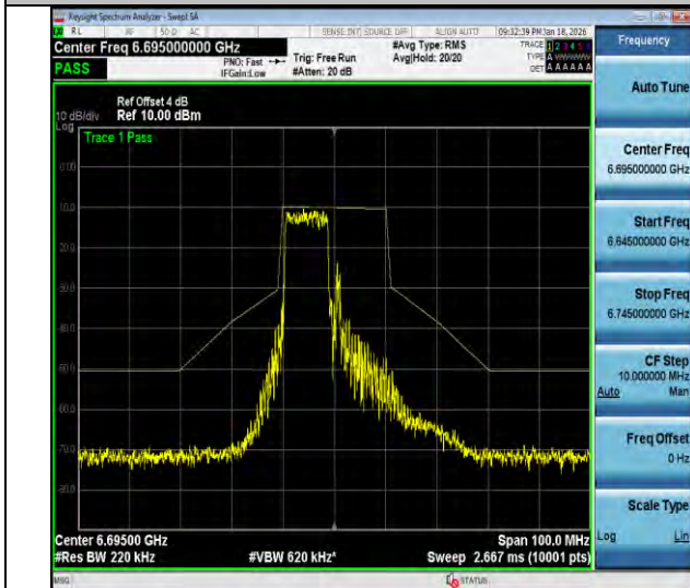
NTVN-11ax20MIMO-Ant2-6695-106Tone-RU53-PASS
