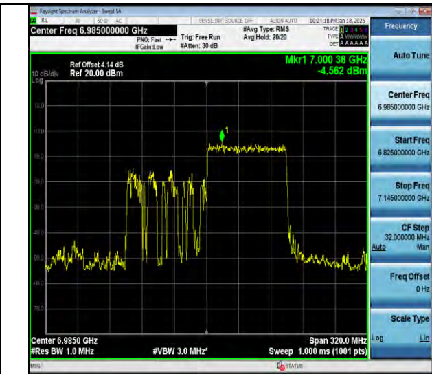
11ax160MIMO-Ant3-6985-996Tone-RU68-PASS
