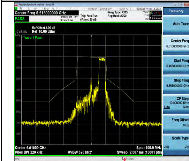
NTVN-11ax20MIMO-Ant2-6515-52Tone-RU40-PASS
