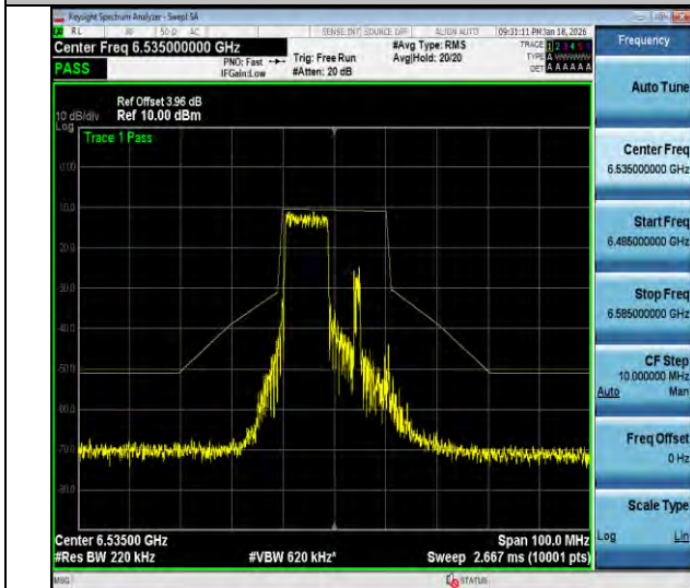
NTVN-11ax20MIMO-Ant2-6535-106Tone-RU53-PASS
