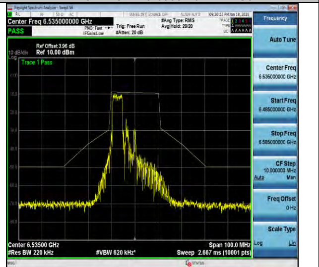
NTVN-11ax20MIMO-Ant3-6535-52Tone-RU37-PASS
