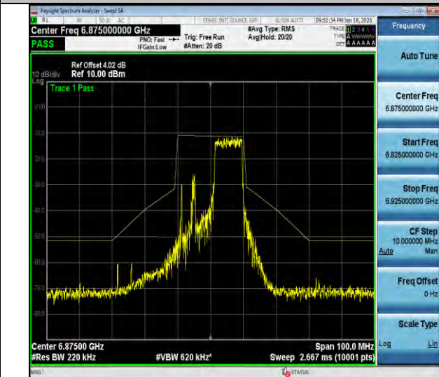
NTVN-11ax20MIMO-Ant3-6875-106Tone-RU54-PASS
