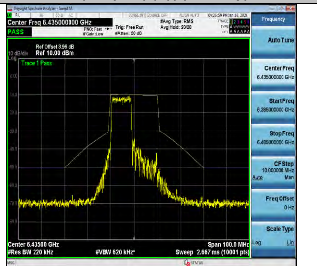
NTVN-11ax20MIMO-Ant3-6435-106Tone-RU53-PASS
