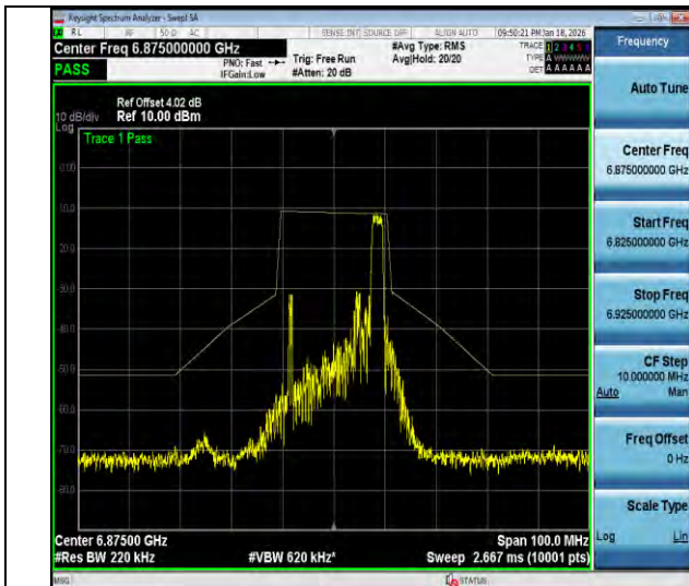
NTVN-11ax20MIMO-Ant2-6875-26Tone-RU8-PASS
