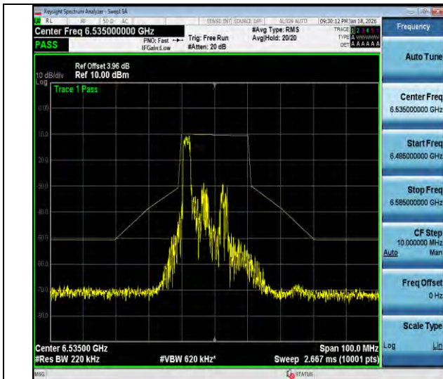
NTVN-11ax20MIMO-Ant2-6535-26Tone-RU0-PASS
