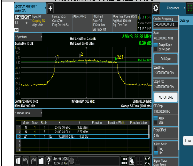
11ax40MIMO-Ant2-2437-PASS
