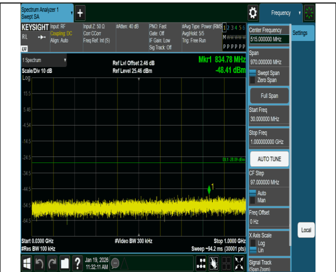
11ax40MIMO-Ant2-2452-30~1000-PASS
