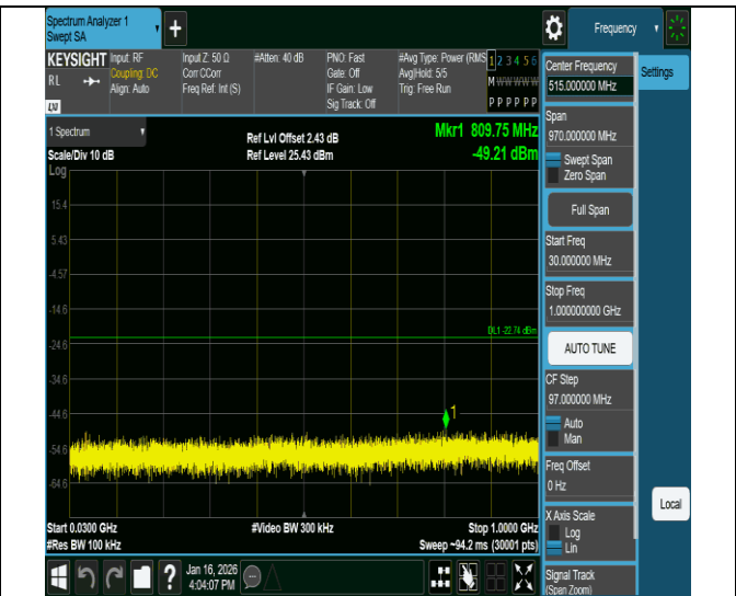
11ax20MIMO-Ant2-2437-30~1000-PASS
