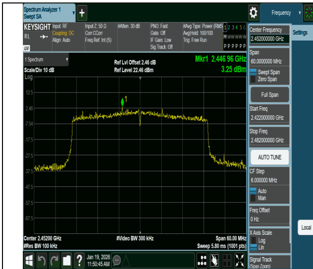
11ax40MIMO-Ant3-2452-0~Reference-PASS
