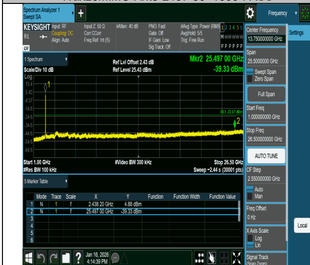
11ax20MIMO-Ant3-2437-1000~26500-PASS
