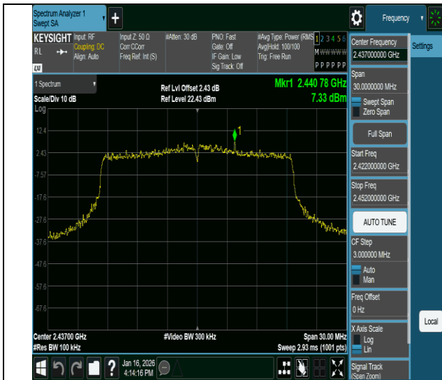
11ax20MIMO-Ant3-2437-0~Reference-PASS
