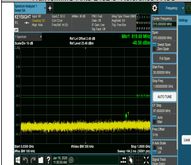
11ax40MIMO-Ant3-2452-30~1000-PASS
