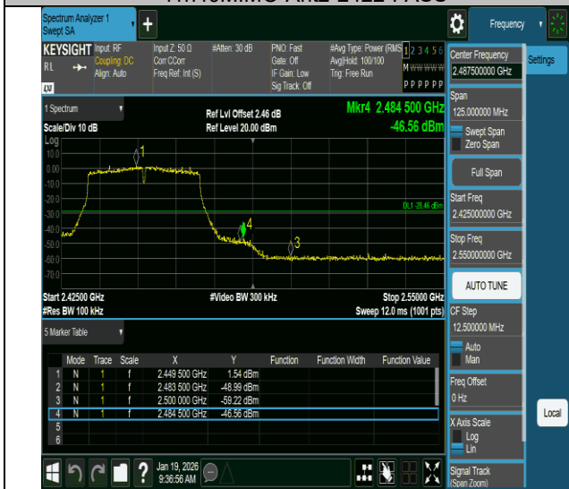
11n40MIMO-Ant2-2452-PASS
