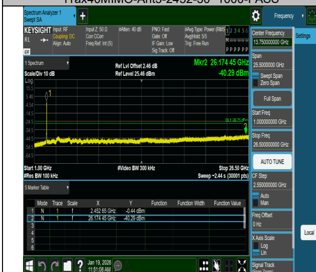
11ax40MIMO-Ant3-2452-1000~26500-PASS
