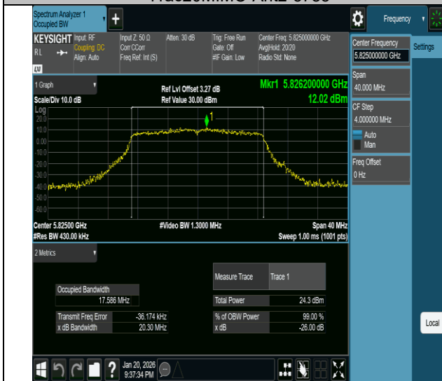
11ac20MIMO-Ant2-5825
