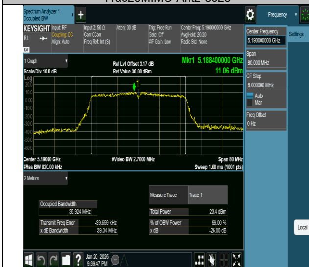
11ac40MIMO-Ant2-5190
