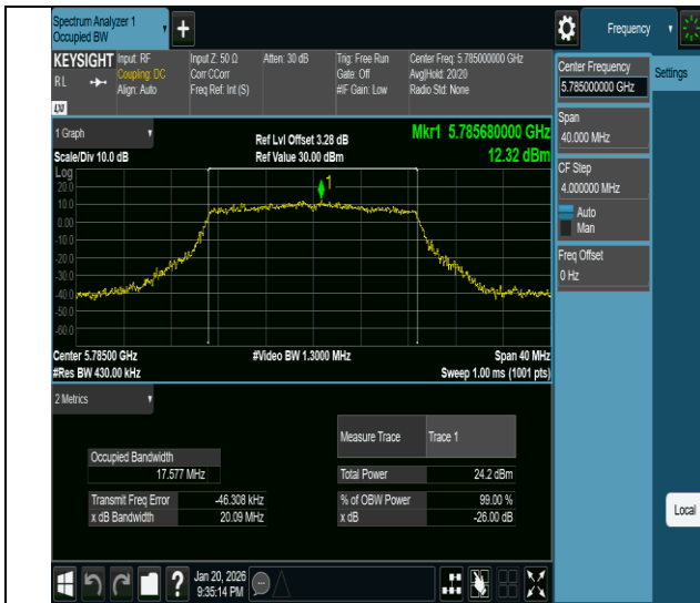
11ac20MIMO-Ant2-5785
