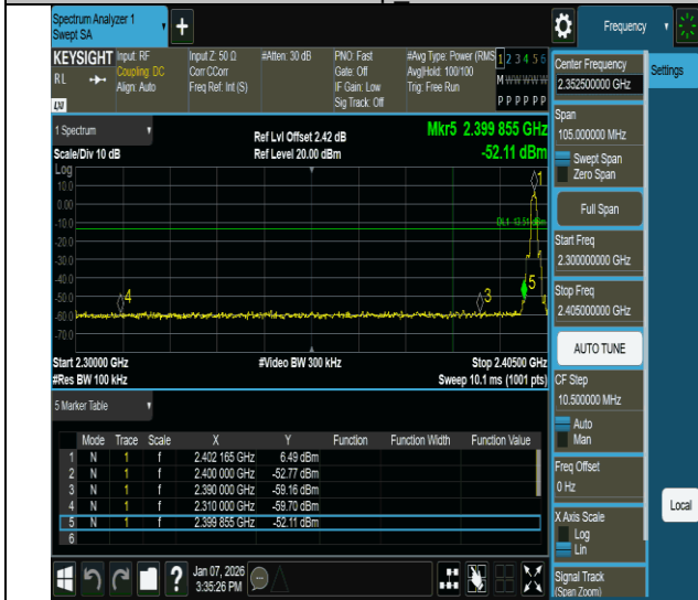
3DH5-Ant2-2402-PASS
