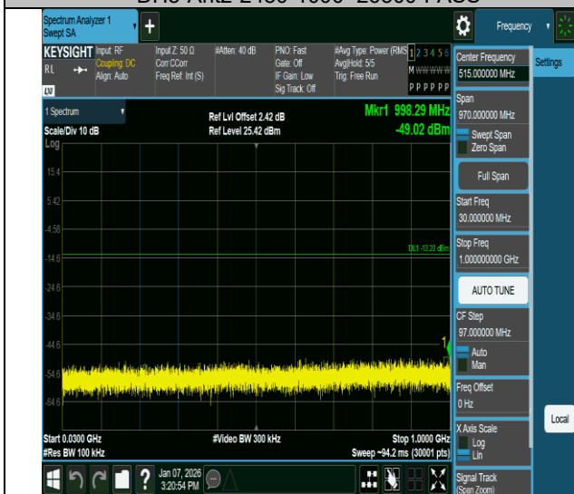
2DH5-Ant2-2402-30~1000-PASS
