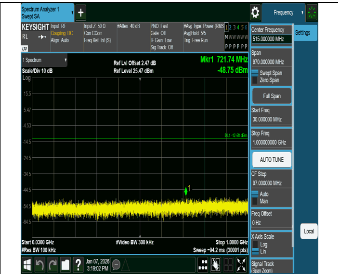
DH5-Ant2-2480-30~1000-PASS
