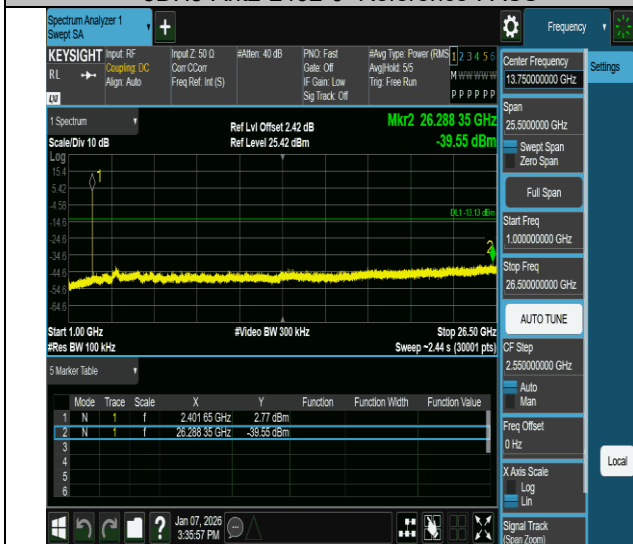
3DH5-Ant2-2402-1000~26500-PASS
