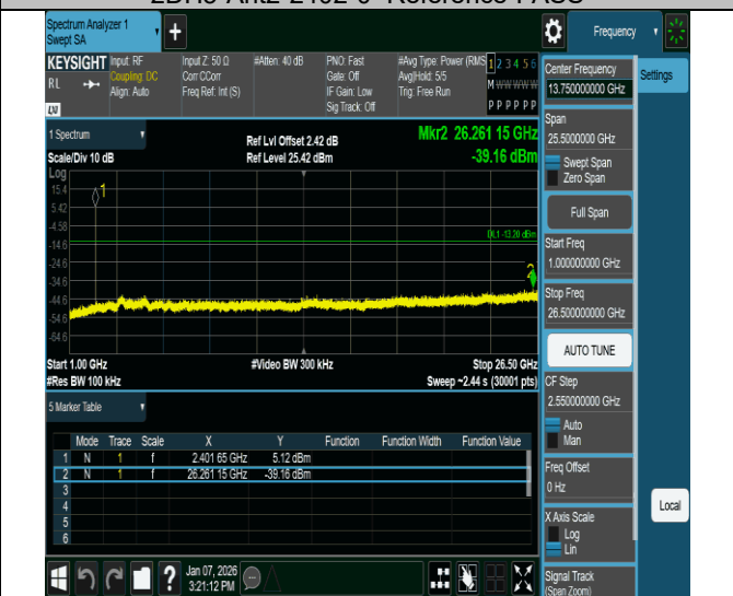
2DH5-Ant2-2402-1000~26500-PASS
