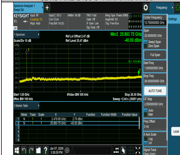
3DH5-Ant2-2480-1000~26500-PASS
