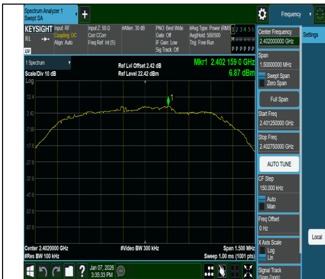
3DH5-Ant2-2402-0~Reference-PASS
