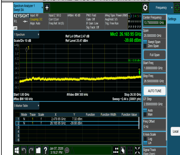
DH5-Ant2-2480-1000~26500-PASS
