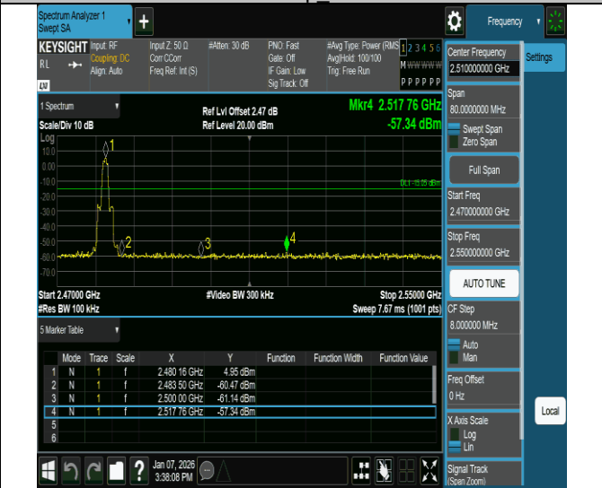
3DH5-Ant2-2480-PASS
