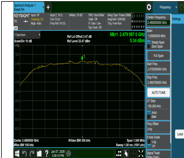
3DH5-Ant2-2480-0~Reference-PASS
