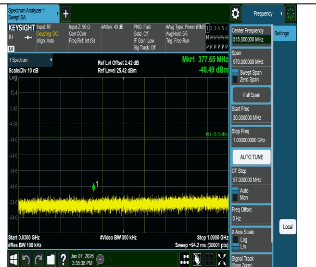
3DH5-Ant2-2402-30~1000-PASS
