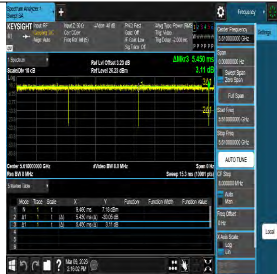
NTNV-11ac80MIMO-Ant3-5610
