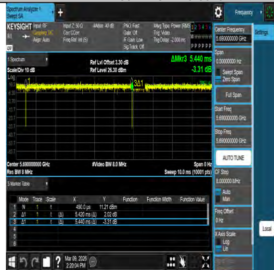
NTNV-11ac80MIMO-Ant3-5690
