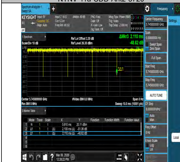
NTNV-11a-CDD-Ant2-5745
