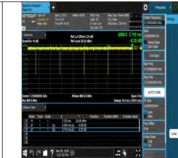
NTNV-11a-CDD-Ant3-5720
