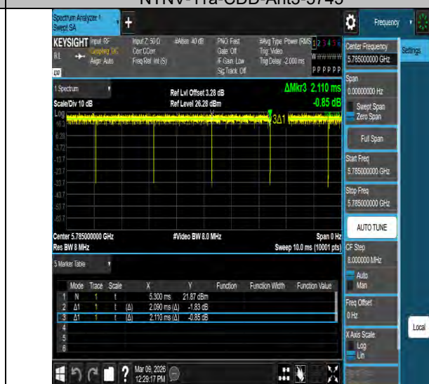
NTNV-11a-CDD-Ant3-5785
