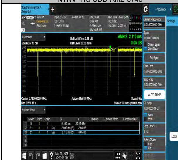
NTNV-11a-CDD-Ant2-5785
