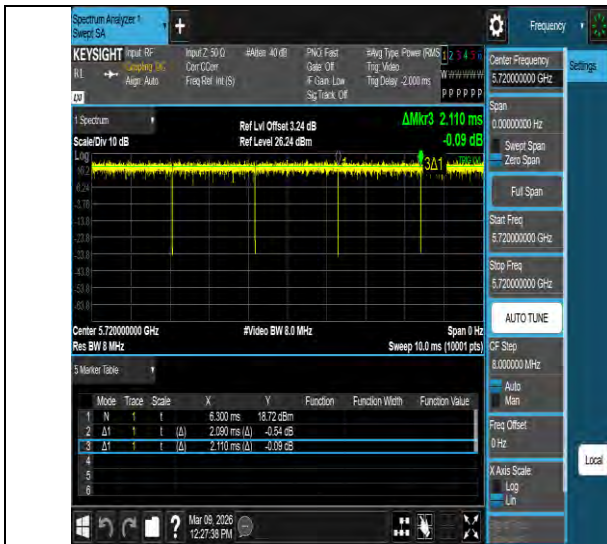
NTNV-11a-CDD-Ant2-5720
