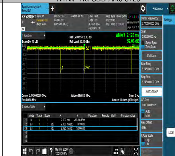
NTNV-11a-CDD-Ant3-5745
