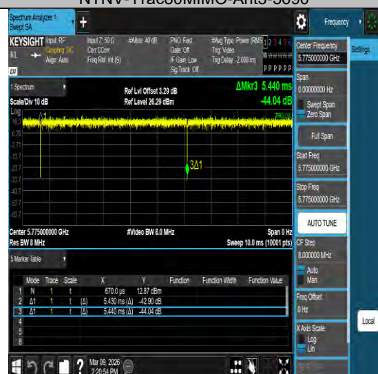
NTNV-11ac80MIMO-Ant3-5775
