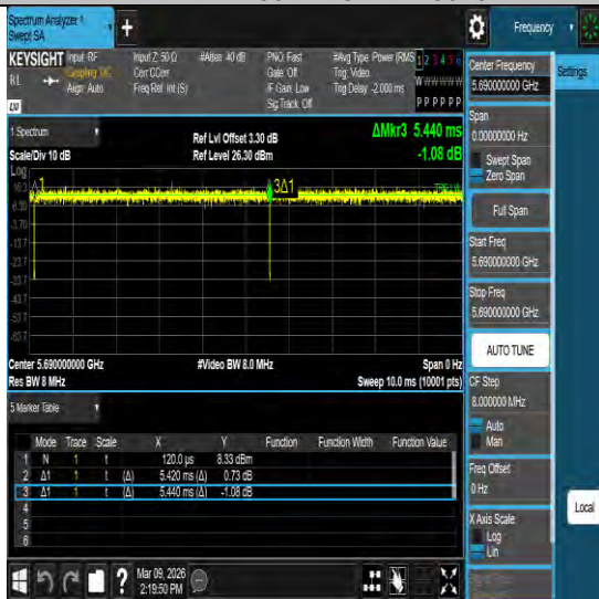
NTNV-11ac80MIMO-Ant2-5690
