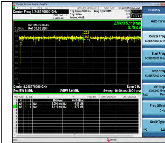
NTNV-11ax20MIMO-Ant2-5240-26Tone-RU8
