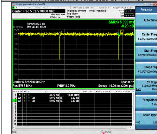
NTVN-11ax20MIMO-Ant2-5320-52Tone-RU40
