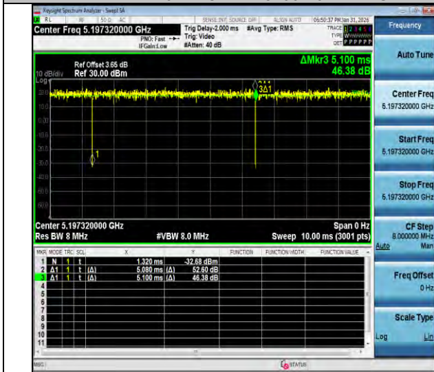
NTNV-11ax20MIMO-Ant2-5200-52Tone-RU39
