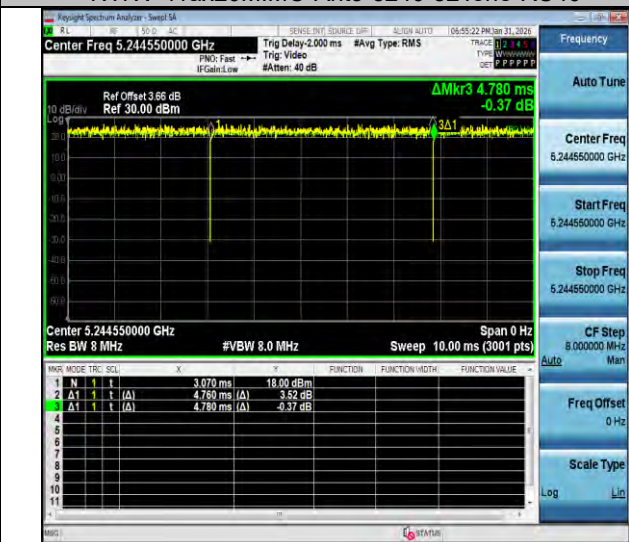
NTNV-11ax20MIMO-Ant3-5240-106Tone-RU54
