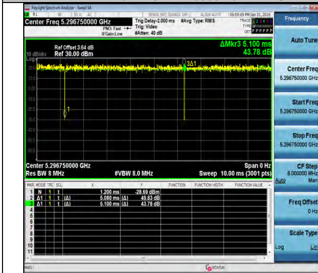
NTNV-11ax20MIMO-Ant2-5300-52Tone-RU39
