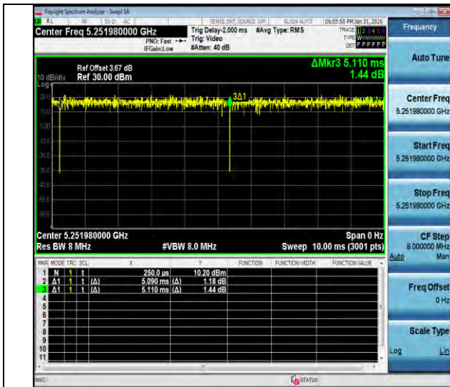
NTNV-11ax20MIMO-Ant2-5260-26Tone-RU0
