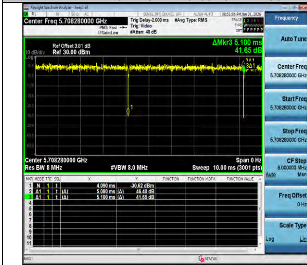
NTNV-11ax20MIMO-Ant2-5700-52Tone-RU40
