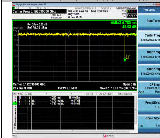
NTNV-11ax20MIMO-Ant2-5200-106Tone-RU53
