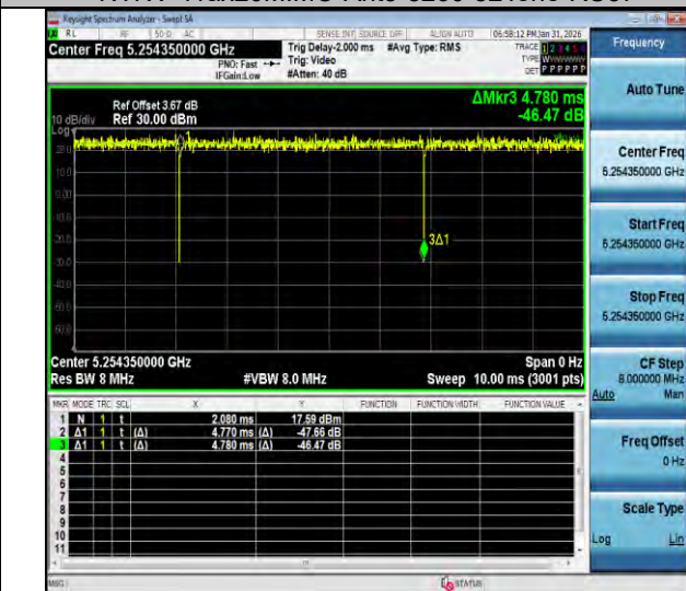
NTNV-11ax20MIMO-Ant3-5260-106Tone-RU53
