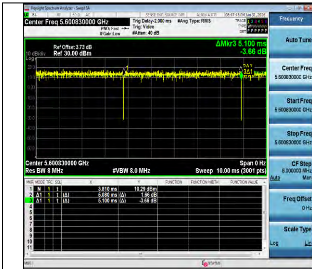
NTNV-11ax20MIMO-Ant2-5600-26Tone-RU4
