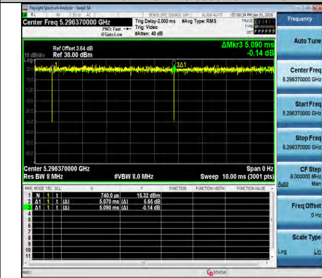
NTNV-11ax20MIMO-Ant3-5300-52Tone-RU39
