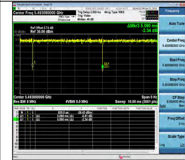
NTNV-11ax20MIMO-Ant3-5500-52Tone-RU37
