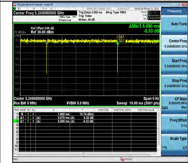
NTNV-11ax20MIMO-Ant3-5240-52Tone-RU40
