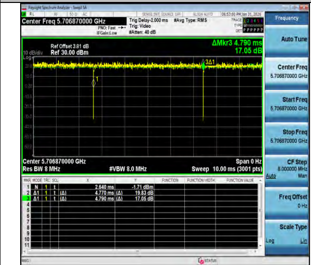
NTNV-11ax20MIMO-Ant3-5700-106Tone-RU54
