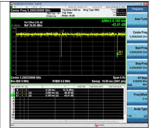
NTNV-11ax20MIMO-Ant3-5200-26Tone-RU4
