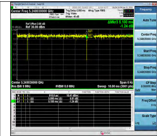
NTNV-11ax20MIMO-Ant3-5240-26Tone-RU8
