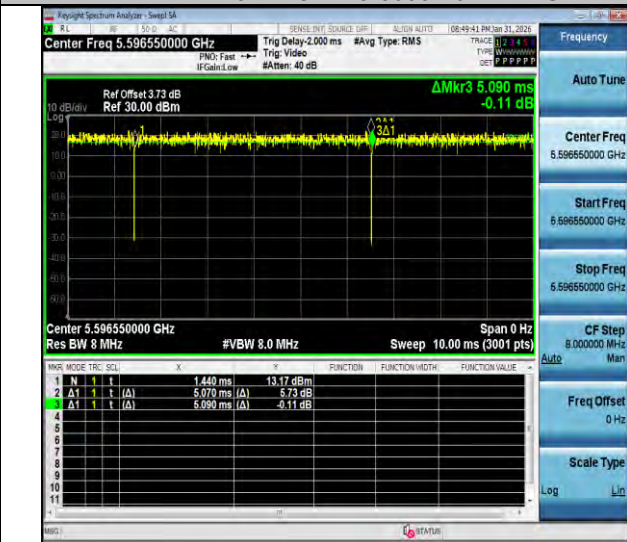
NTNV-11ax20MIMO-Ant3-5600-52Tone-RU39
