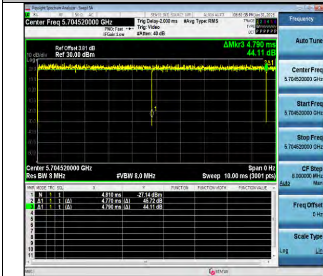
NTNV-11ax20MIMO-Ant2-5700-106Tone-RU54
