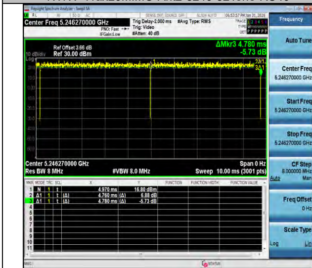
NTNV-11ax20MIMO-Ant2-5240-106Tone-RU54
