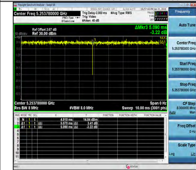
NTNV-11ax20MIMO-Ant3-5260-52Tone-RU37
