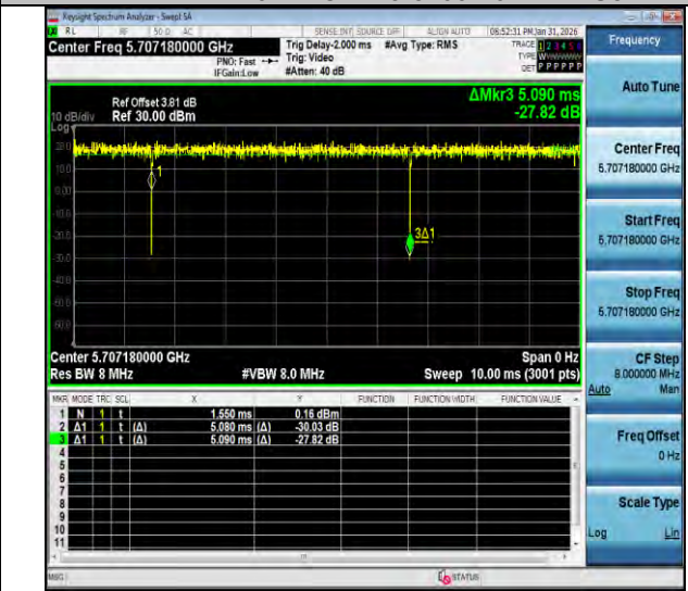
NTNV-11ax20MIMO-Ant3-5700-52Tone-RU40
