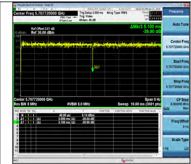
NTNV-11ax20MIMO-Ant3-5700-26Tone-RU8
