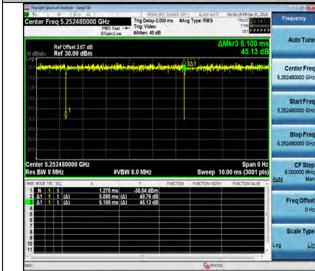
NTNV-11ax20MIMO-Ant2-5260-52Tone-RU37
