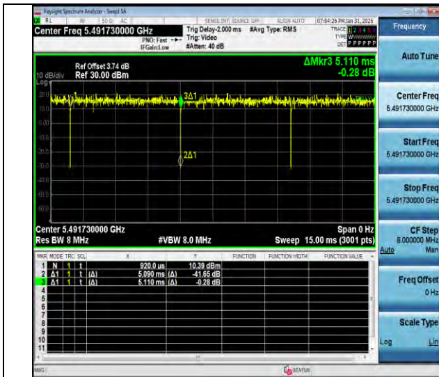
NTNV-11ax20MIMO-Ant2-5500-26Tone-RU0
