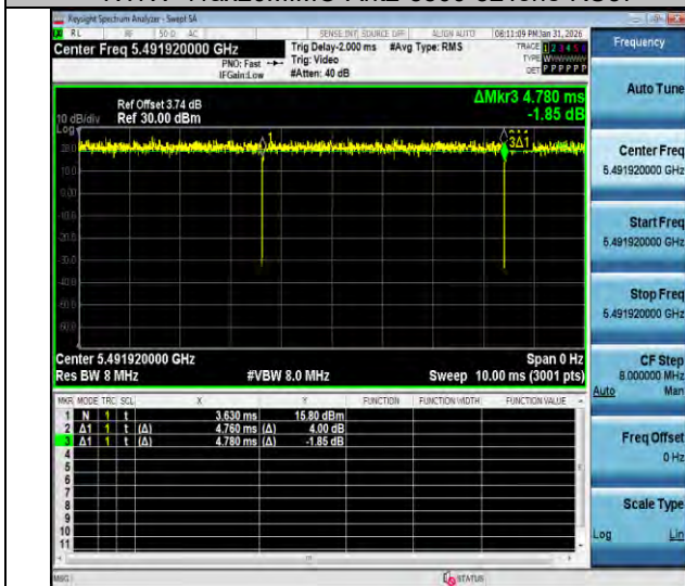
NTNV-11ax20MIMO-Ant2-5500-106Tone-RU53
