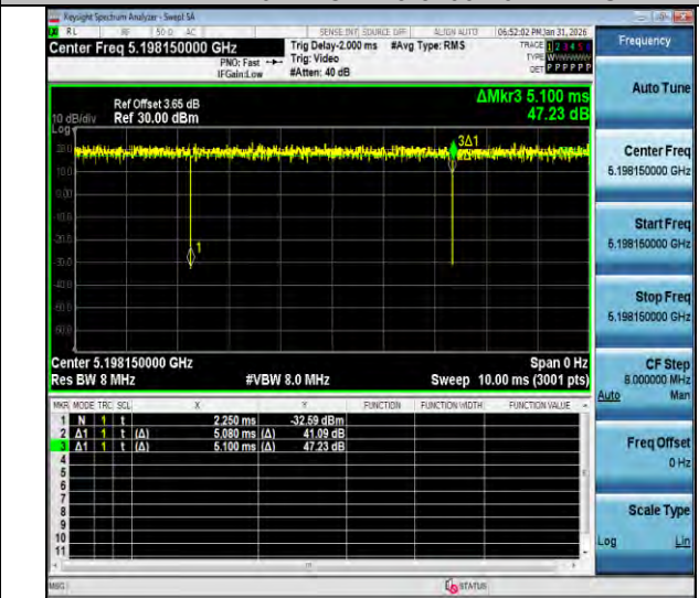
NTNV-11ax20MIMO-Ant3-5200-52Tone-RU39
