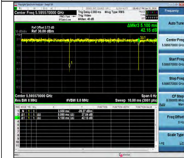
NTNV-11ax20MIMO-Ant2-5600-52Tone-RU39
