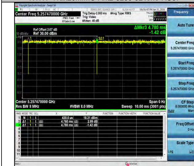
NTNV-11ax20MIMO-Ant2-5260-106Tone-RU53
