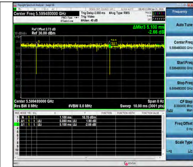
NTNV-11ax20MIMO-Ant3-5600-26Tone-RU4
