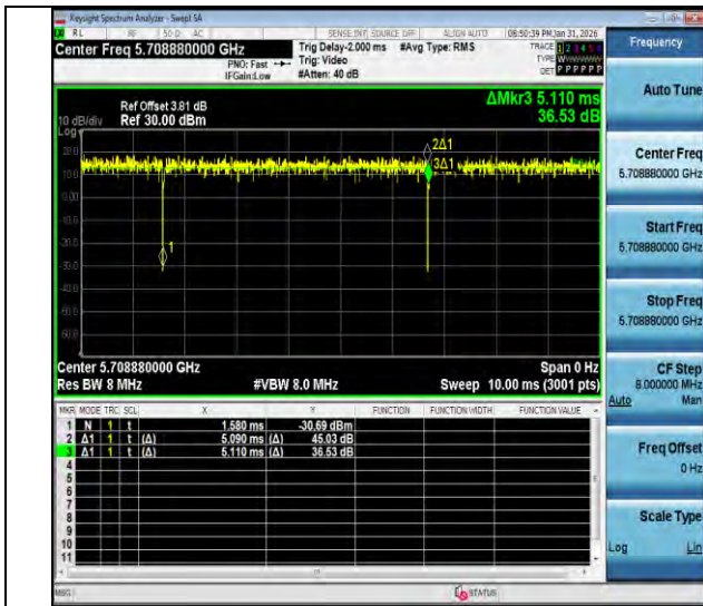
NTNV-11ax20MIMO-Ant2-5700-26Tone-RU8
