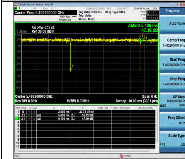
NTNV-11ax20MIMO-Ant2-5500-52Tone-RU37
