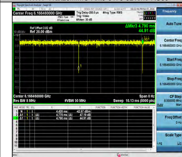
NTNV-11ax20MIMO-Ant3-6175-106Tone-RU53
