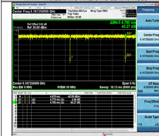
NTNV-11ax20MIMO-Ant2-6175-106Tone-RU53
