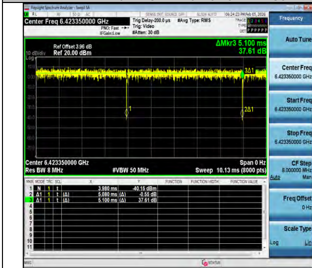
NTVN-11ax20MIMO-Ant2-6415-52Tone-RU40
