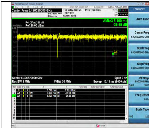
NTVN-11ax20MIMO-Ant2-6435-26Tone-RU0
