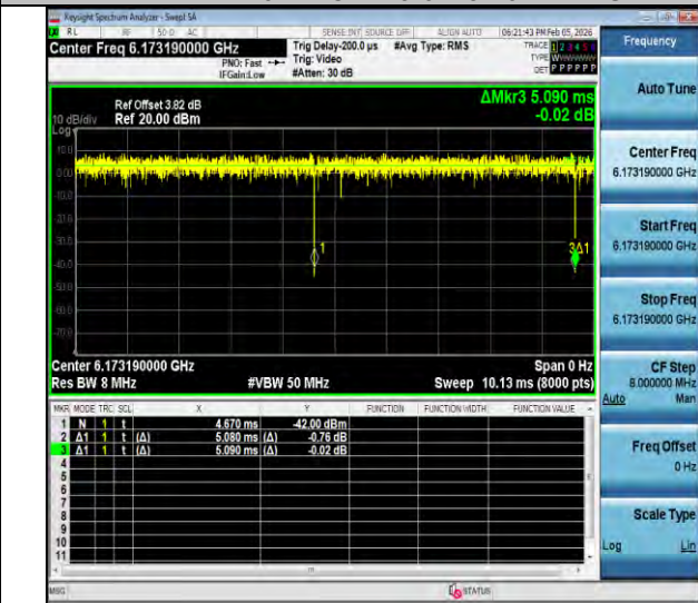
NTNV-11ax20MIMO-Ant3-6175-52Tone-RU39
