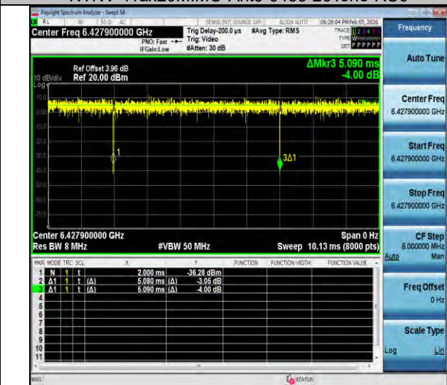
NTVN-11ax20MIMO-Ant3-6435-52Tone-RU37
