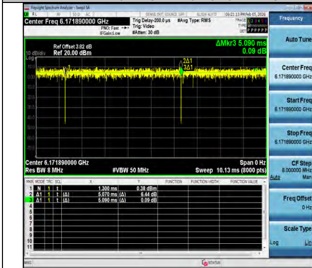
NTNV-11ax20MIMO-Ant2-6175-52Tone-RU39
