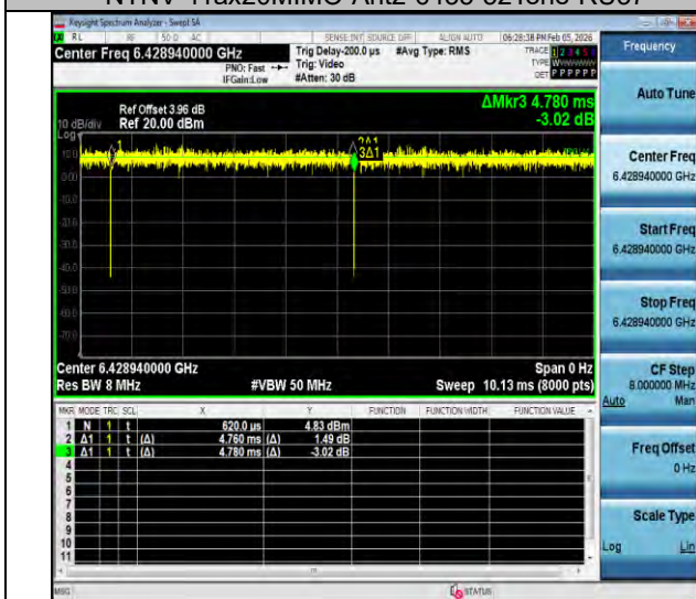
NTVN-11ax20MIMO-Ant2-6435-106Tone-RU53
