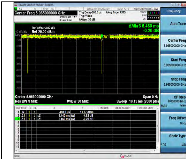
NTNV-11ax40MIMO-Ant2-5965
