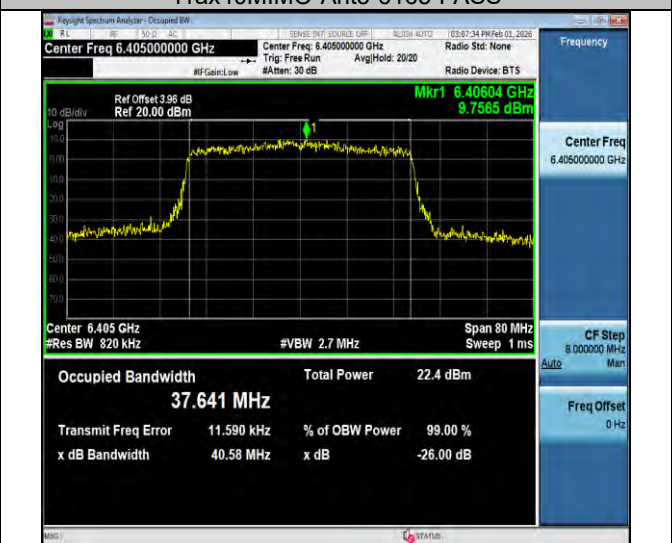
11ax40MIMO-Ant3-6405-PASS
