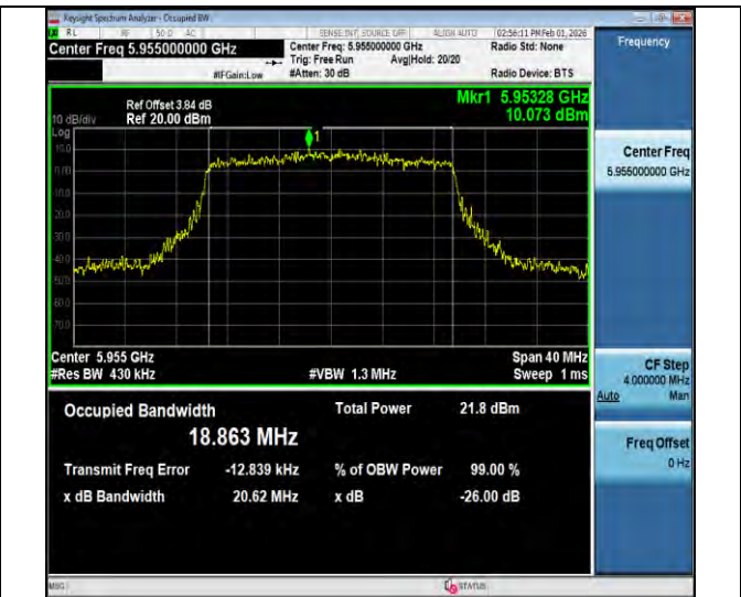
11ax20MIMO-Ant3-5955-PASS
