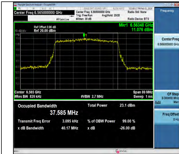
11ax40MIMO-Ant2-6565-PASS
