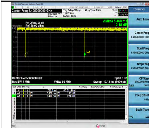
NTNV-11ax40MIMO-Ant2-6405
