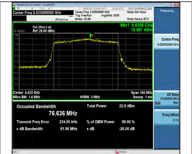
11ax80MIMO-Ant3-6625-PASS
