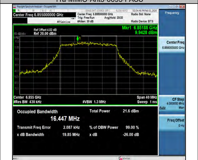
11a-MIMO-Ant3-6855-PASS
