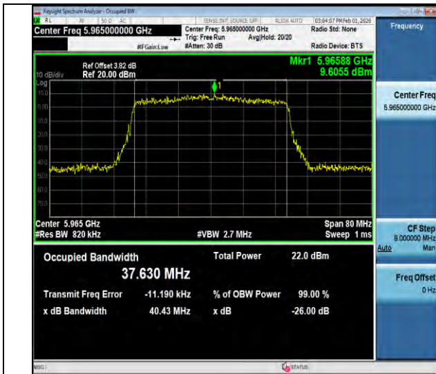
11ax40MIMO-Ant2-5965-PASS
