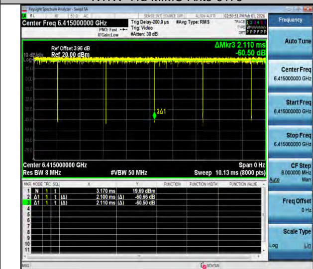
NTNV-11a-MIMO-Ant3-6415
