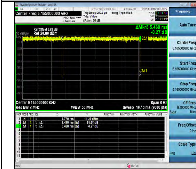
NTNV-11ax40MIMO-Ant2-6165
