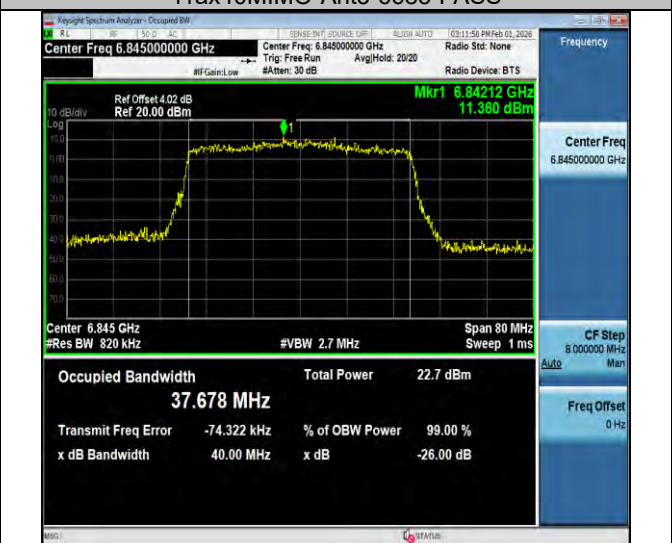
11ax40MIMO-Ant3-6845-PASS
