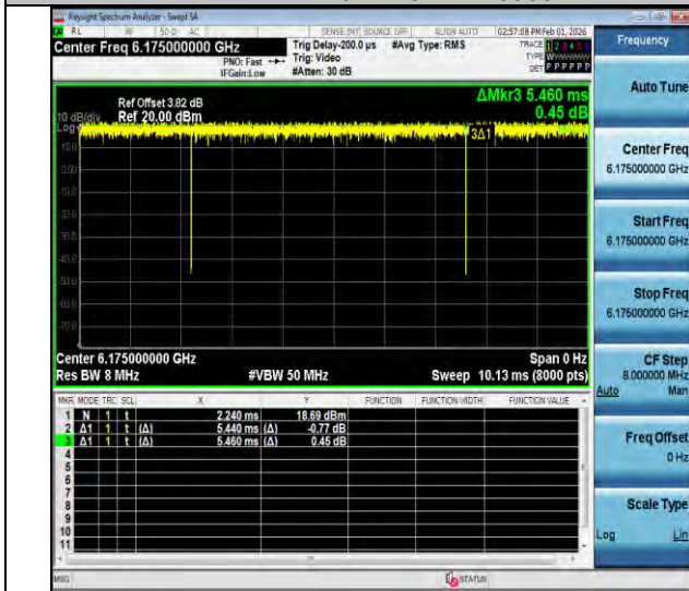
NTNV-11ax20MIMO-Ant2-6175
