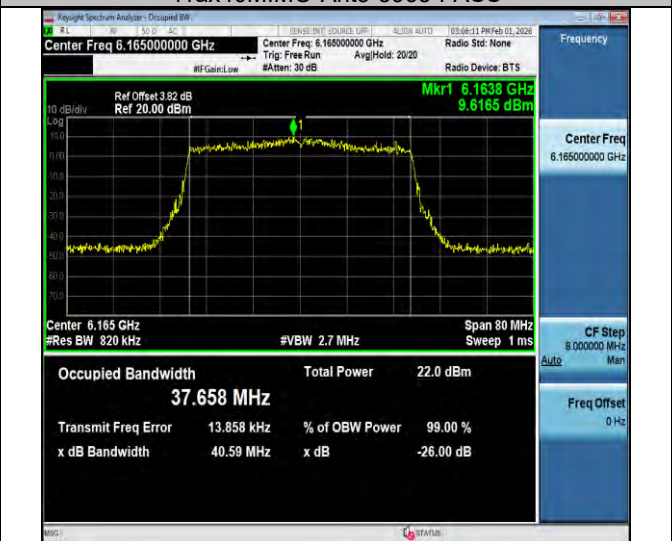
11ax40MIMO-Ant3-6165-PASS
