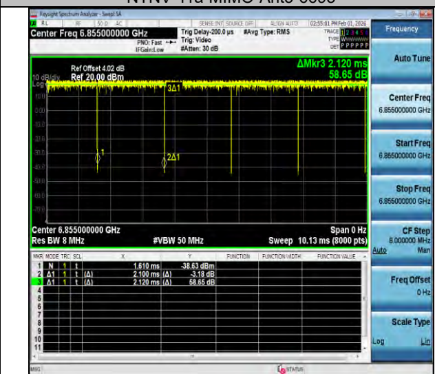
NTNV-11a-MIMO-Ant3-6855
