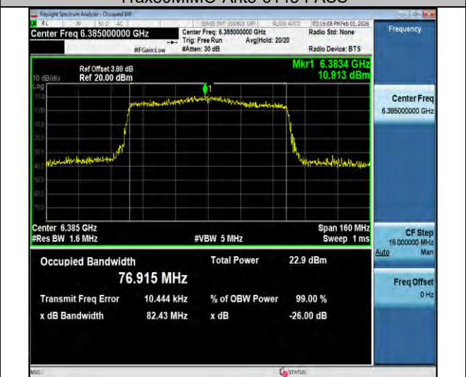
11ax80MIMO-Ant3-6385-PASS
