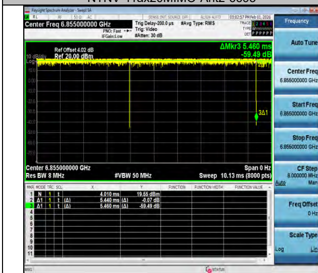
NTNV-11ax20MIMO-Ant2-6855
