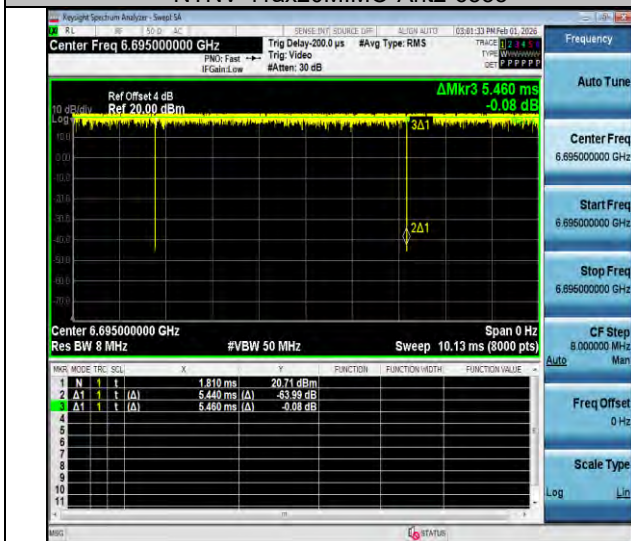
NTNV-11ax20MIMO-Ant2-6695
