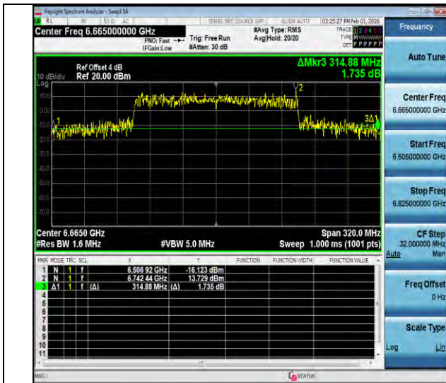
11ax160MIMO-Ant2-6665
