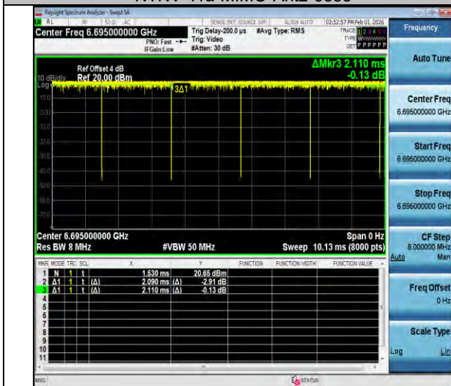
NTNV-11a-MIMO-Ant2-6695
