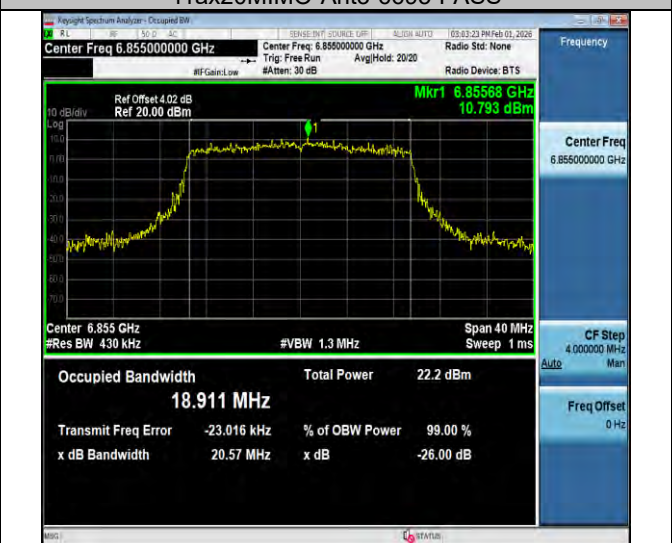
11ax20MIMO-Ant3-6855-PASS
