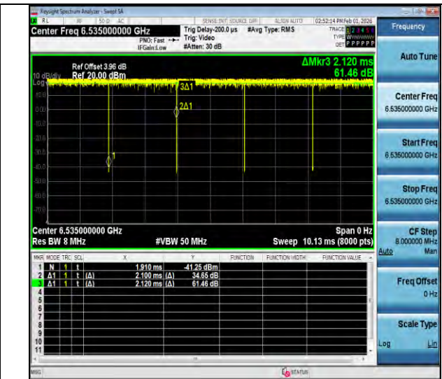
NTNV-11a-MIMO-Ant3-6535
