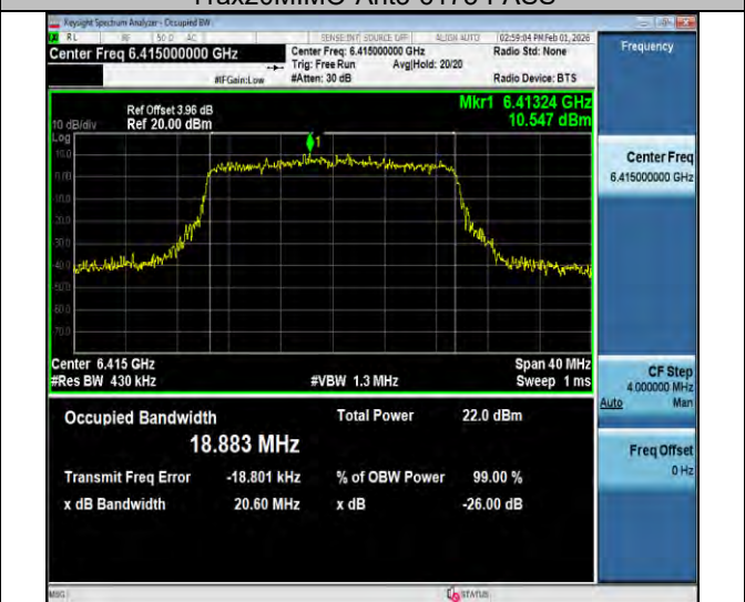
11ax20MIMO-Ant3-6415-PASS
