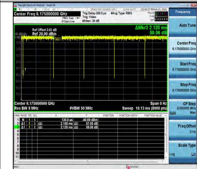
NTNV-11a-MIMO-Ant3-6175
