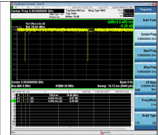
NTNV-11ax20MIMO-Ant3-5955
