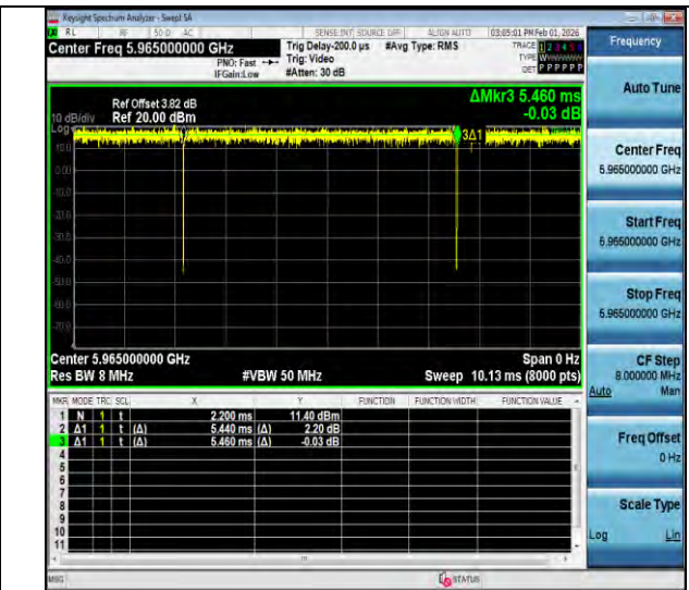
NTNV-11ax40MIMO-Ant3-5965
