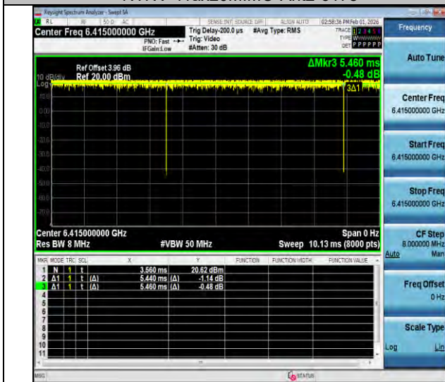
NTNV-11ax20MIMO-Ant2-6415
