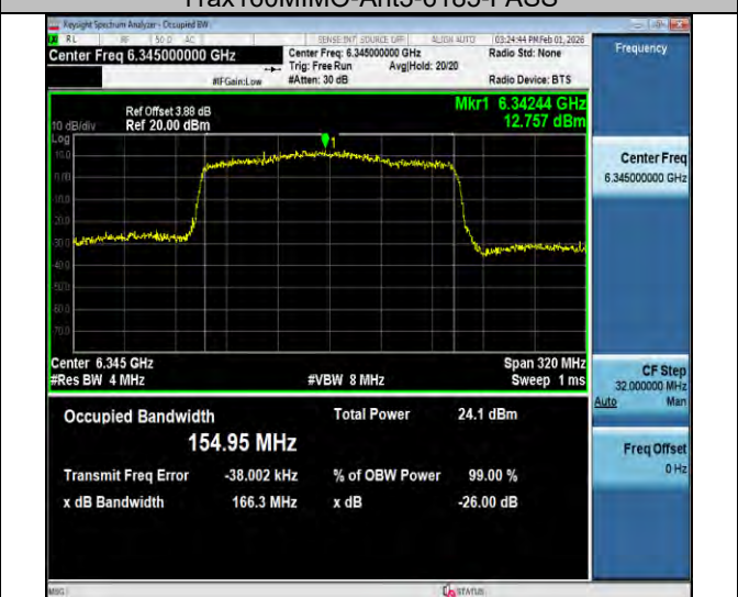
11ax160MIMO-Ant3-6345-PASS
