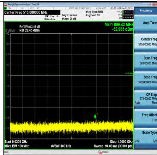
2DH5-Ant2-2441-30~1000-PASS
