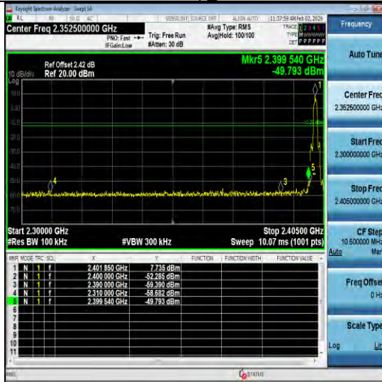
3DH5-Ant2-2402-PASS
