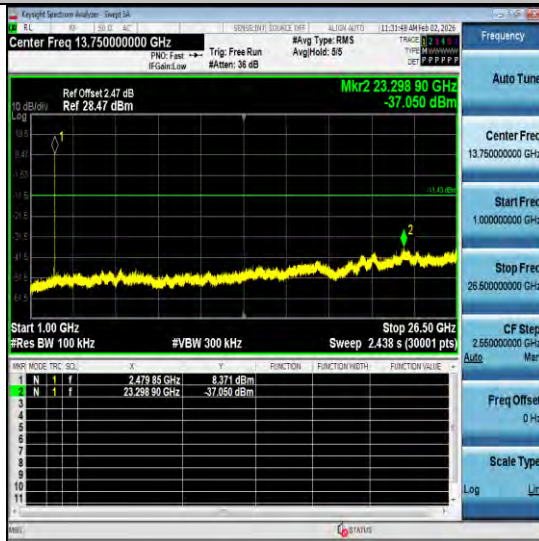
DH5-Ant2-2480-1000~26500-PASS
