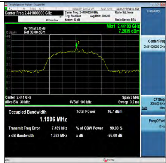
3DH5-Ant2-2441
