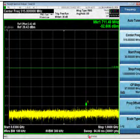
3DH5-Ant2-2402-30~1000-PASS
