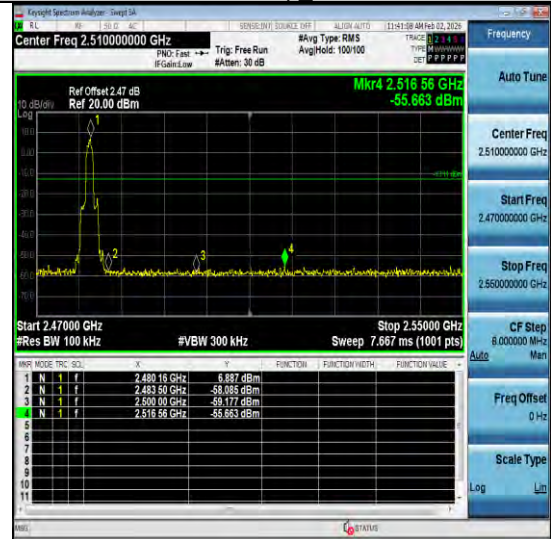
3DH5-Ant2-2480-PASS
