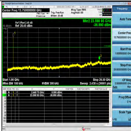
2DH5-Ant2-2441-1000~26500-PASS
