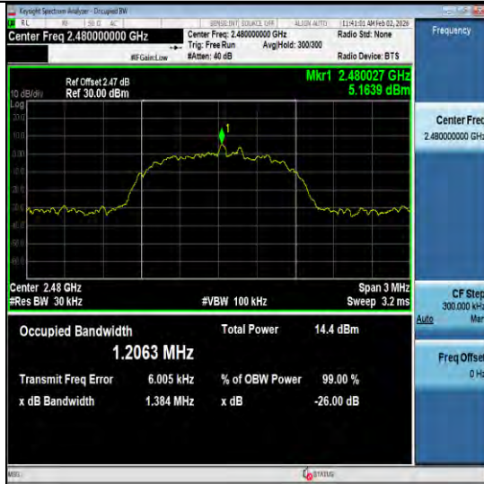
3DH5-Ant2-2480
