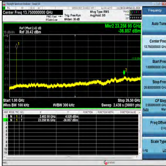
3DH5-Ant2-2402-1000~26500-PASS
