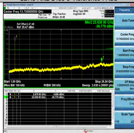
2DH5-Ant2-2480-1000~26500-PASS
