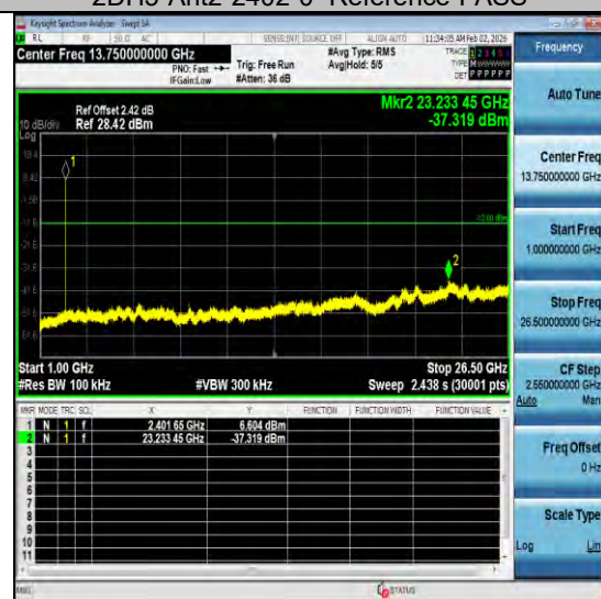
2DH5-Ant2-2402-1000~26500-PASS
