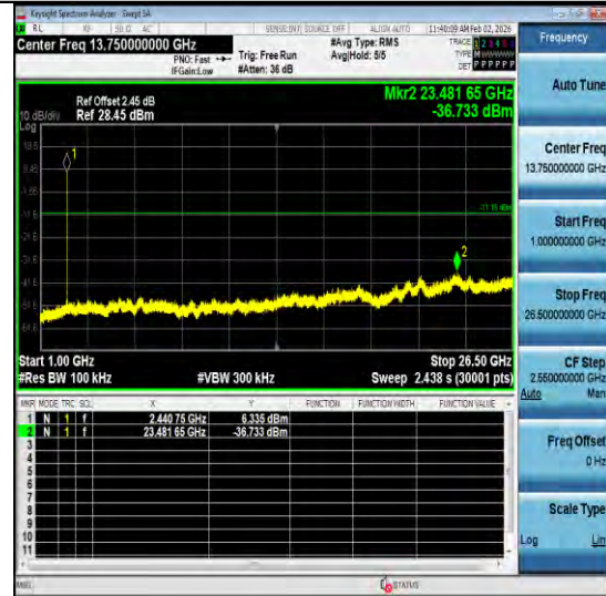
3DH5-Ant2-2441-1000~26500-PASS
