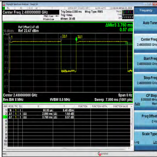
NTNV-3DH5-Ant2-2480
