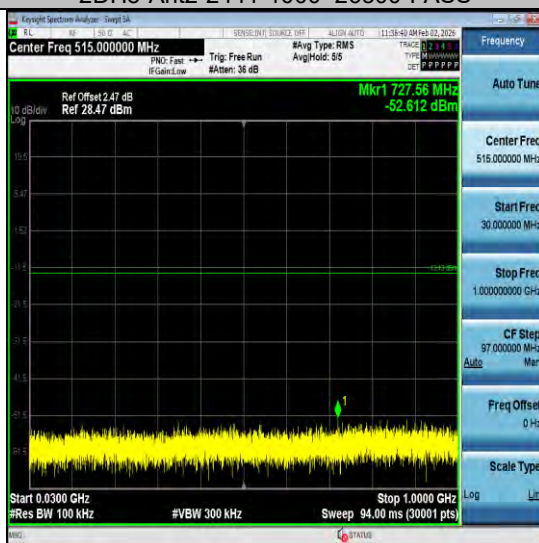
2DH5-Ant2-2480-30~1000-PASS
