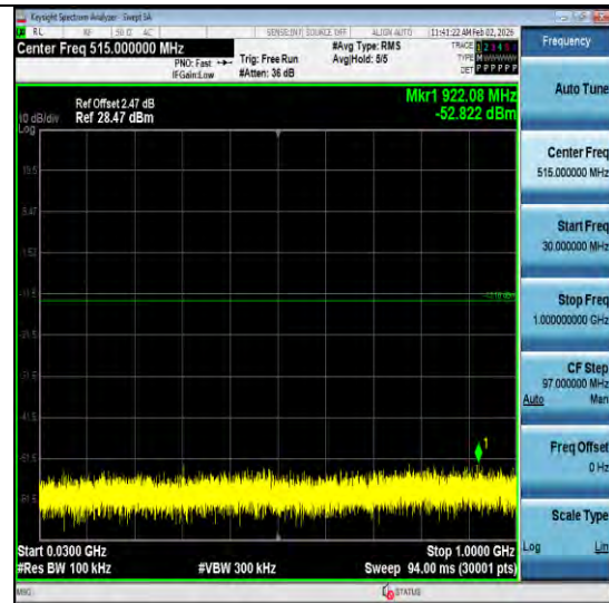
3DH5-Ant2-2480-30~1000-PASS
