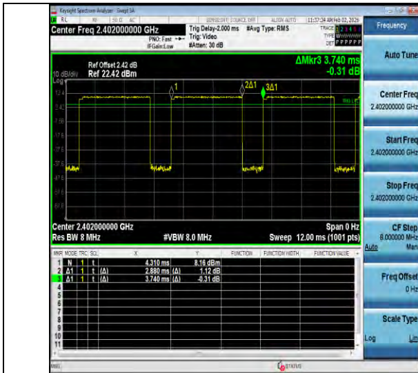
NTNV-3DH5-Ant2-2402
