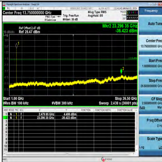
3DH5-Ant2-2480-1000~26500-PASS
