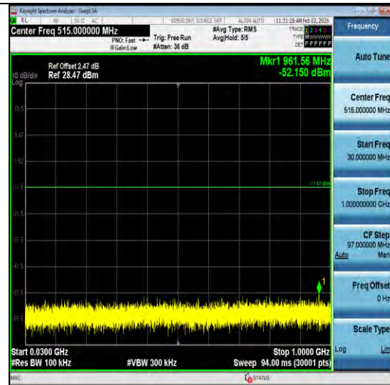
DH5-Ant2-2480-30~1000-PASS
