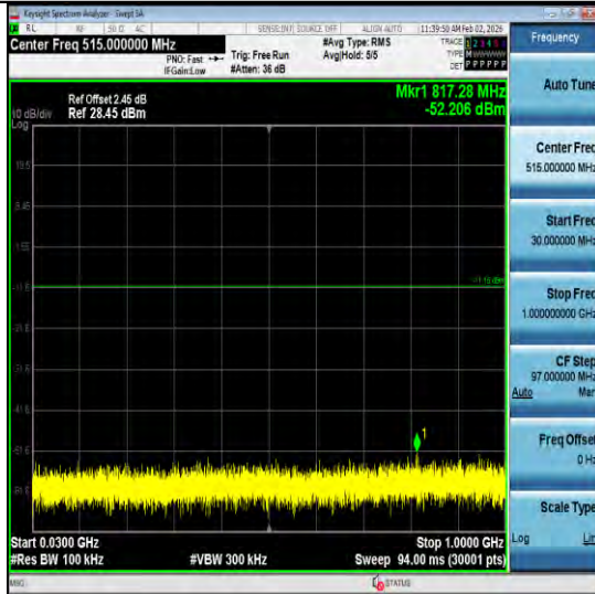
3DH5-Ant2-2441-30~1000-PASS
