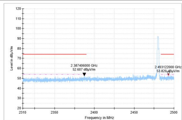
BANDEDGE-S8-CH39-PK
