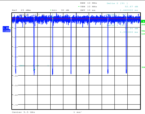
NTNV-11A-Ant1-5500
