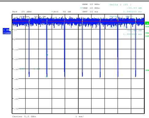
NTNV-11N20SISO-Ant1-5200
