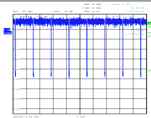
NTNV-11N20SISO-Ant1-5180
