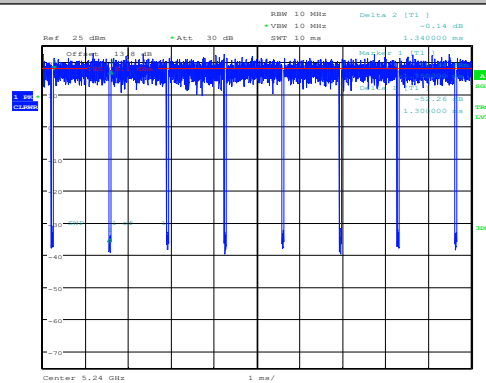
NTNV-11N20SISO-Ant1-5240
