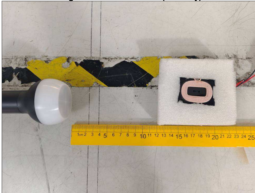
Magnetic & Electric Field (EUT+EPP15W+7mm)
