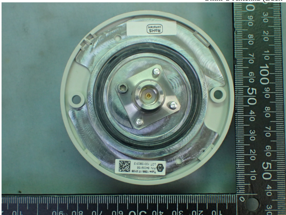
Figure 8 Omni-S Antenna (Back View)
