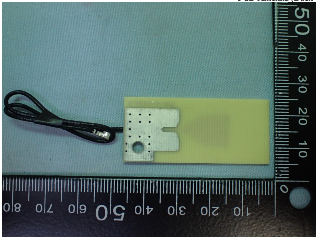
Figure 4 PCB Antenna (Back View)
