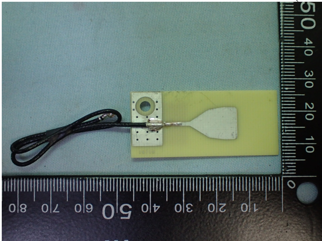
Figure 3 PCB Antenna (Front View)
