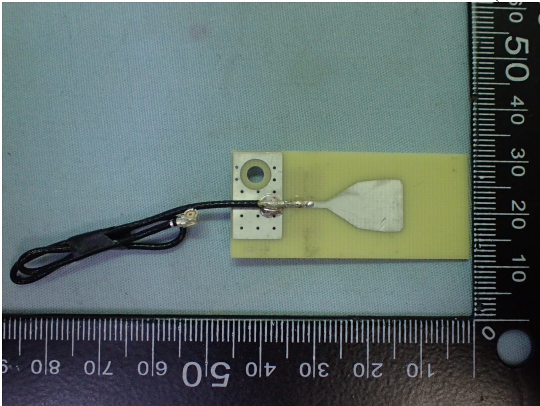
Figure 5 PCB Antenna (Front View)
