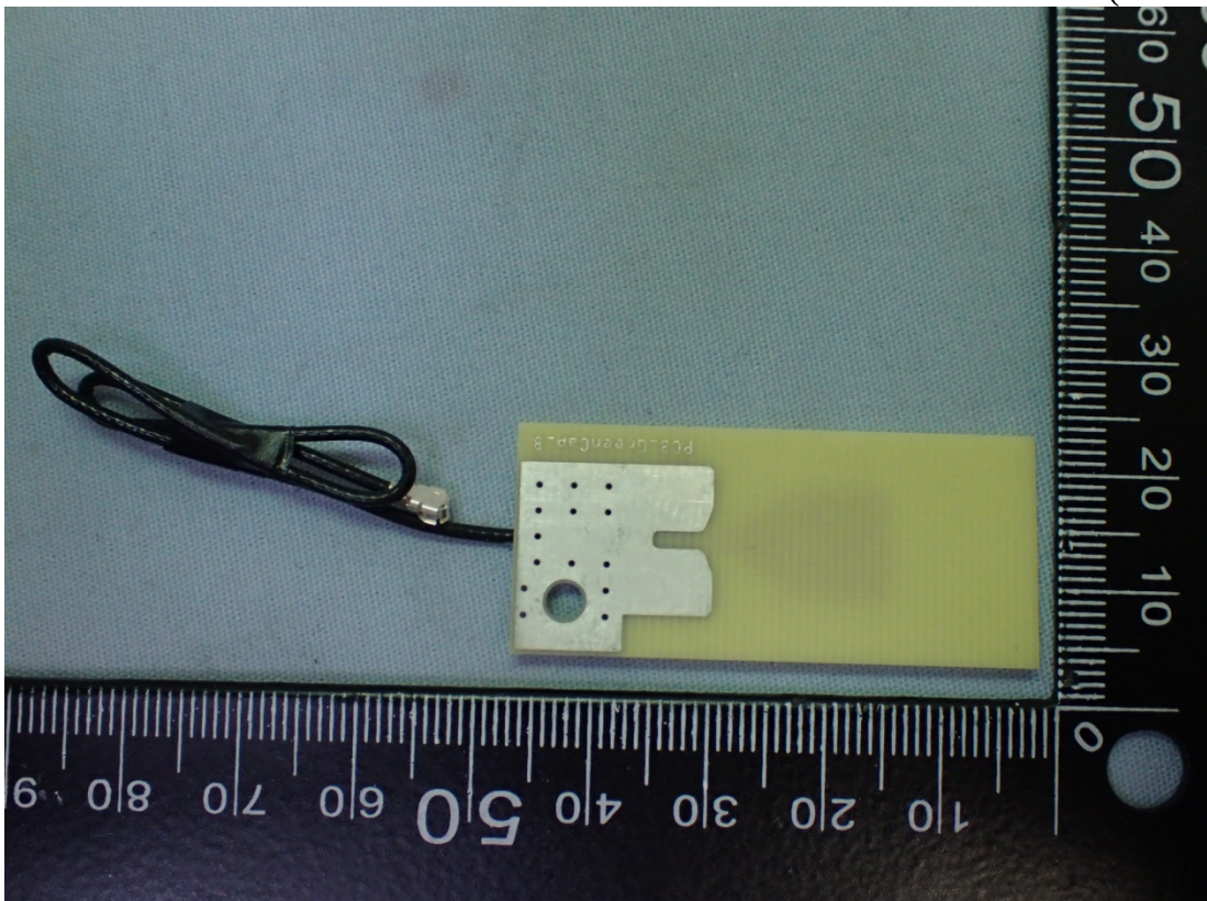
Figure 6 PCB Antenna (Back View)
