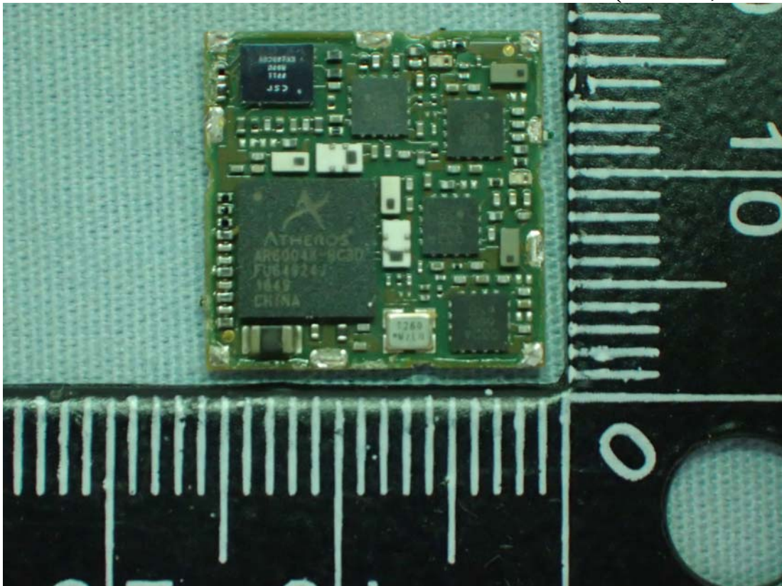
Figure 11 Internal View (RF Board, Front View)
