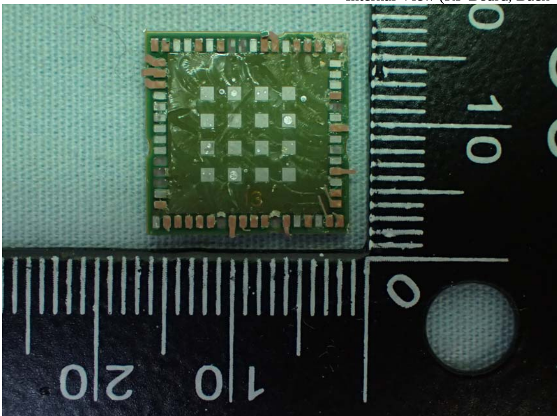
Figure 12 Internal View (RF Board, Back View)
