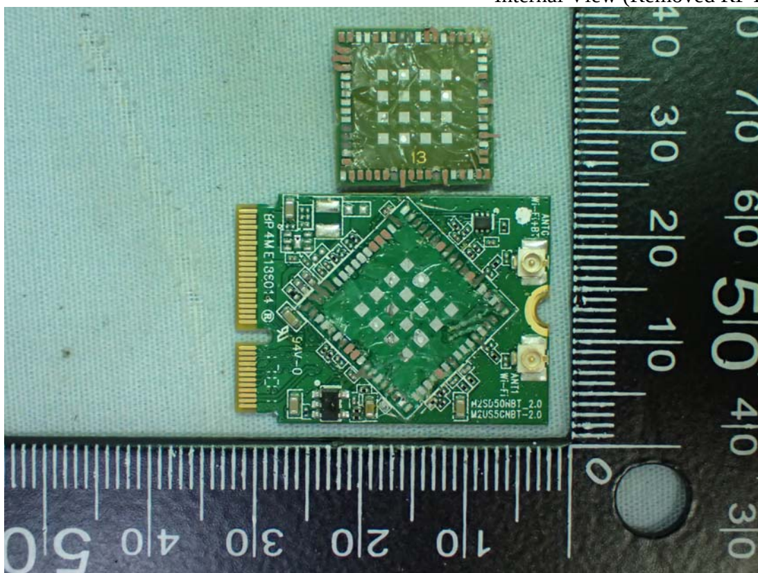
Internal View (Removed RF Board)
