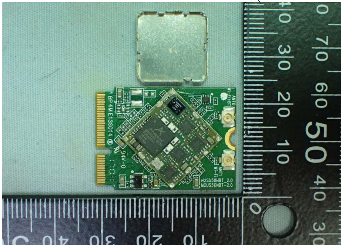
Internal View (Removed Shielded Cover)
